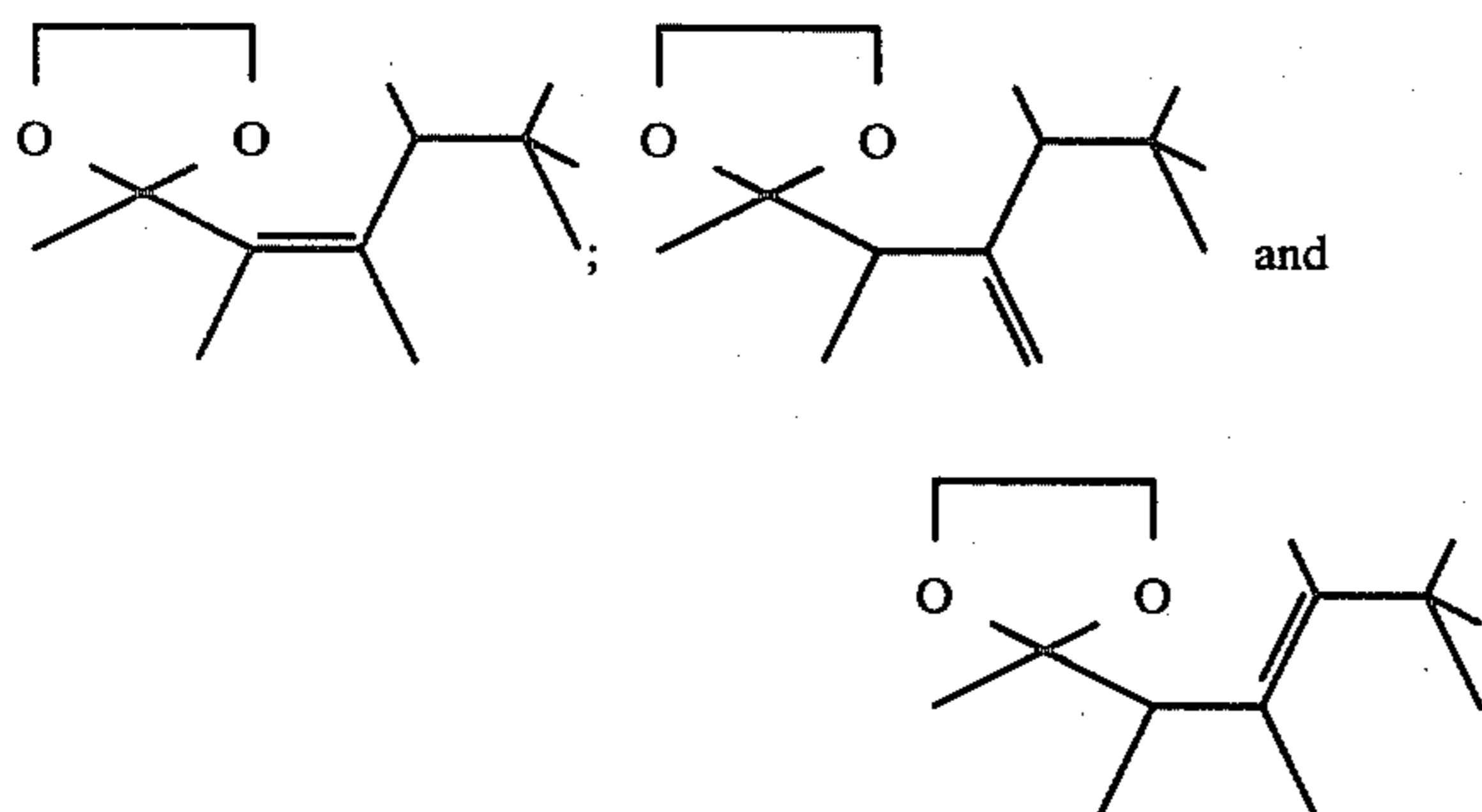
FIG. 18 is the GLC profile for the reaction product of Example X.
