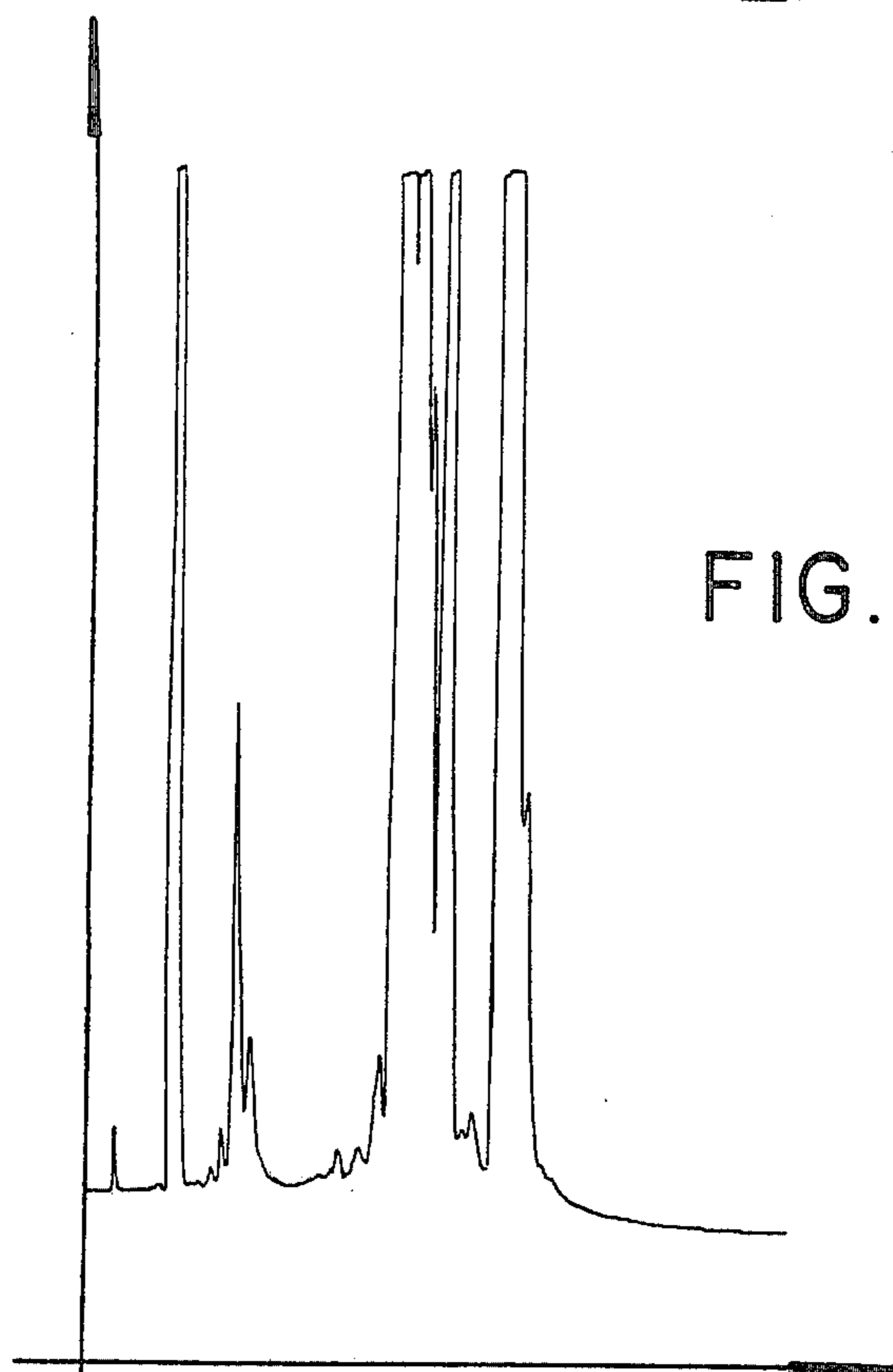
FIG.16 NMR SPECTRUM FOR EXAMPLE IX.
