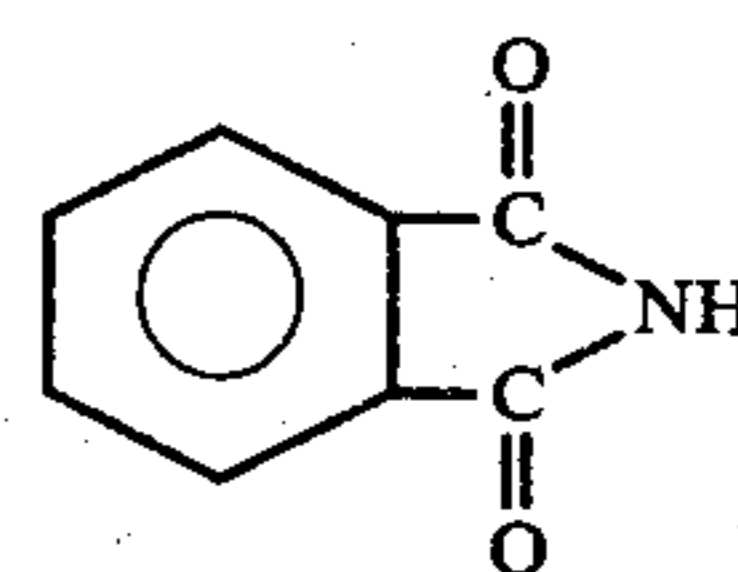
Phthalimide
