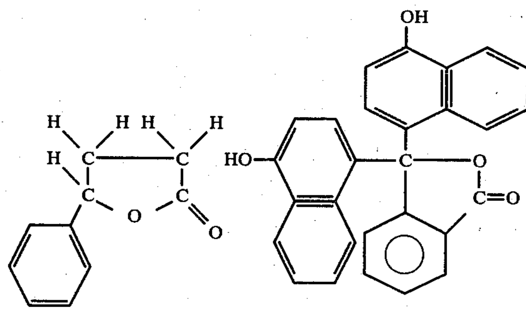
\gamma -Phenyl- \gamma -butyrolactone
