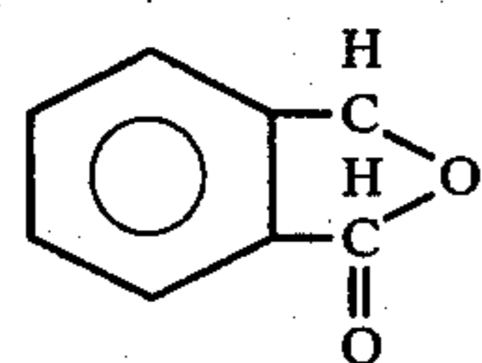
Phthalide
