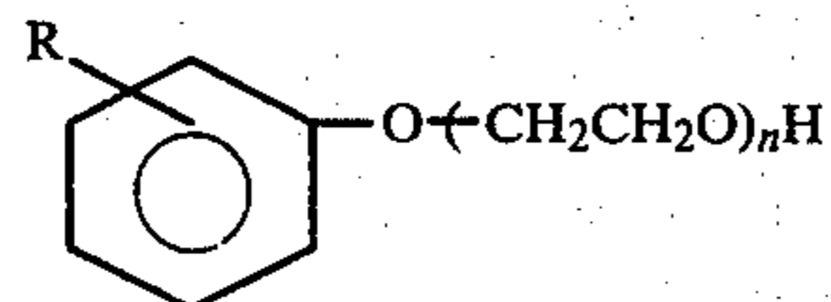
Polyethoxyalkylphenol
