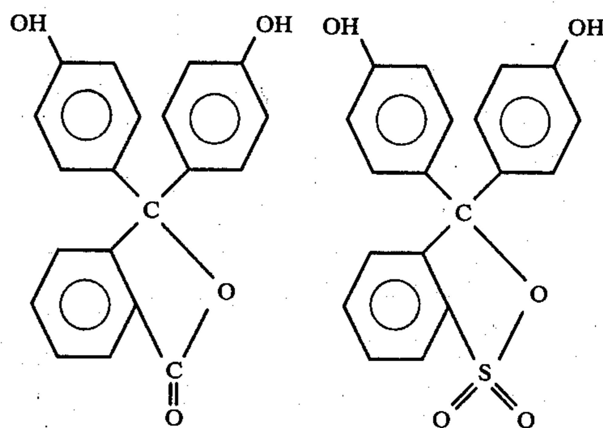
Phenolphthalein
