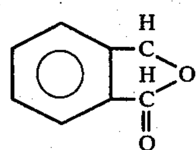
Phthalide
