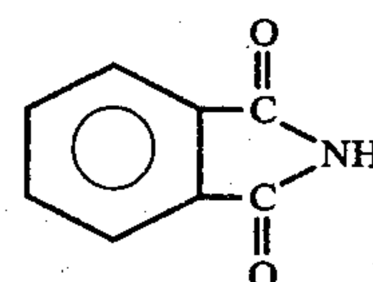
Phthalimide
