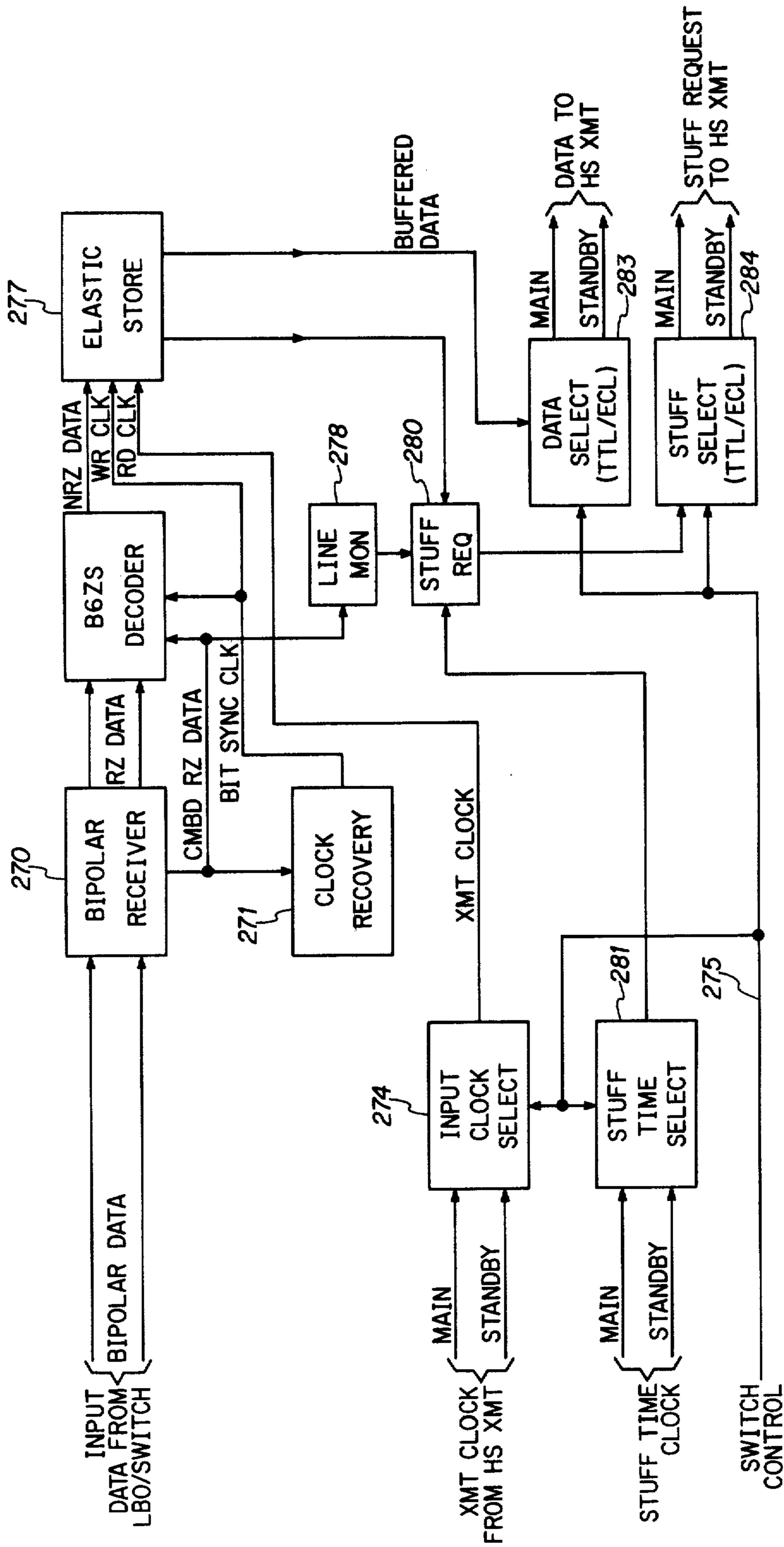
FIG. 8 INTERMEDIATE SPEED XMT INTERFACE (IS XMT INTFC)
