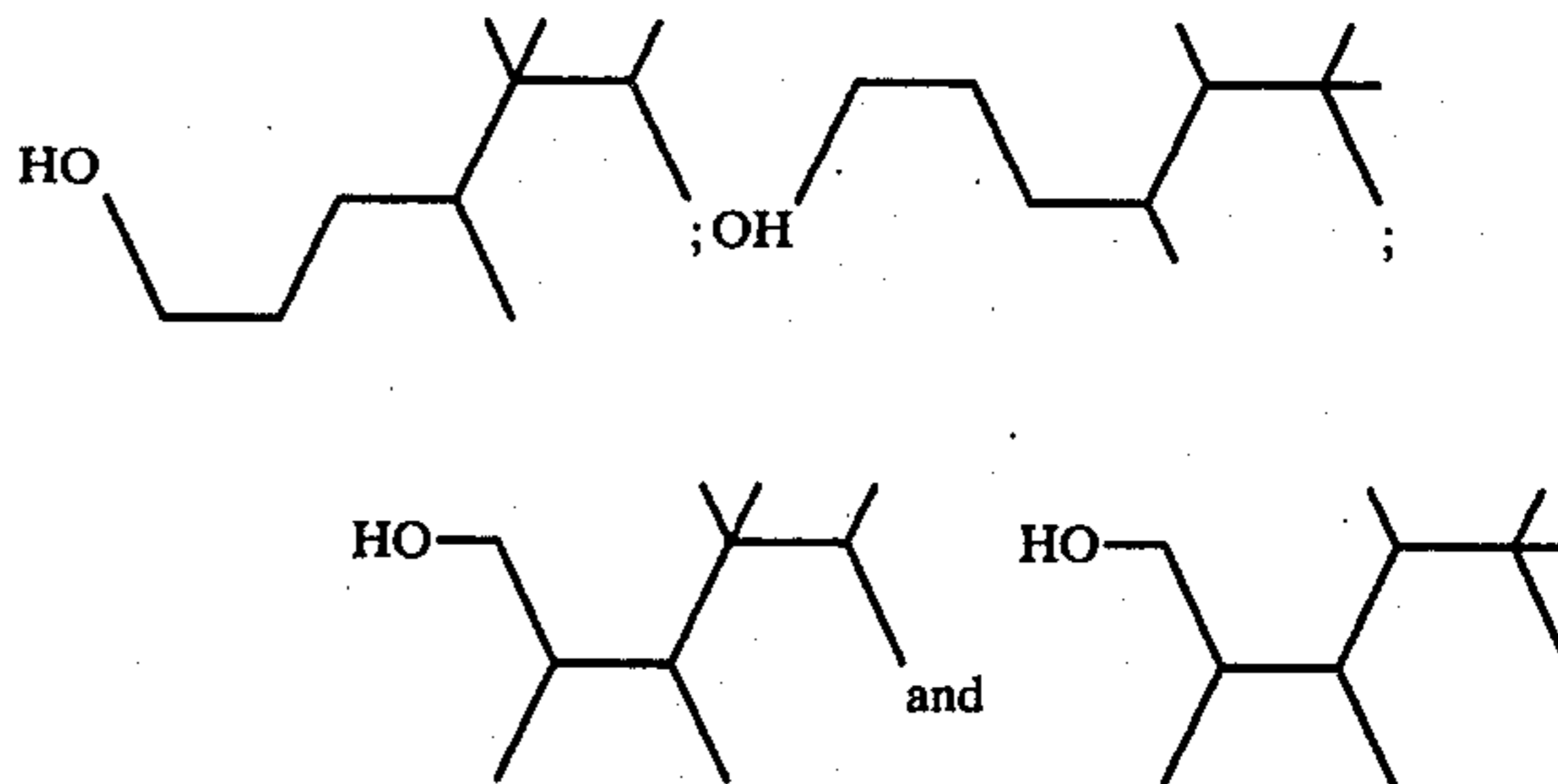
FIG. 10 is the NMR spectrum for the diisoundecanol compounds produced according to Example II having the structures:
