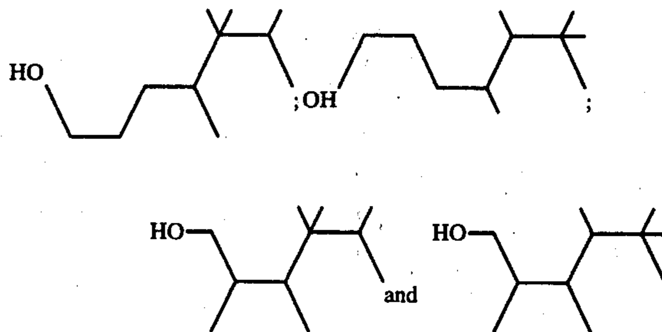
FIG. 8 is the infra-red spectrum for the diisoundecanal compounds produced according to Example II having the structures:
