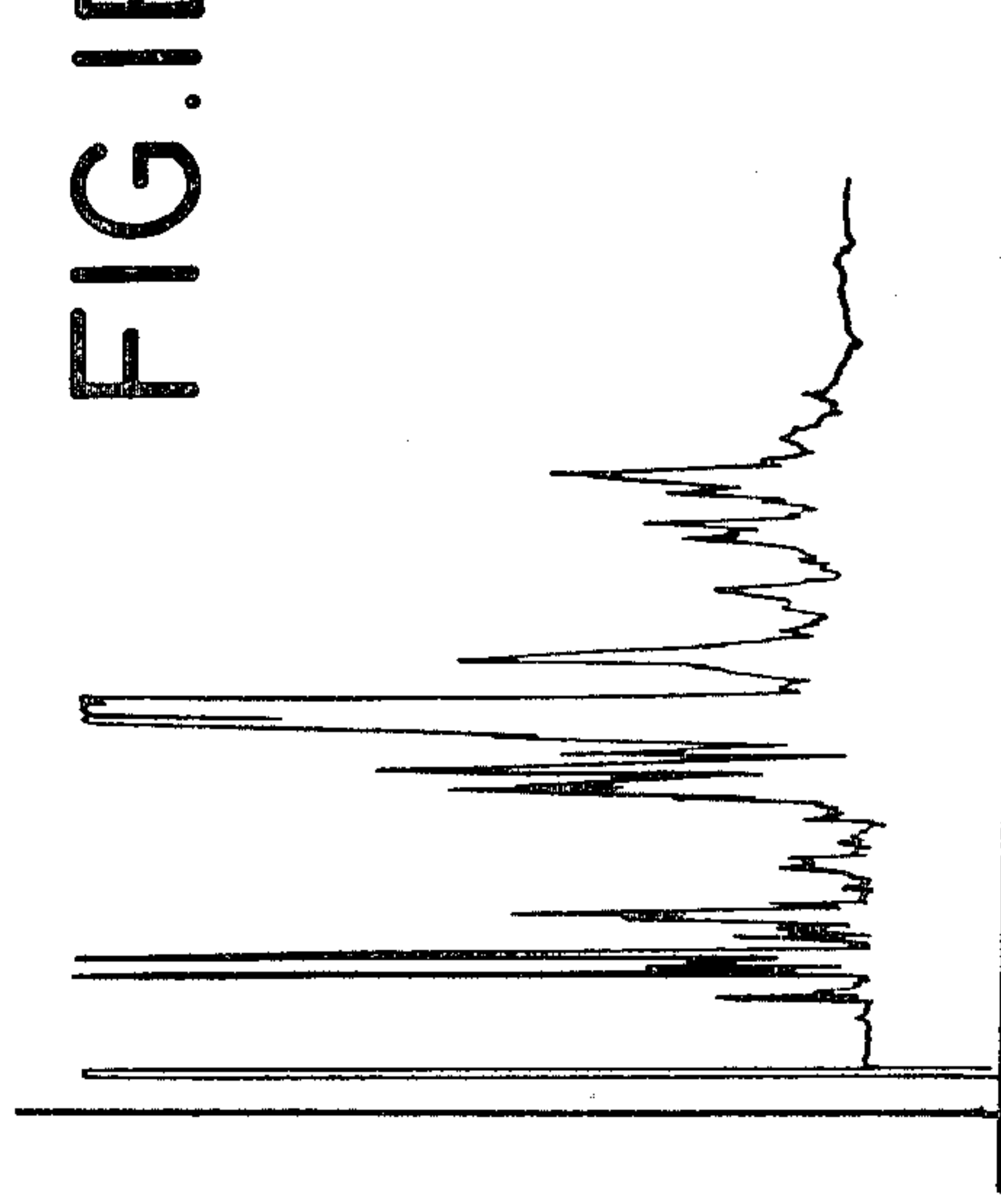
GLC PROFILE FOR EXAMPLE I.
