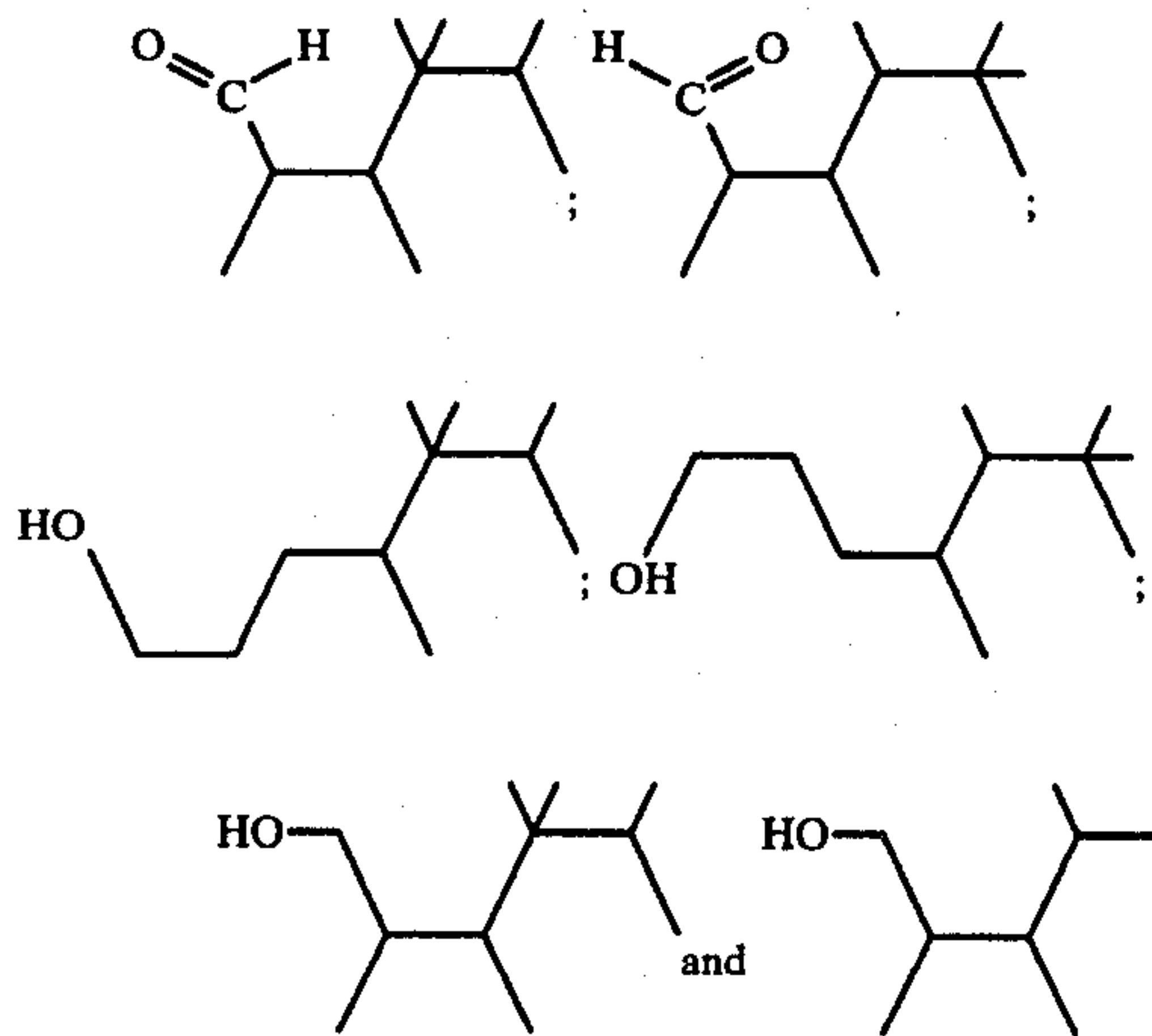
FIG. 6 is the GLC profile for the diisoundecanal compounds produced according to Example II having the structures:
