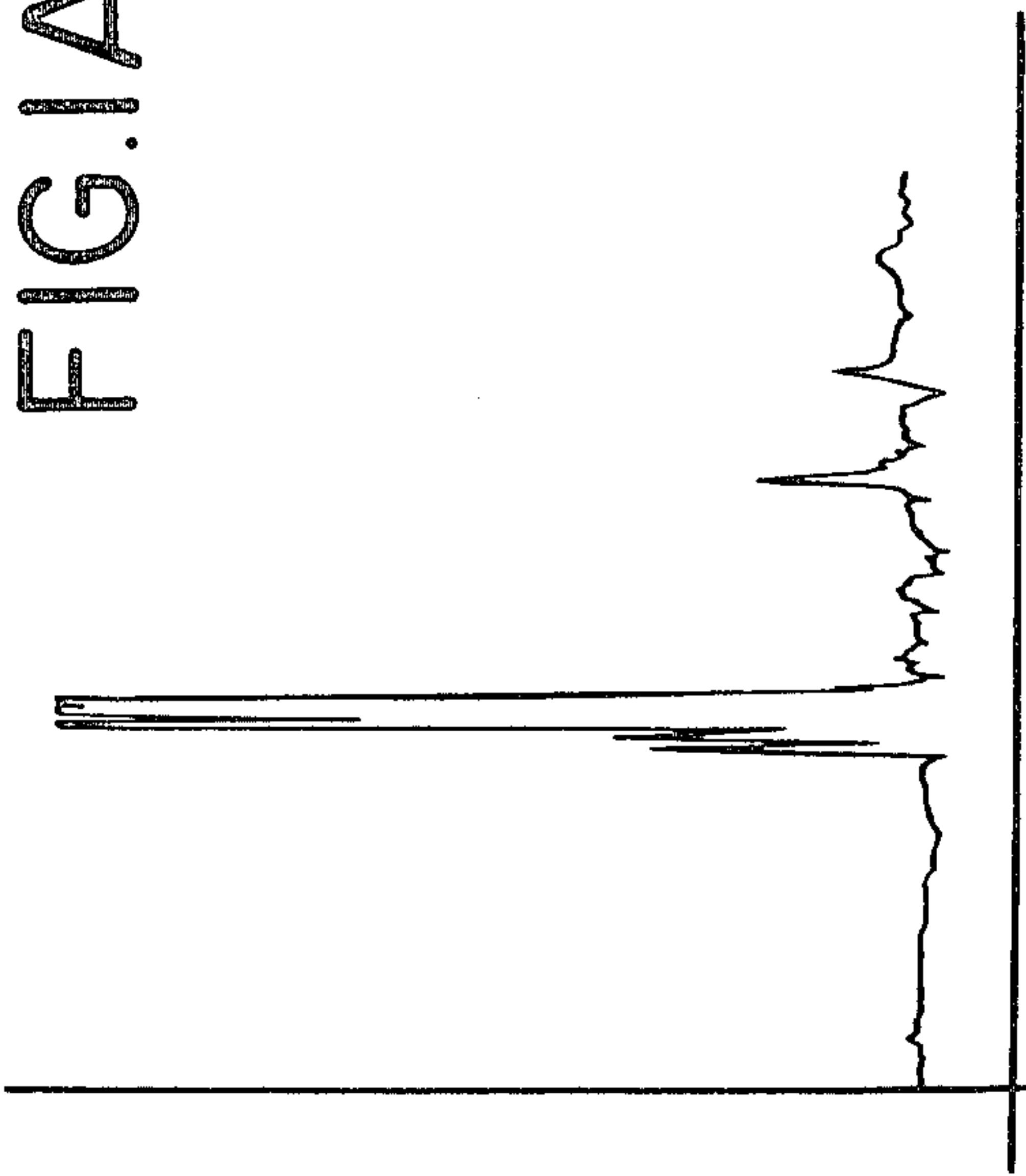
GLC PROFILE FOR EXAMPLE I.
