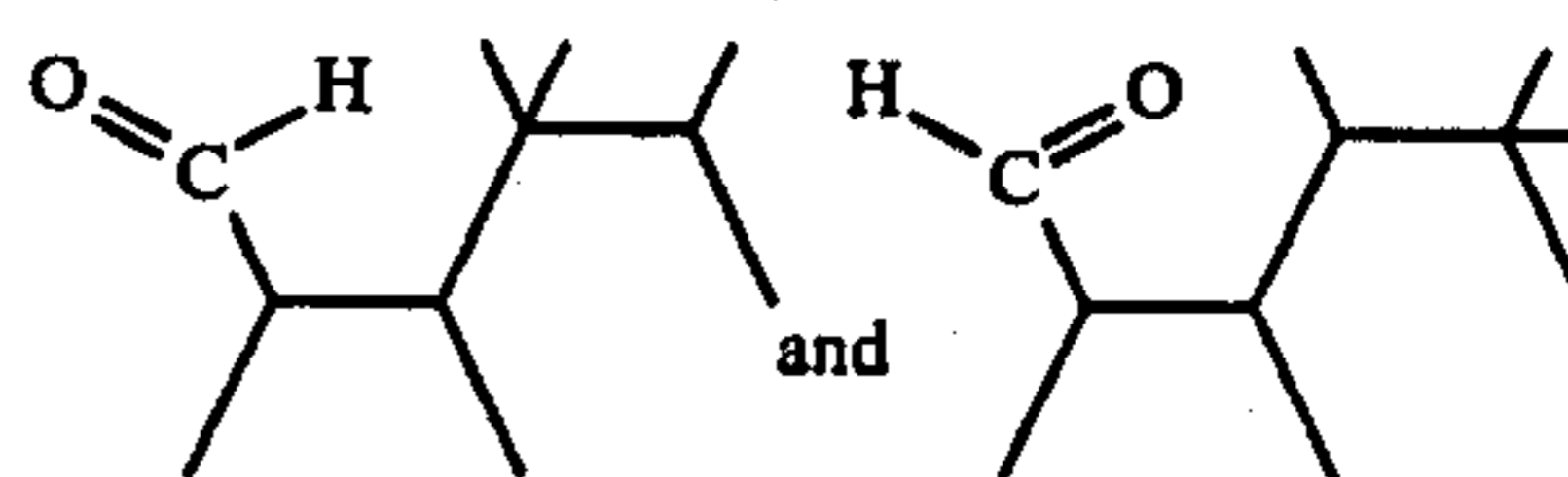
FIG. 9 is the GLC profile (conditions: SF-96, 6" x 1/4" 180° C. isothermal column) produced according to Example II containing the compounds having the structures:
