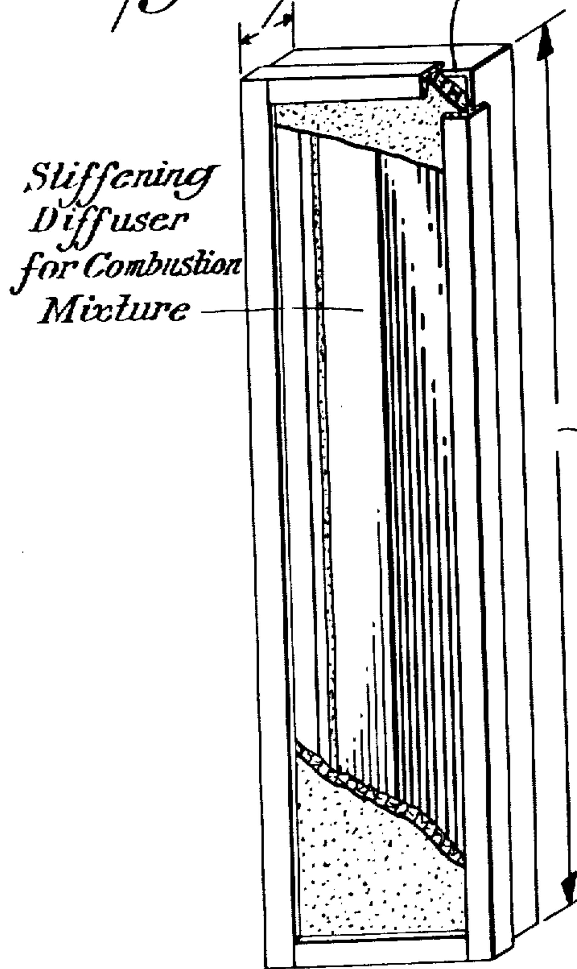
Fig. 16. about 2 1/2 inches deep 1/16 inch thick stainless steel sheet
