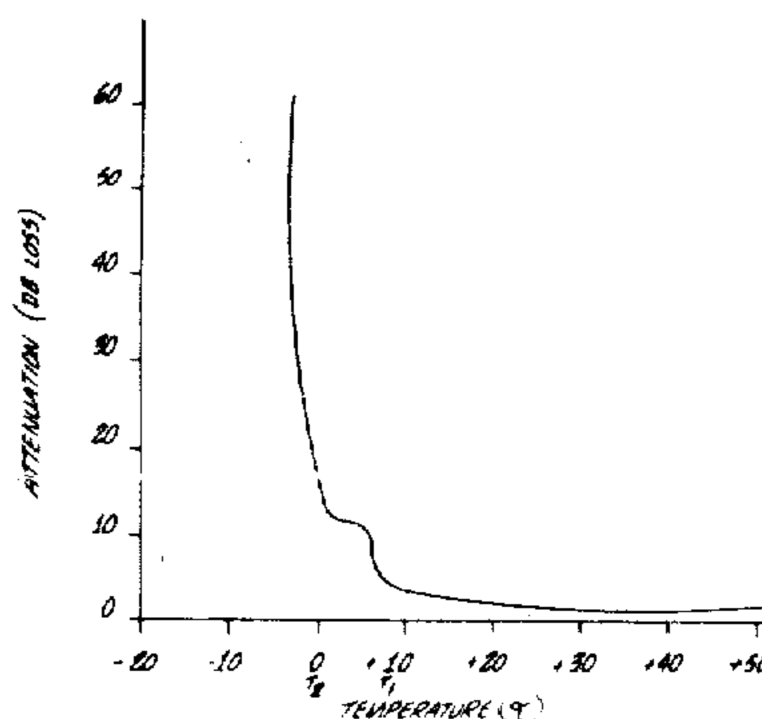
ATTENUATION WITH DOUBLE CLADDING
