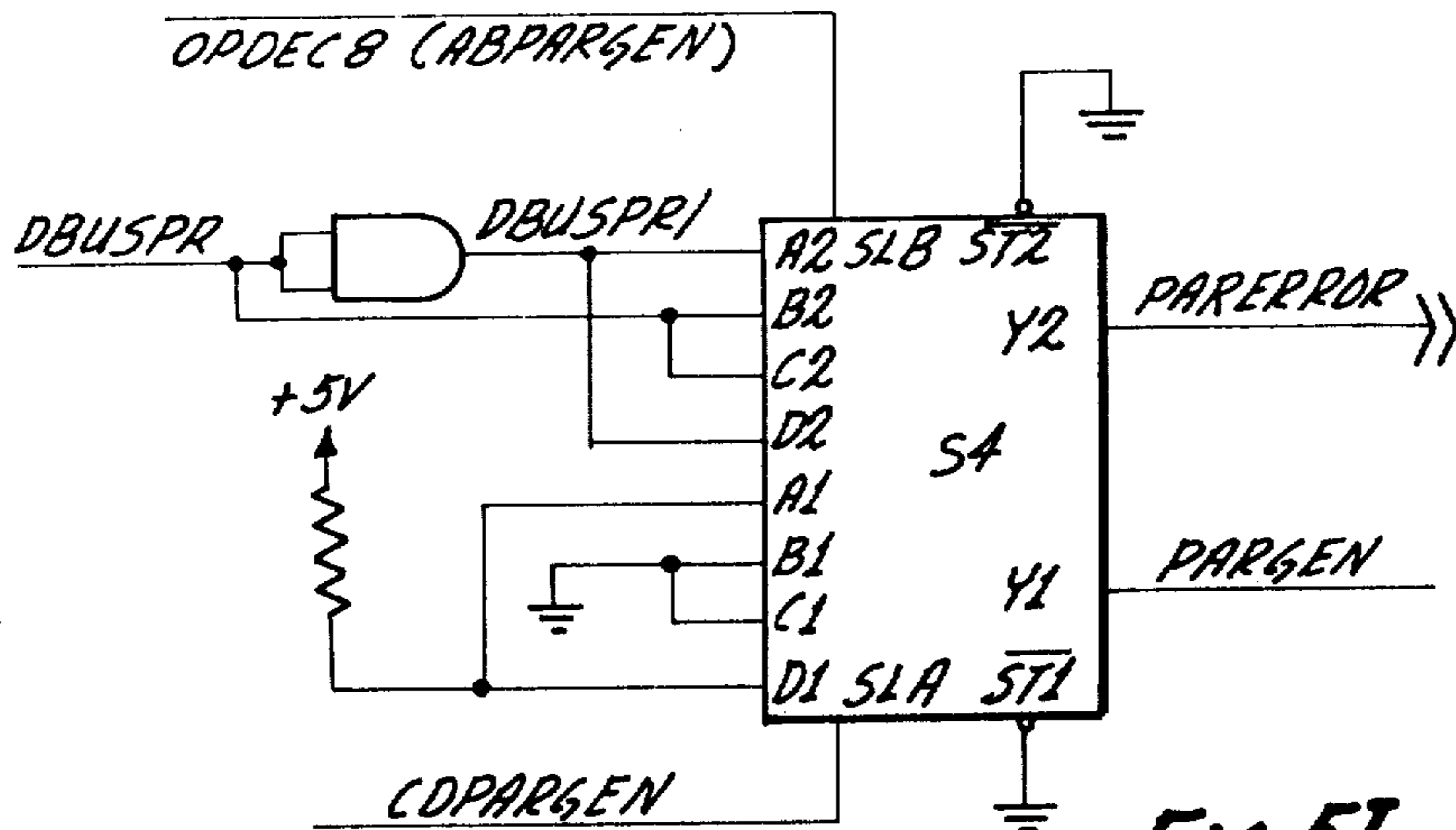
VERTICAL PARITY GENERATION/ CHECK
