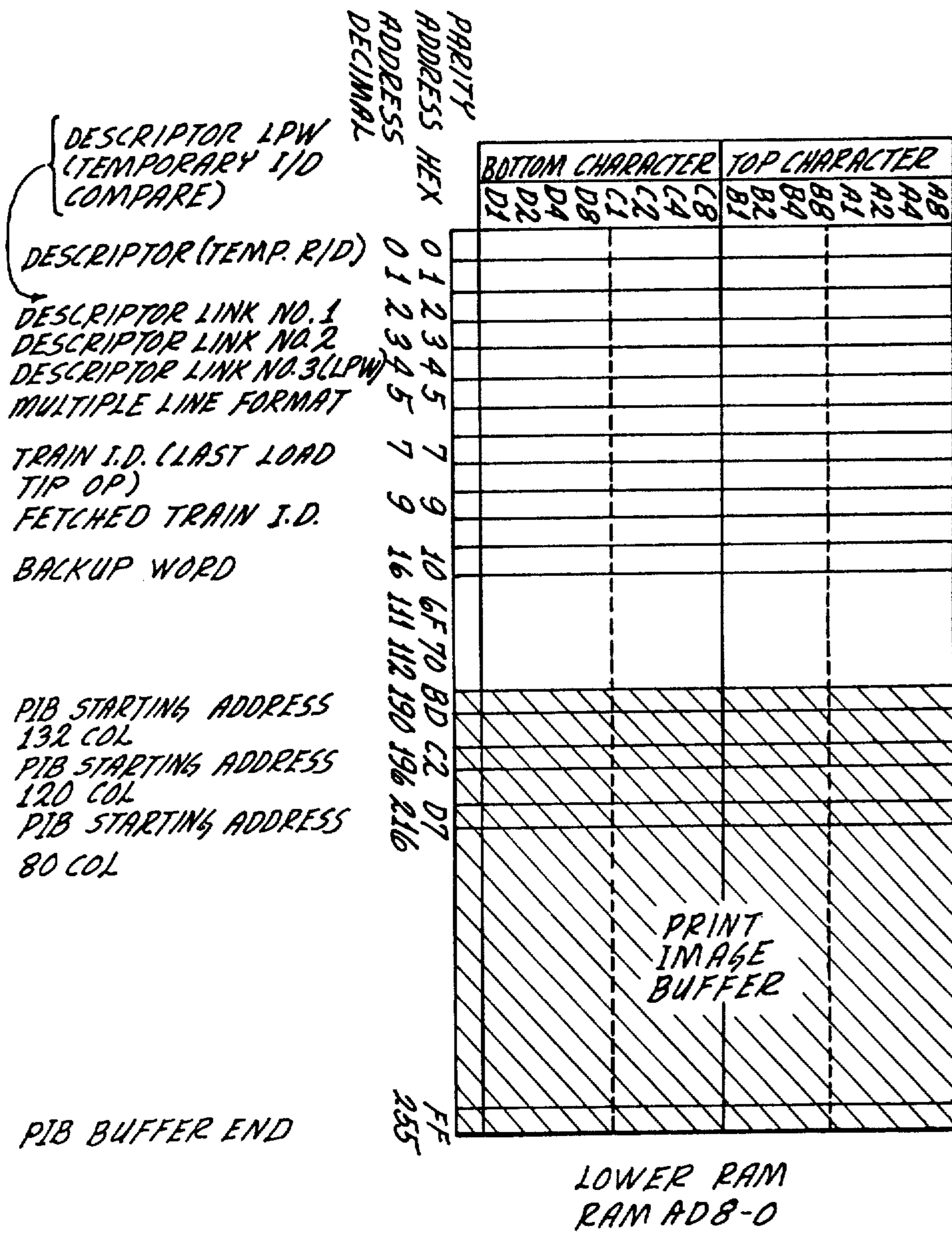
FIG. 5C-1 MEMORY USAGE
