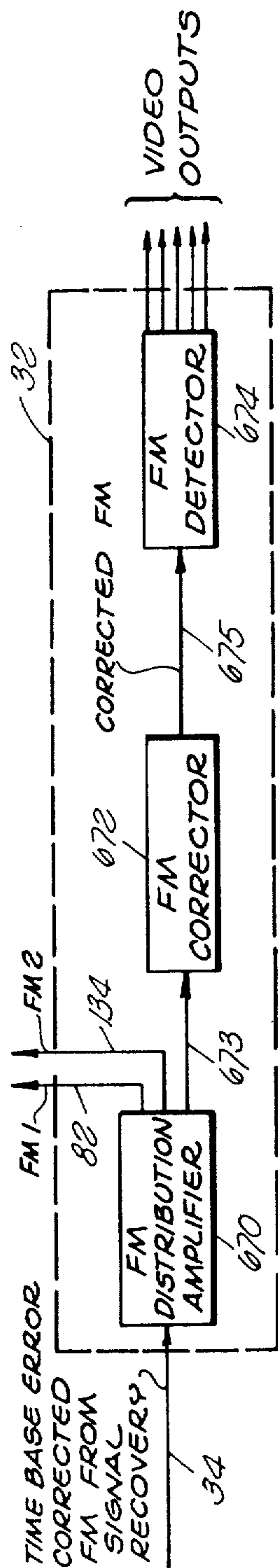
FIG. 14 FM PROCESSING
