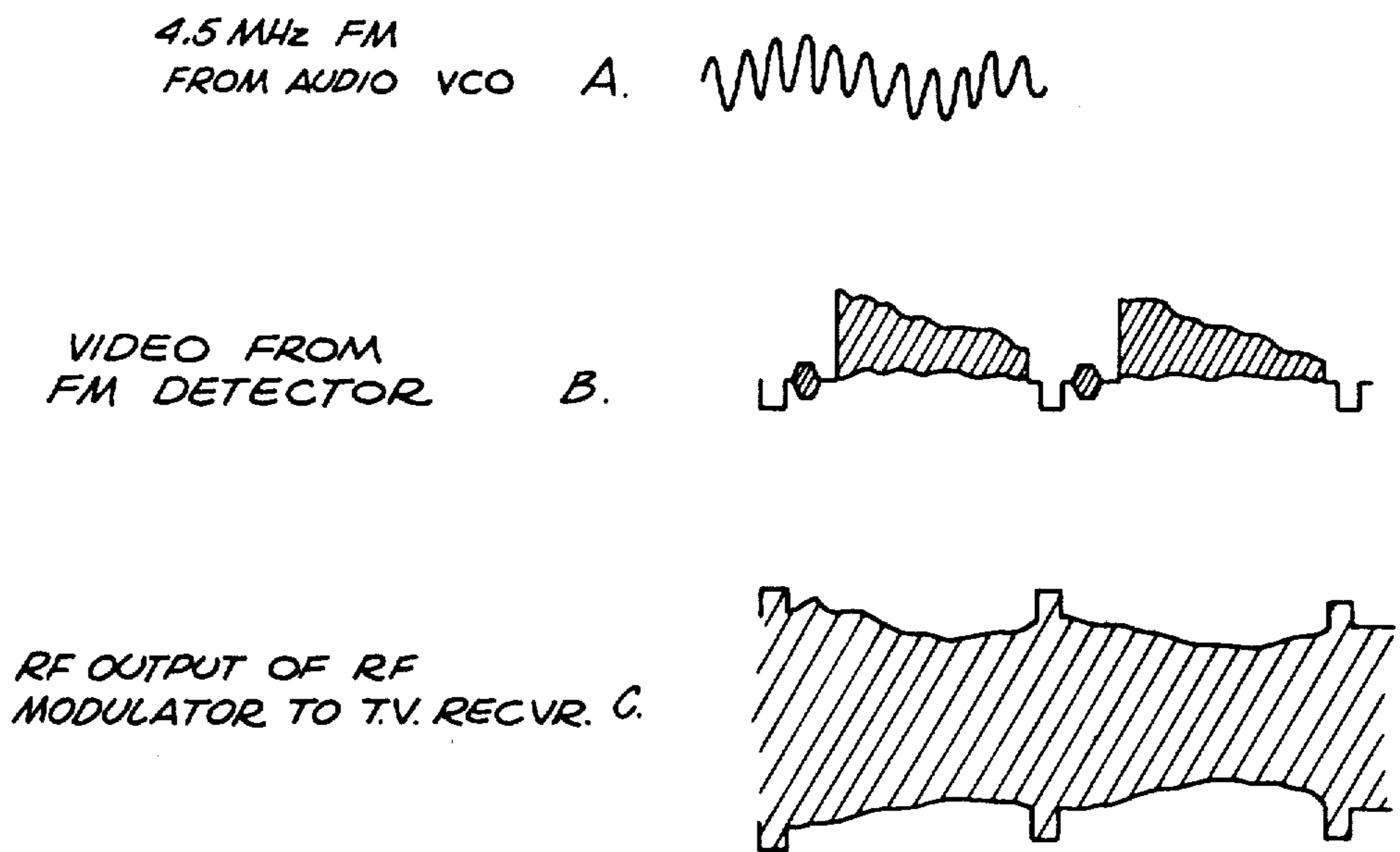
FIG. 25 RF MODULATOR
