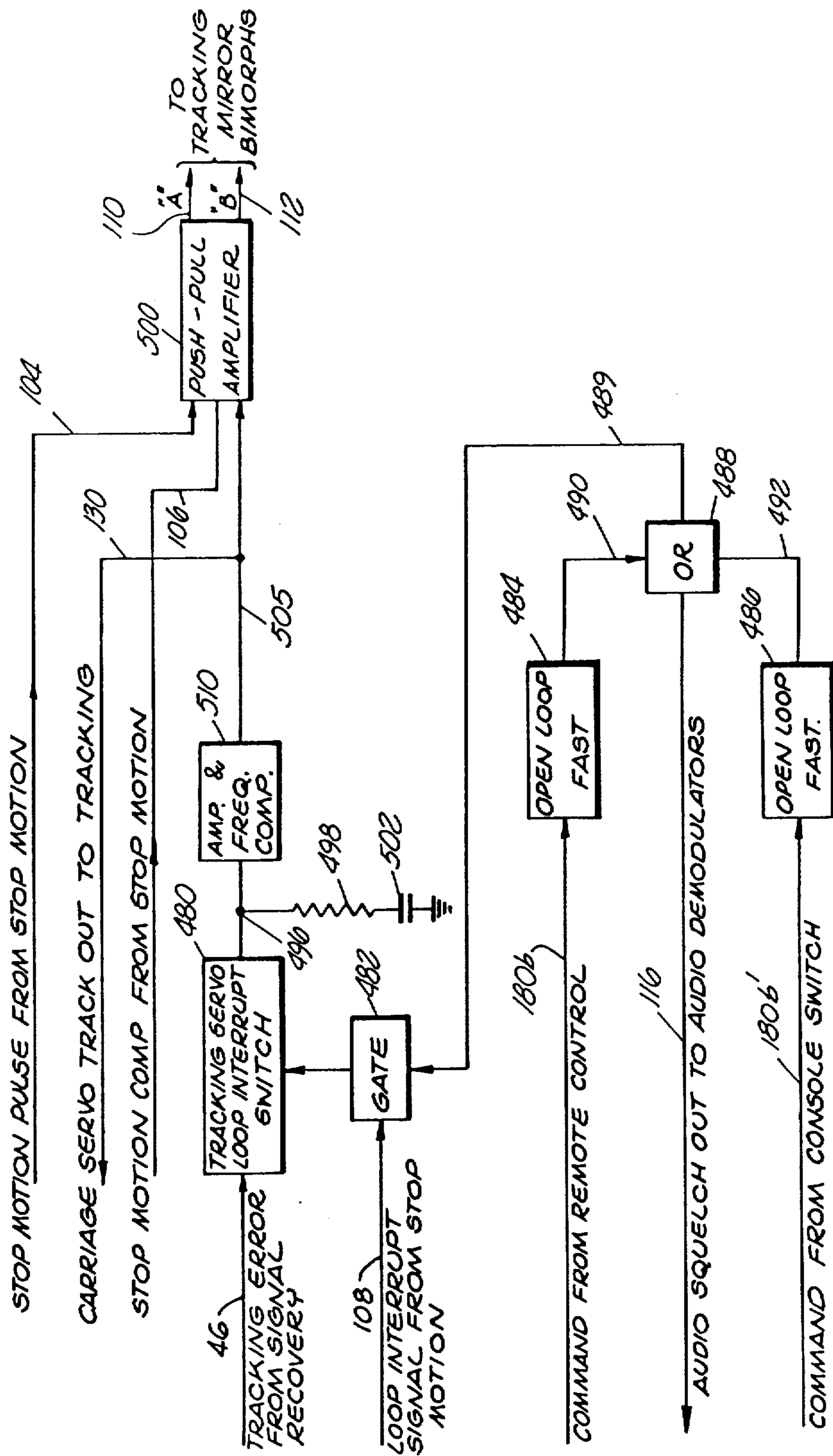
FIG. 9 TRACKING SERVO
