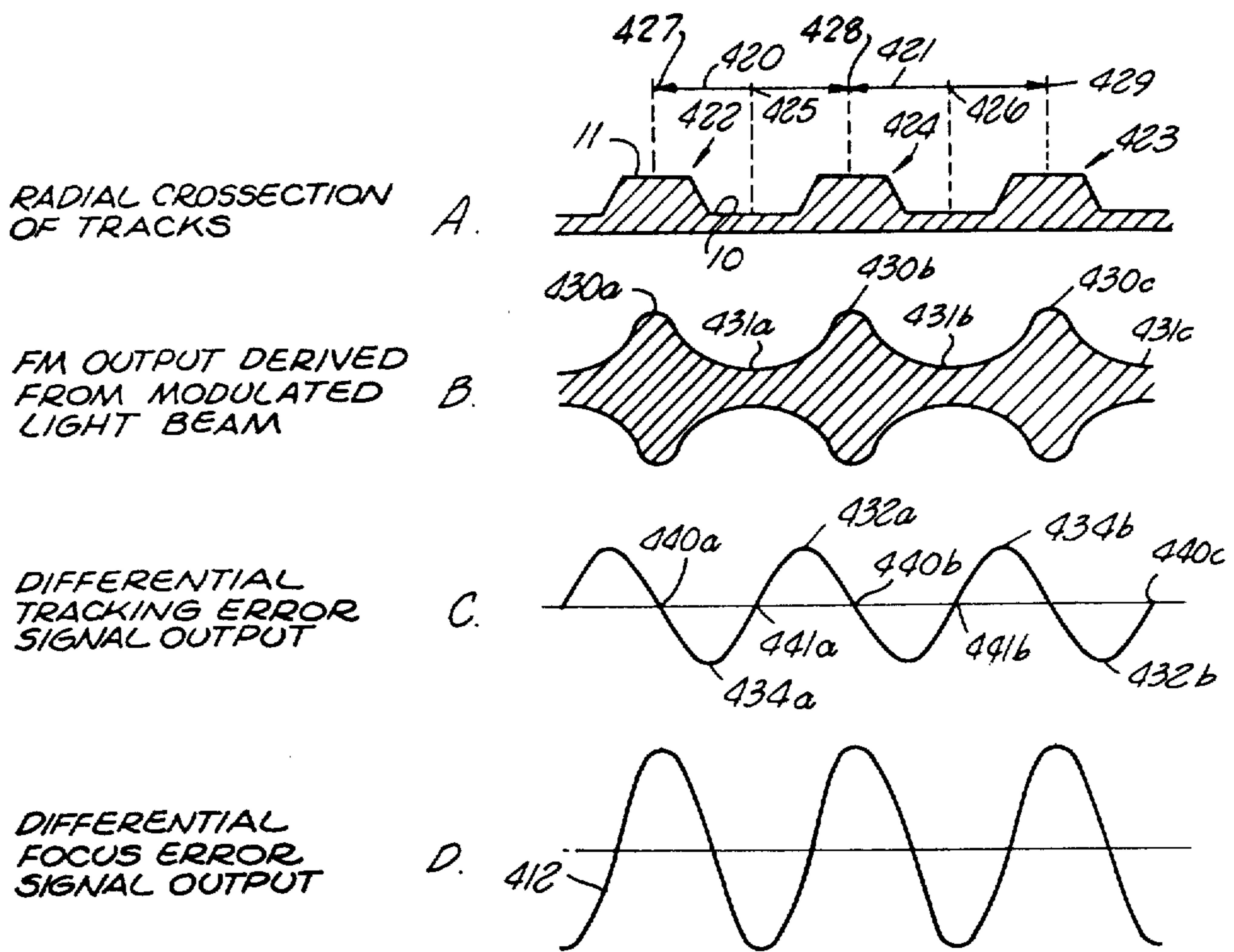
FIG. 8 SIGNAL RECOVERY
