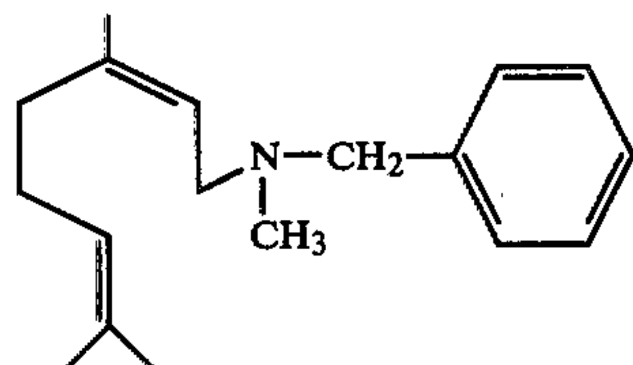
N-neryl-N-methylbenzylamine (XI)
