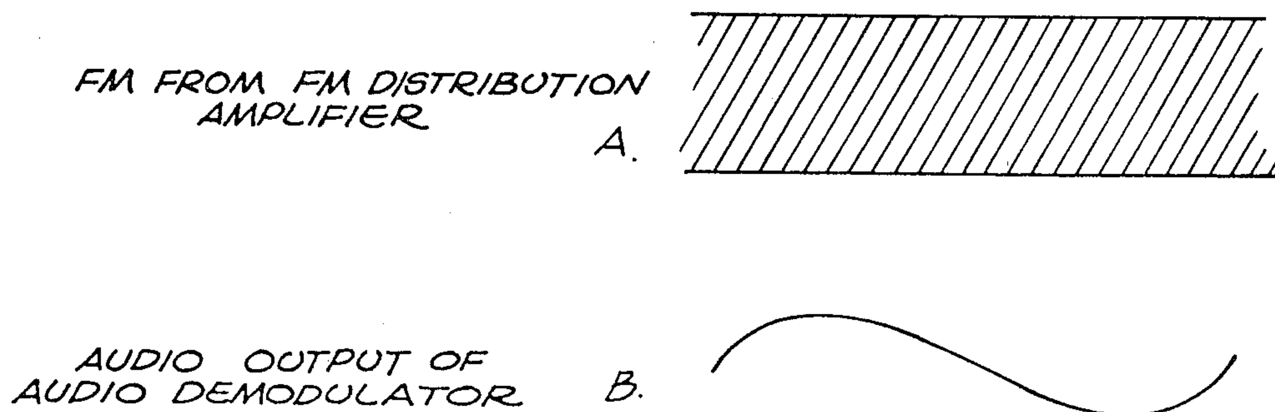
FIG. 21 AUDIO DEMODULATOR
