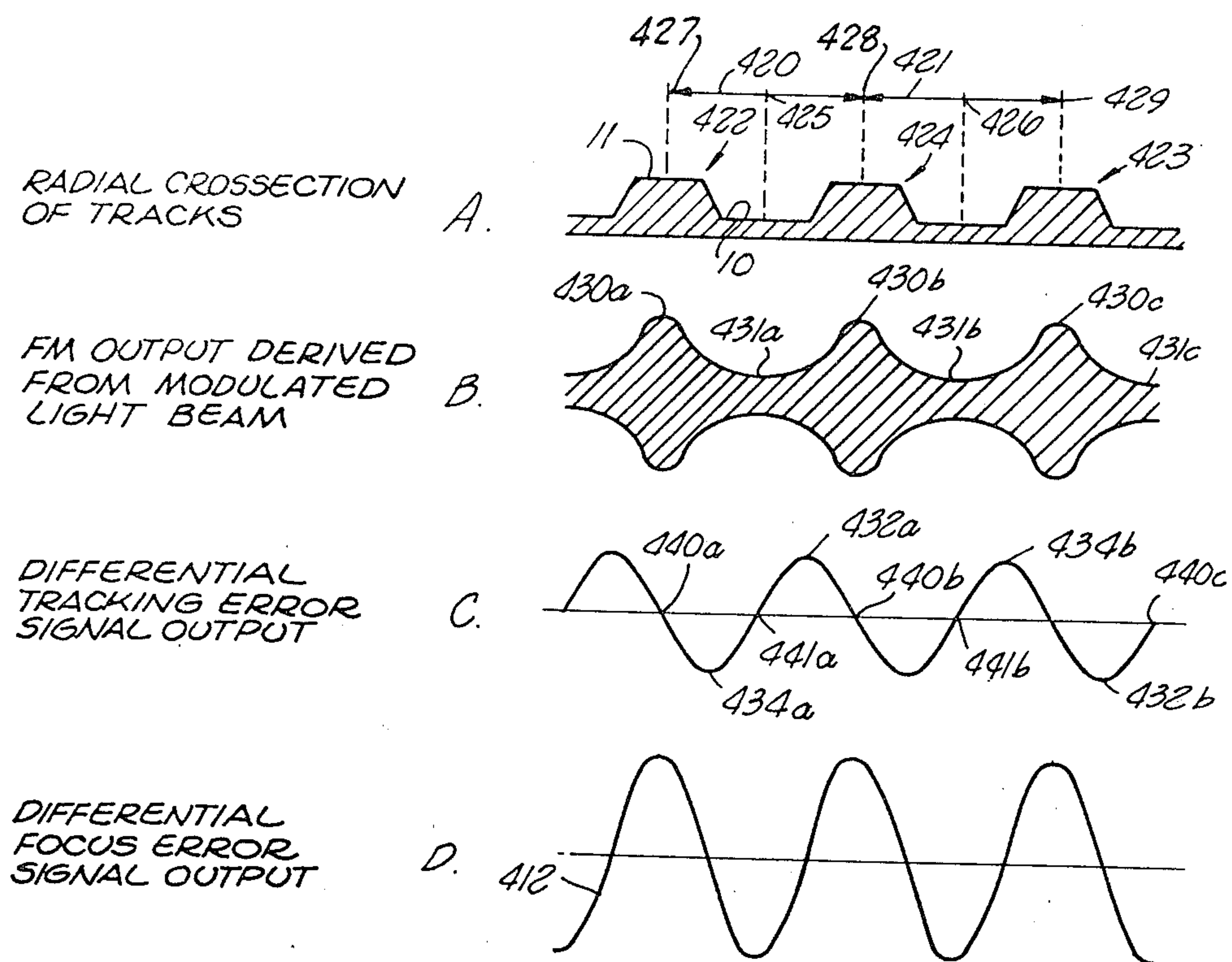
FIG. 8 SIGNAL RECOVERY
