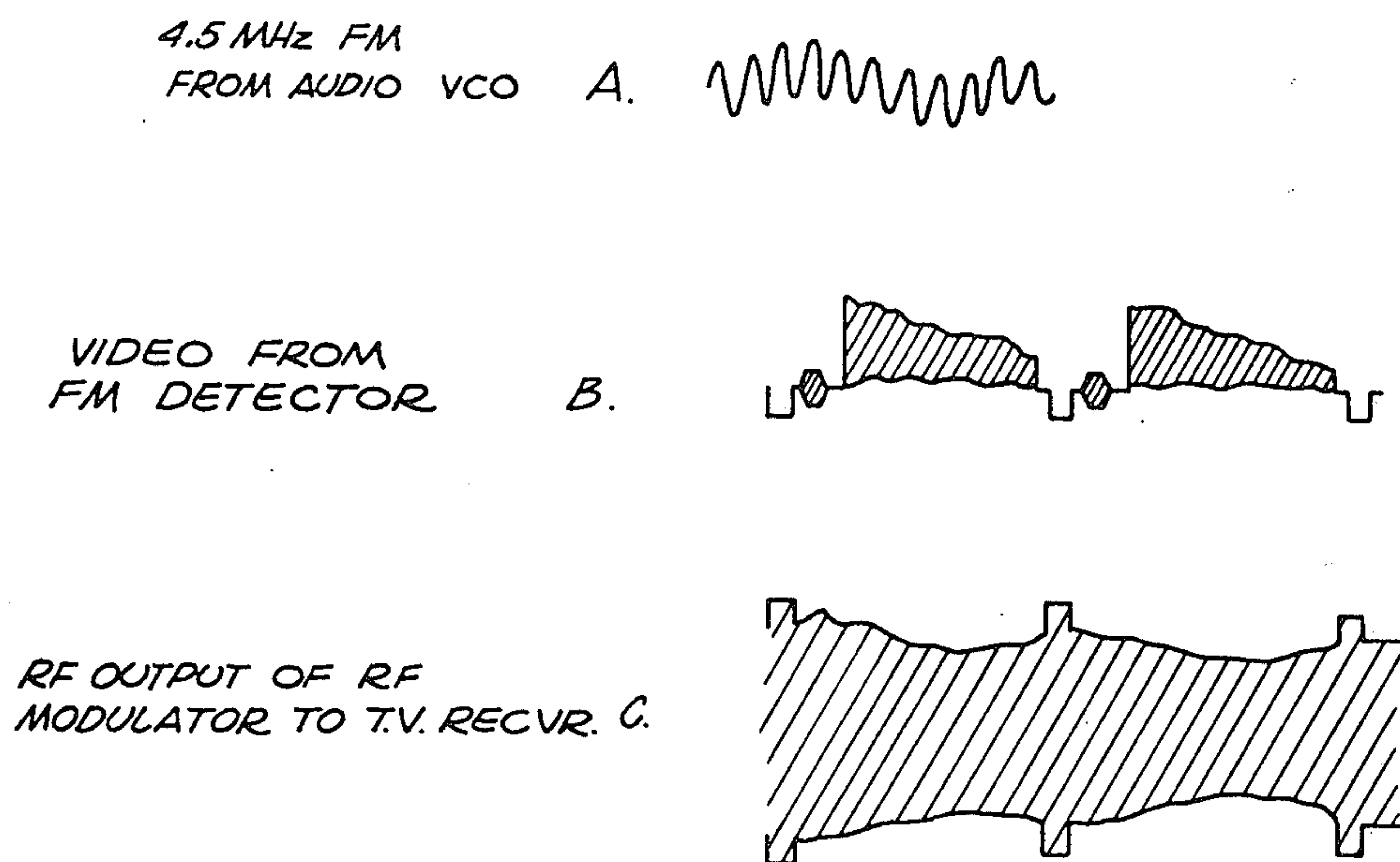
FIG. 25 RF MODULATOR
