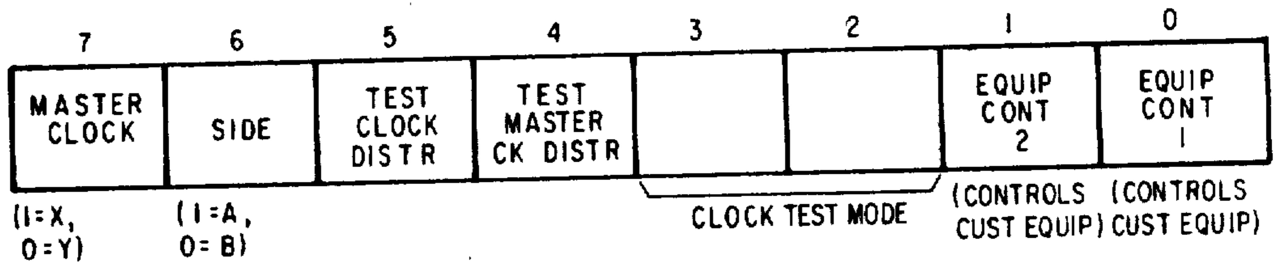
FIG. 25b CONTROL REGISTER 2 BIT FORMAT
