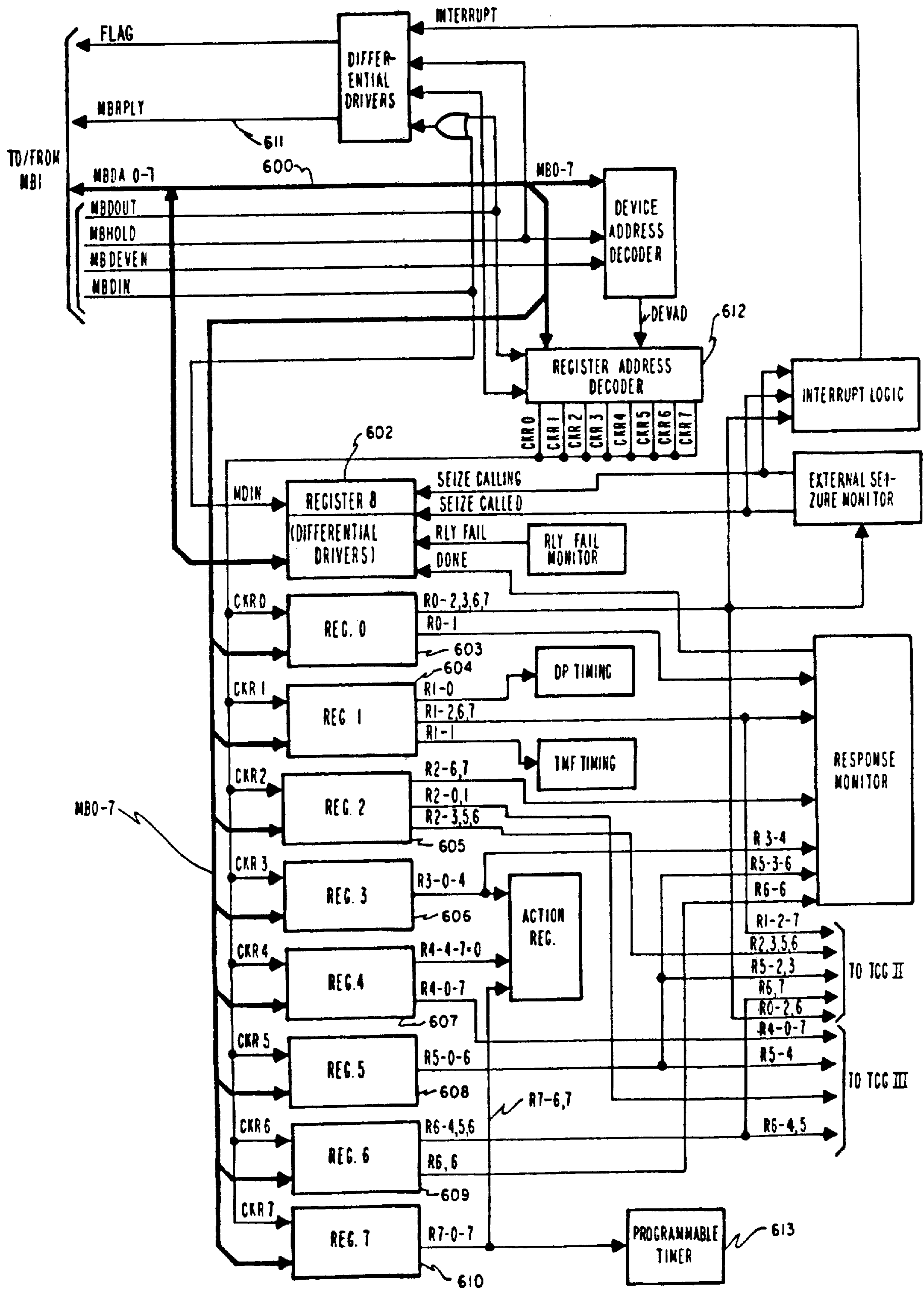
FUNCTIONAL BLOCK DIAGRAM TEST CALL GENERATOR I
