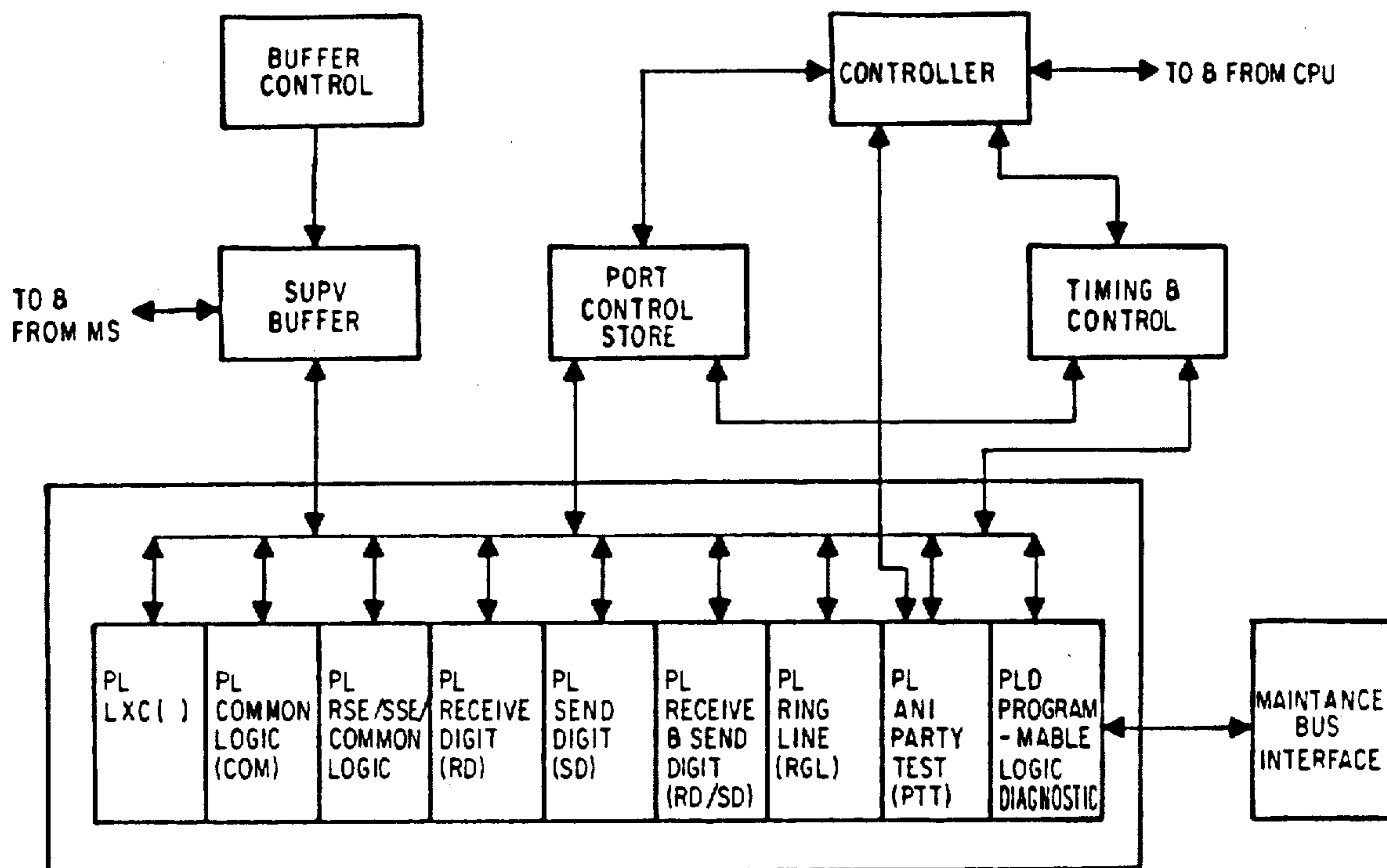
FIG. 17 PROGRAMMABLE LOGIC DIAGNOSTIC BLOCK DIAGRAM
