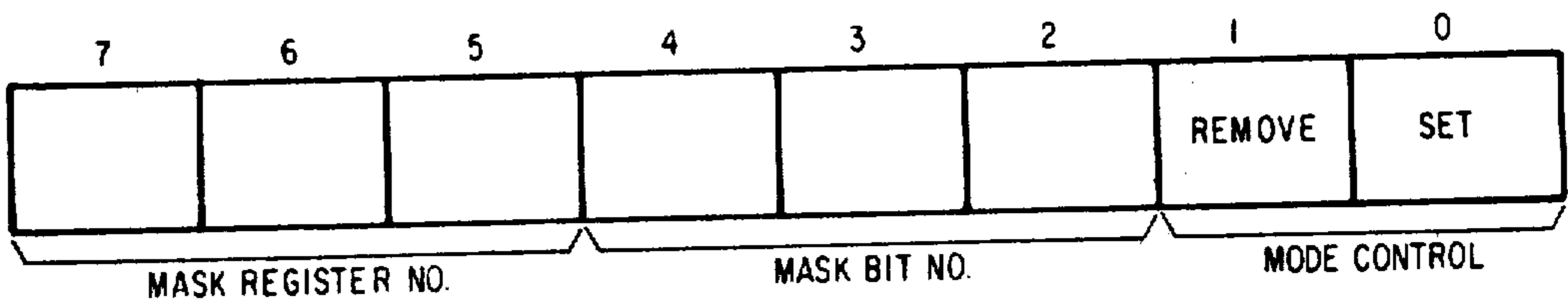
FIG. 25a MASK CONTROL REGISTER 1 BIT FORMAT
