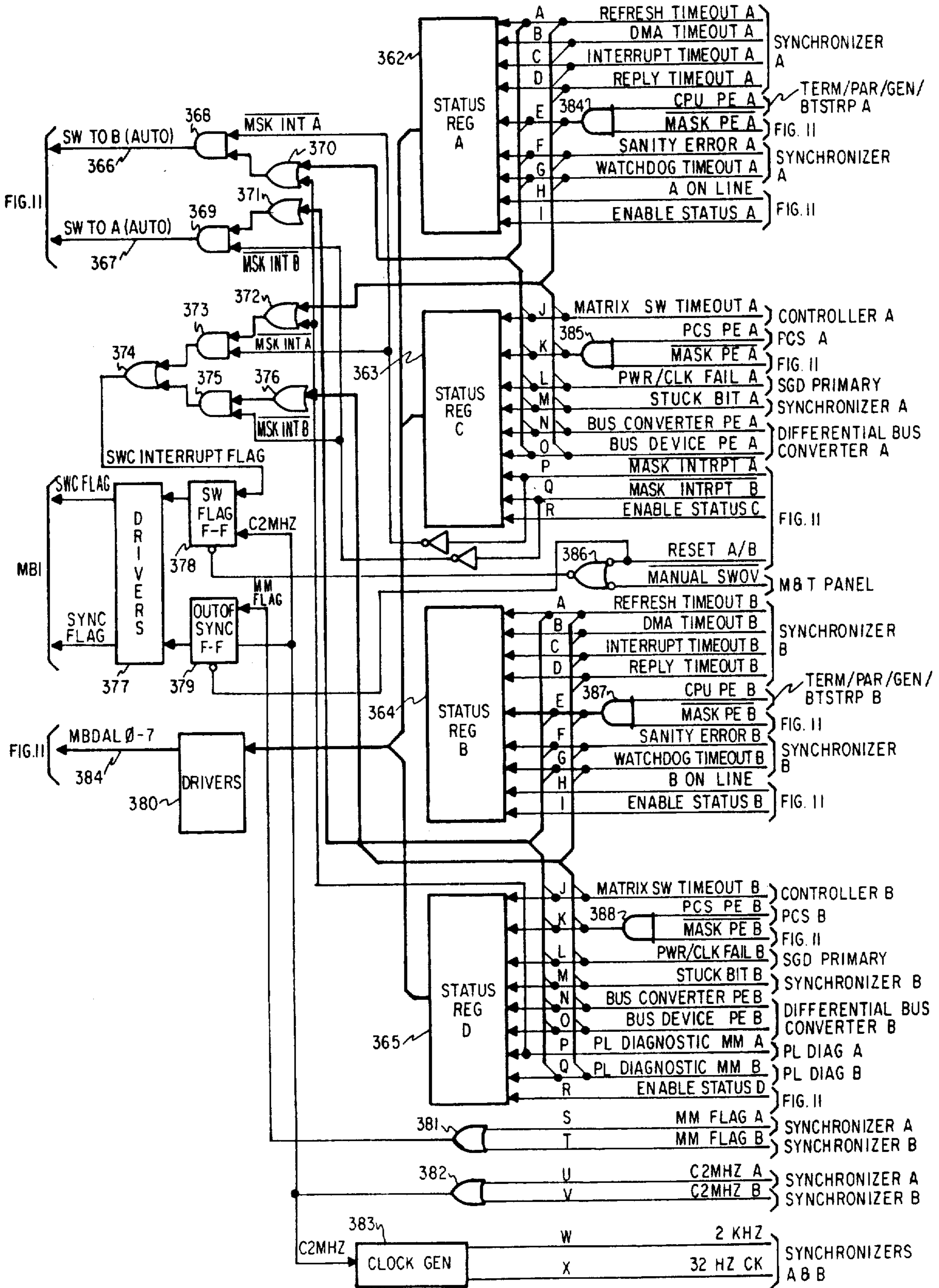
FIG. 10 SWITCHOVER CONTROL
