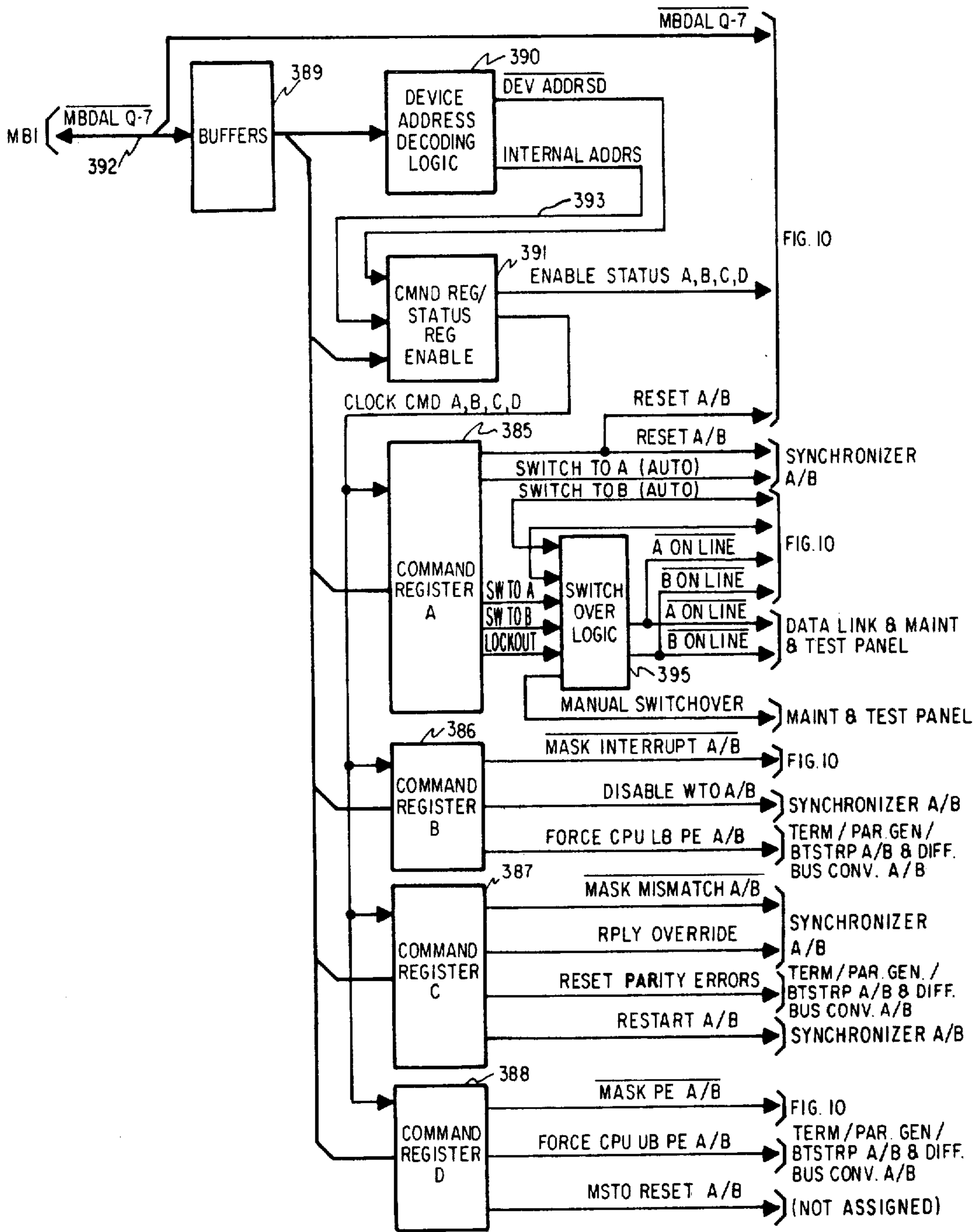
FIG. II SWITCHOVER CONTROL
