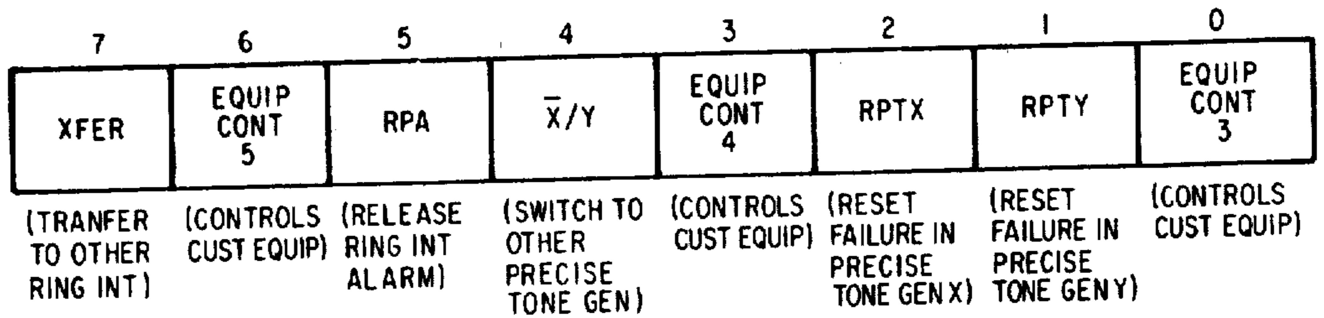
FIG. 25c CONTROL REGISTER BIT FORMAT
