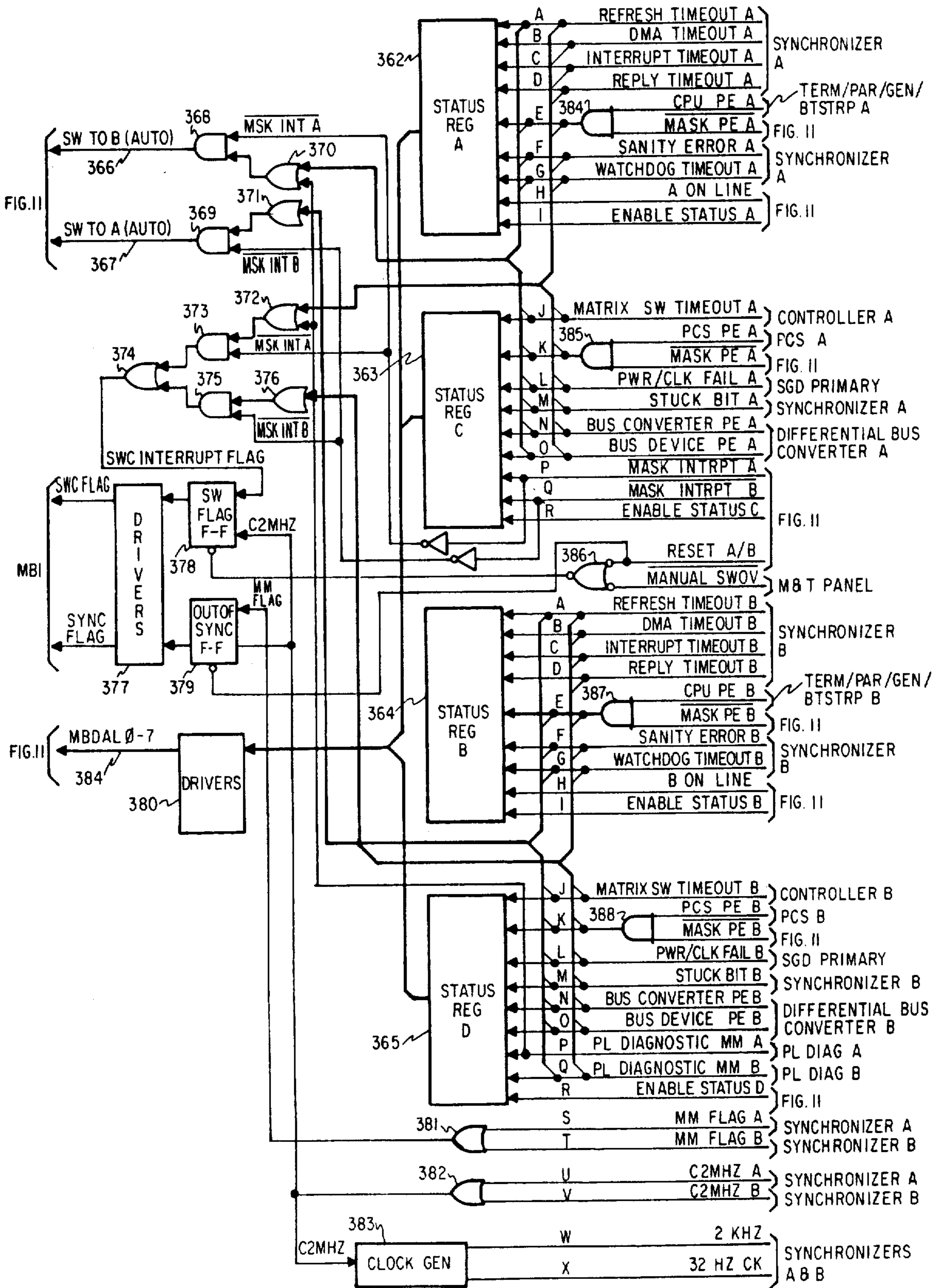
FIG. 10 SWITCHOVER CONTROL
