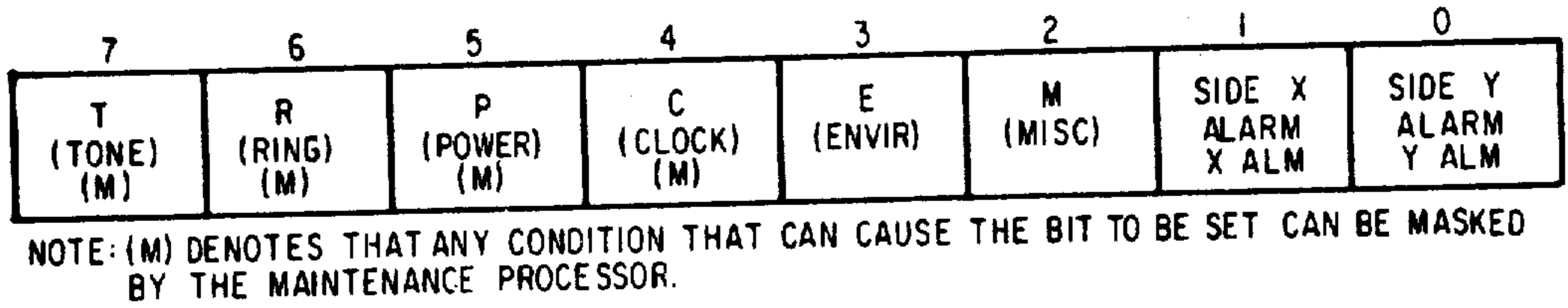
FIG. 24g SGD STATUS REGISTER BIT FORMAT
