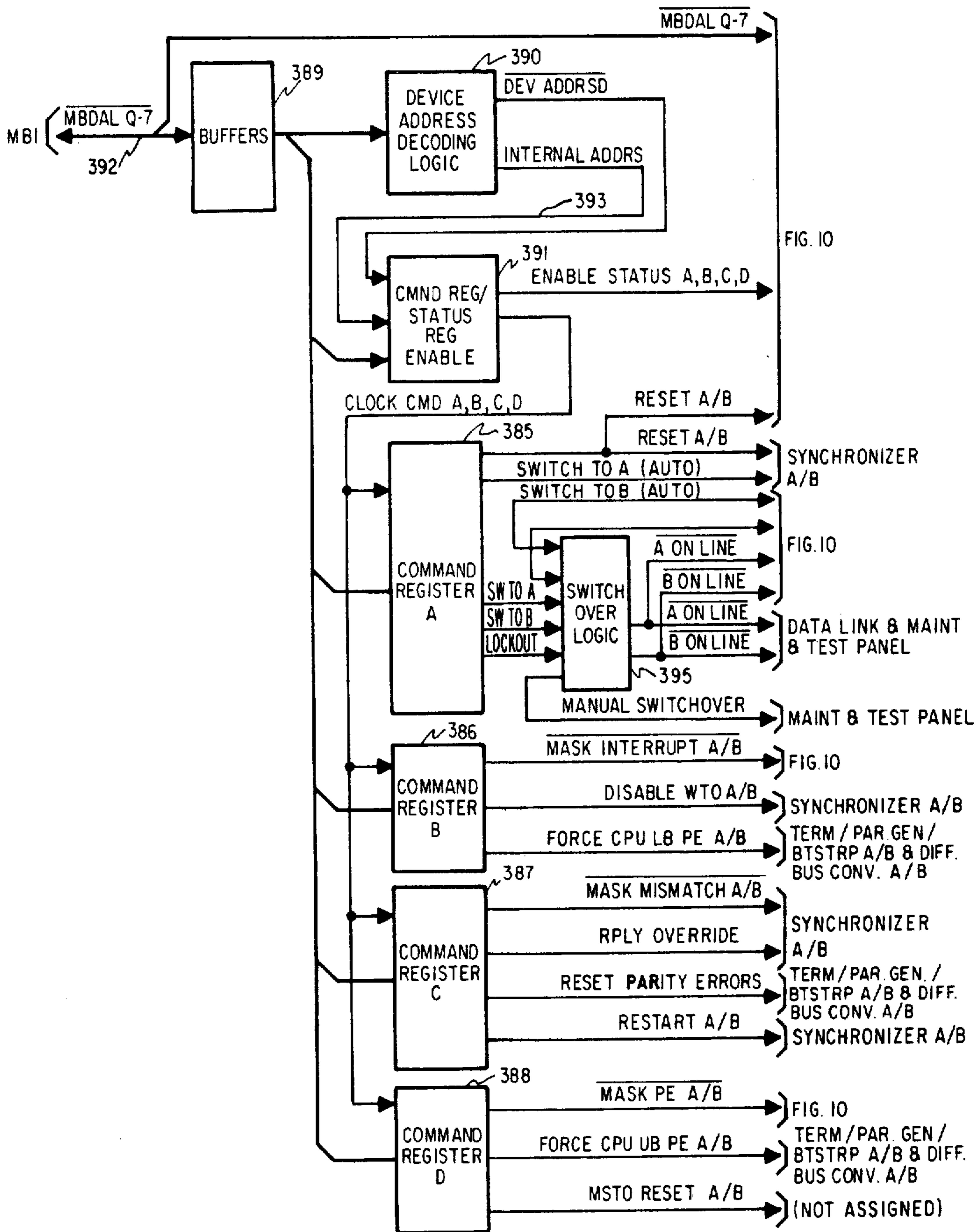
FIG. II SWITCHOVER CONTROL
