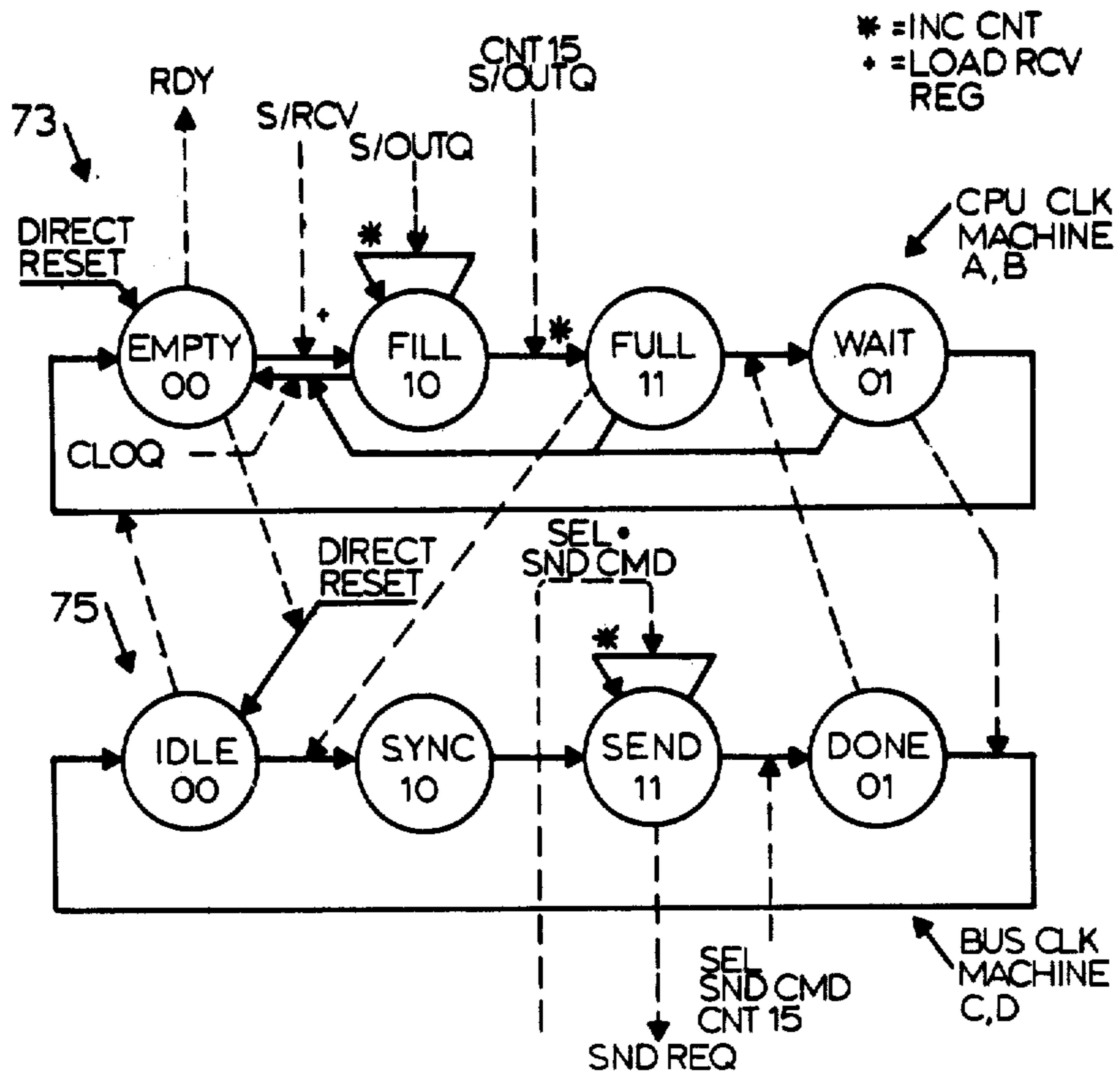
BUS EMPTY STATE LOGIC DIAGRAM
