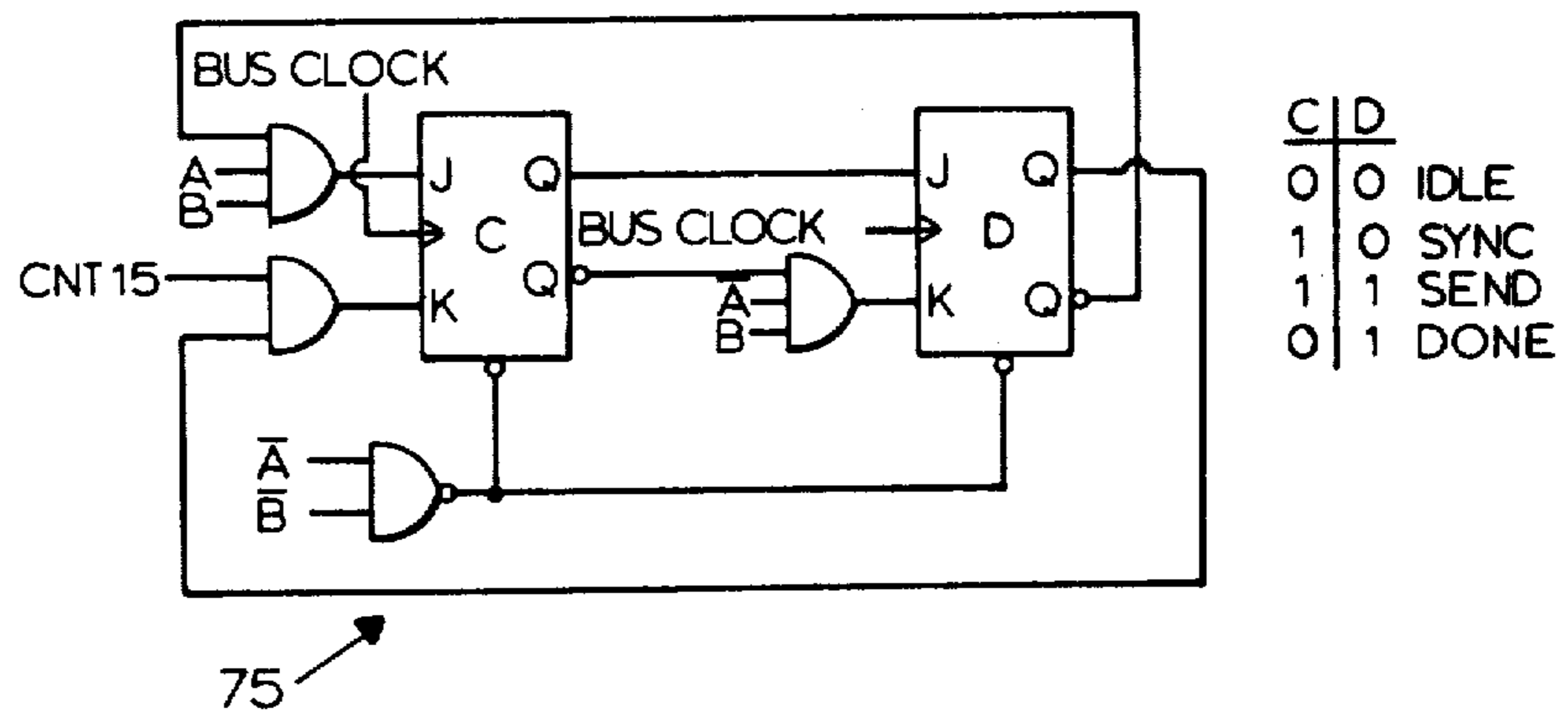
BUS EMPTY STATE LOGIC
