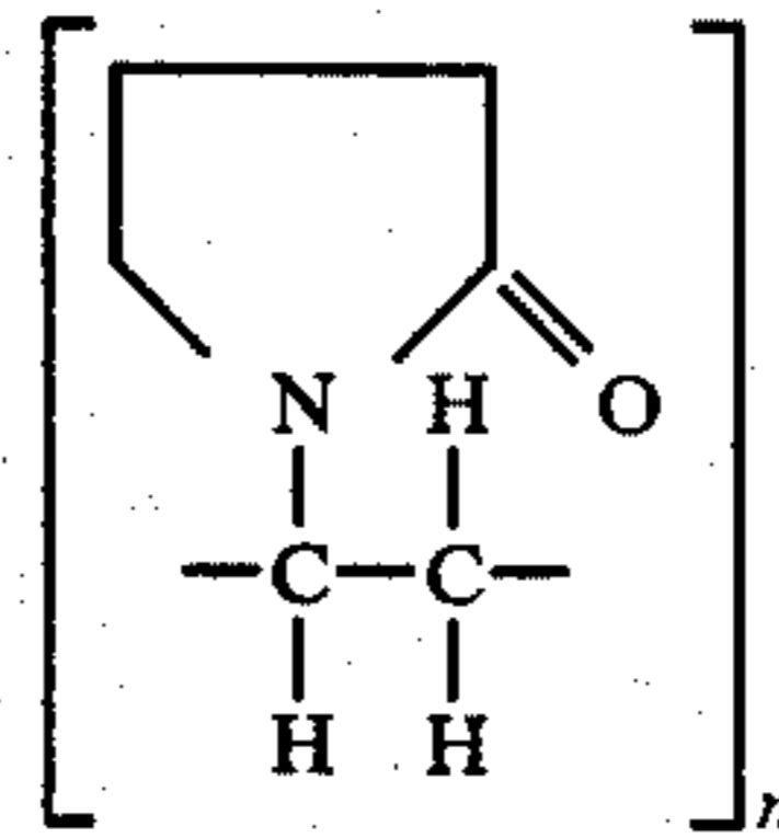
polyvinyl pyrrolidone
