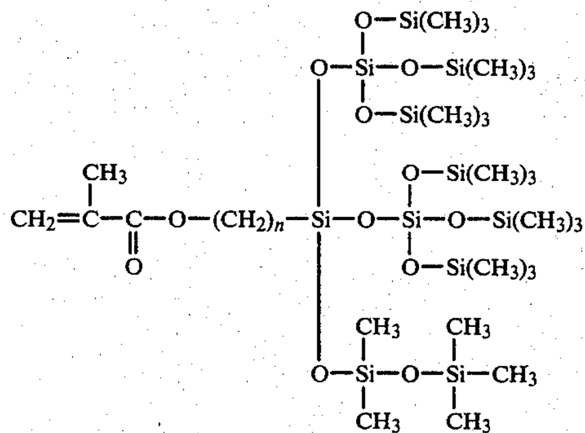
bis(tris-trimethylsiloxy-siloxanyl)monopentamethyldisiloxanylmethacryloxyalkylsilane
