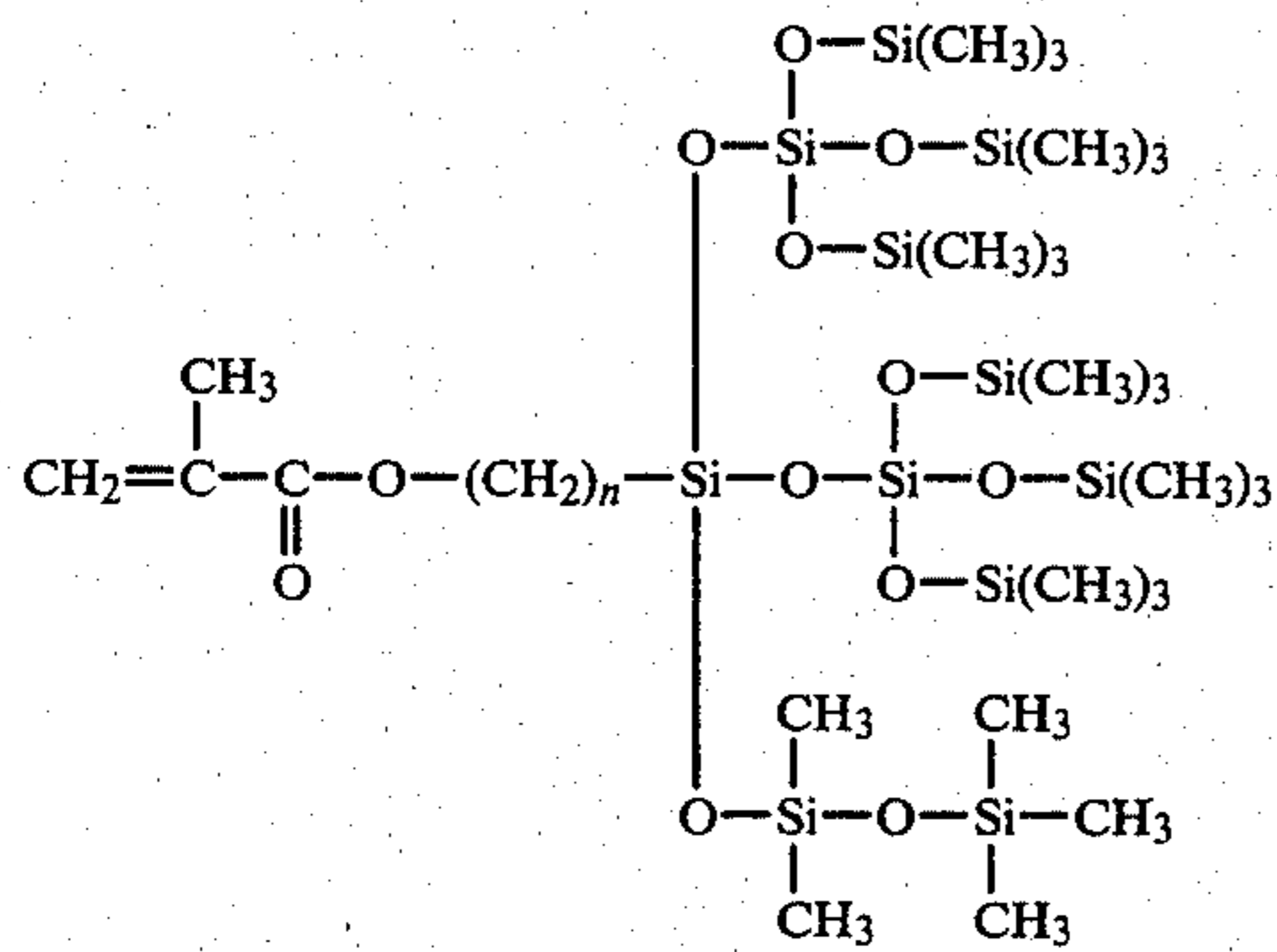
bis(tris-trimethylsiloxy-siloxanyl)monopentamethyldisiloxanylemethacryloxyalkylsilane
