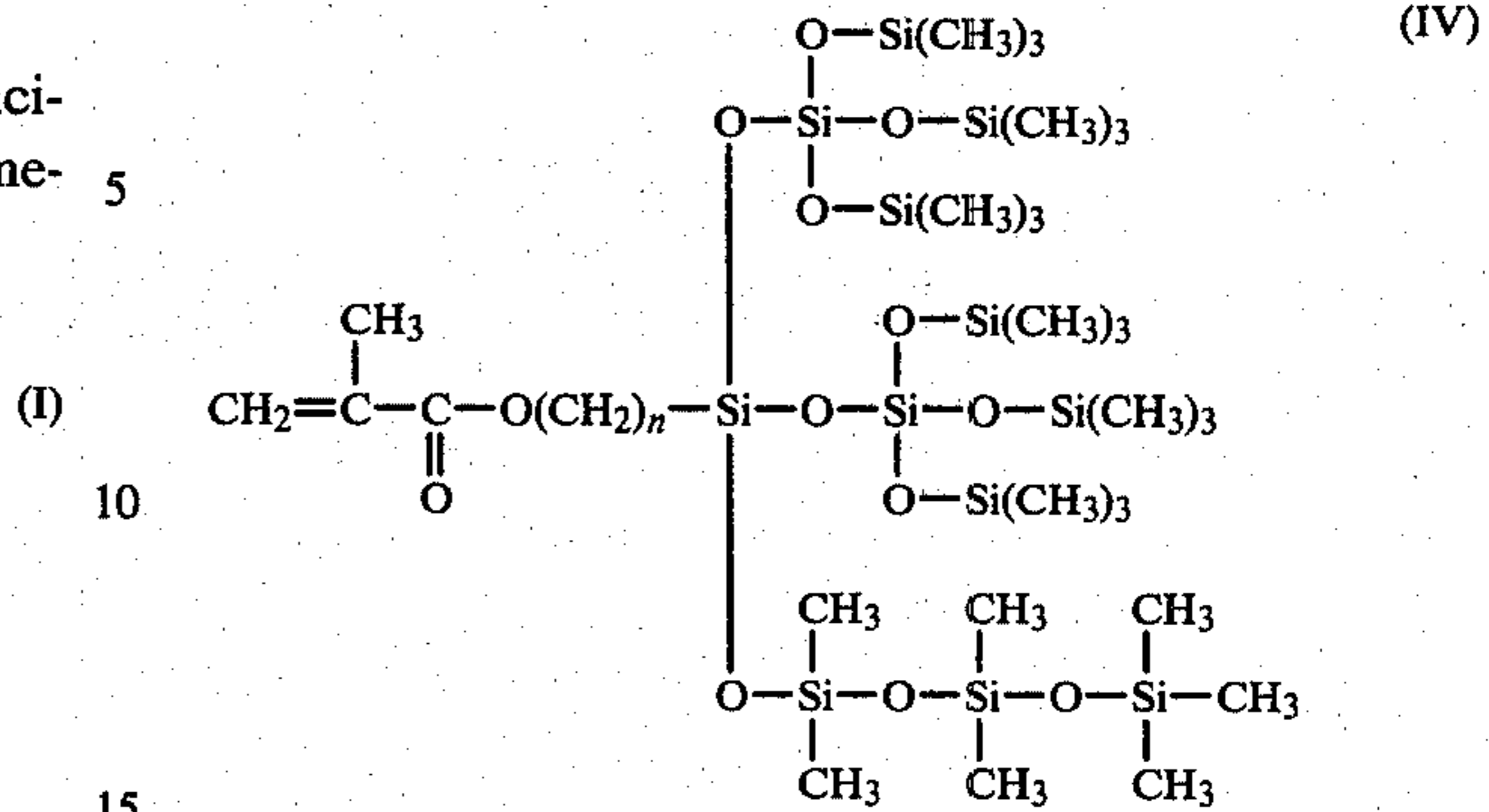
bis(tris-trimethylsiloxy-siloxanyl)mono(heptamethyl-trisiloxanyl)methacryloxyalkylsilane
