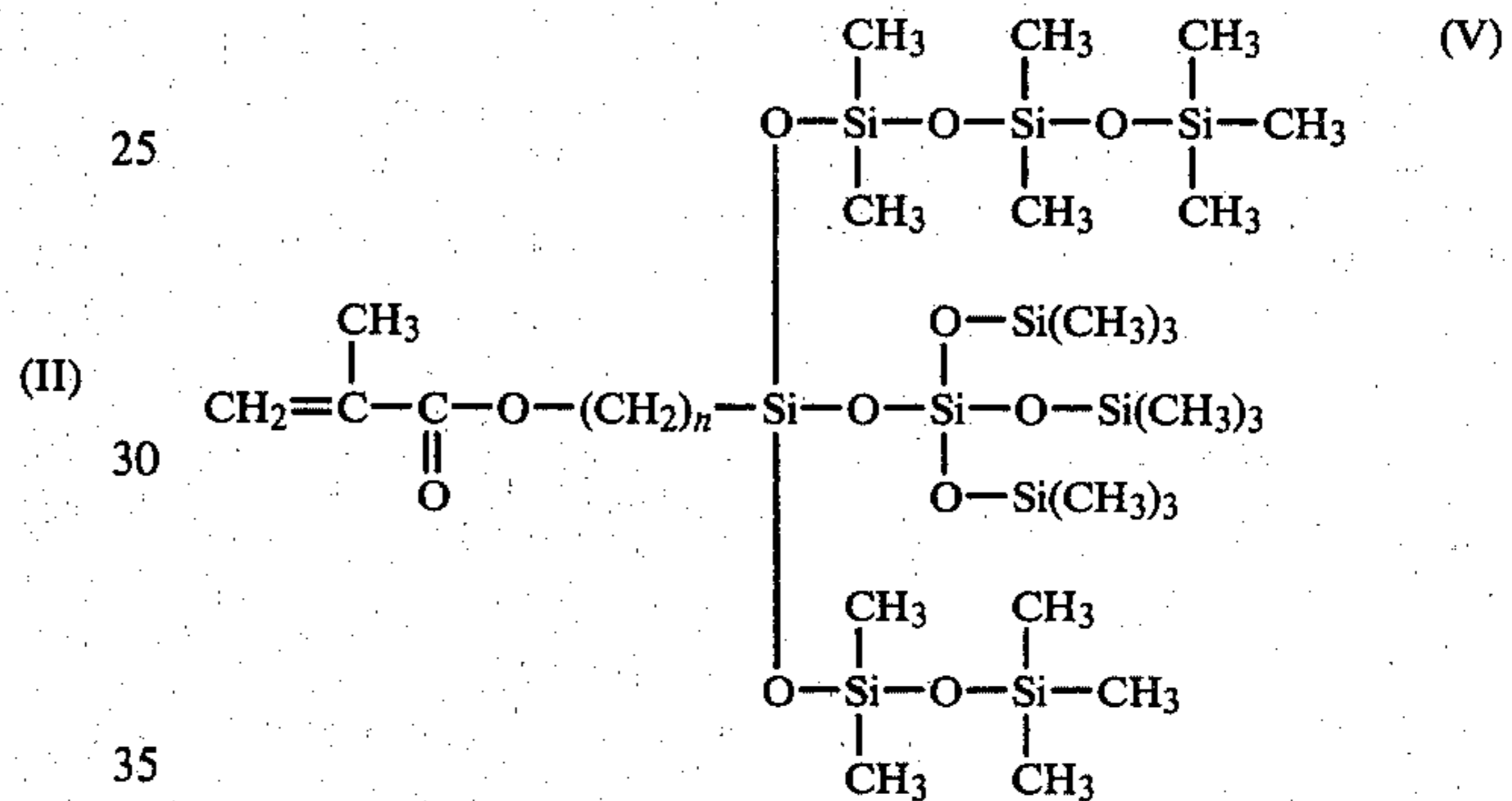
mono(tris-trimethylsiloxy-siloxanyl)mono(heptamethyl-trisiloxanyl)monopentamethyldisiloxanylmethacryloxyalkylsilane
