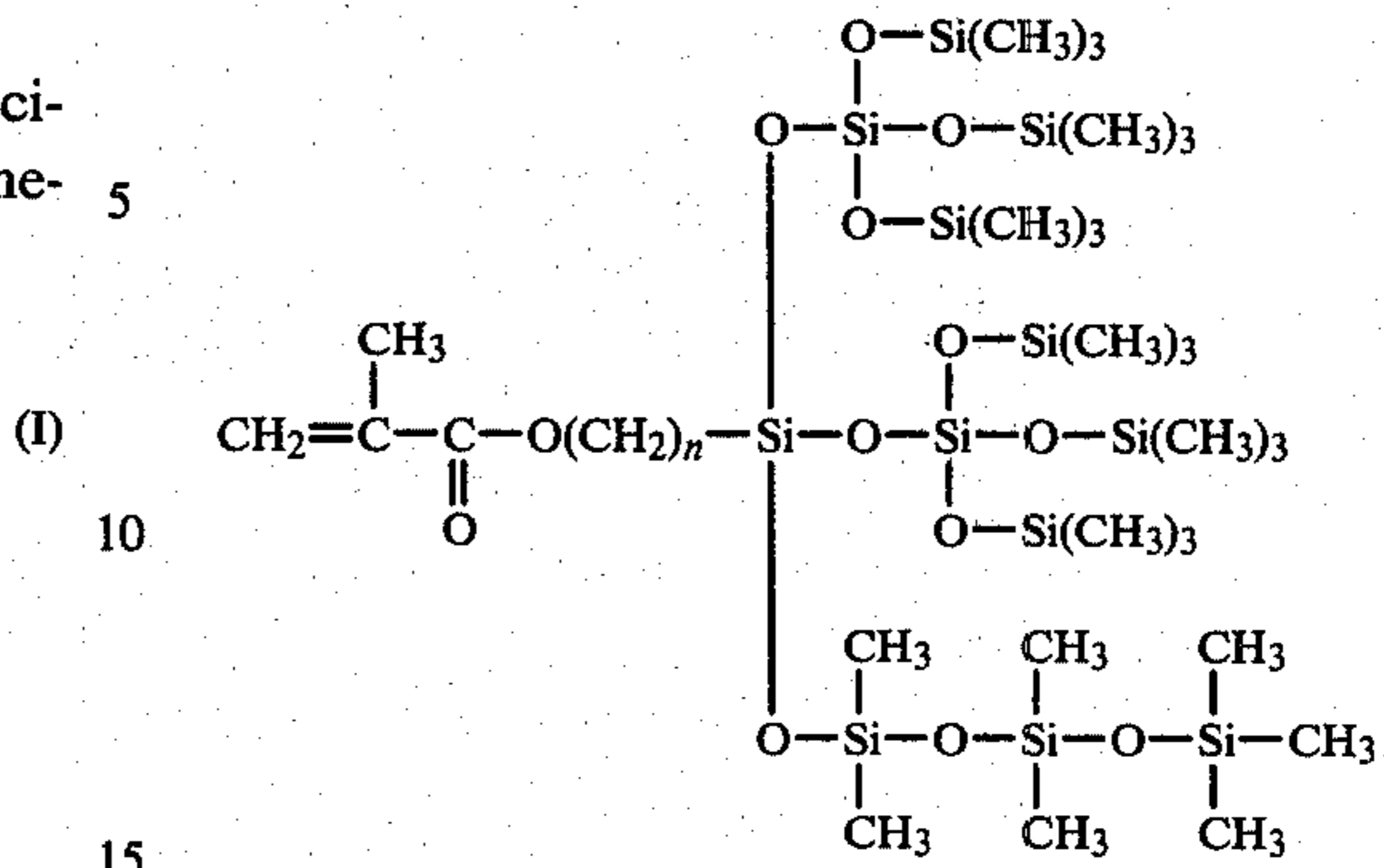
bis(tris-trimethylsiloxy-siloxanyl)mono(heptamethyl-trisiloxanyl)methacryloxyalkylsilane
