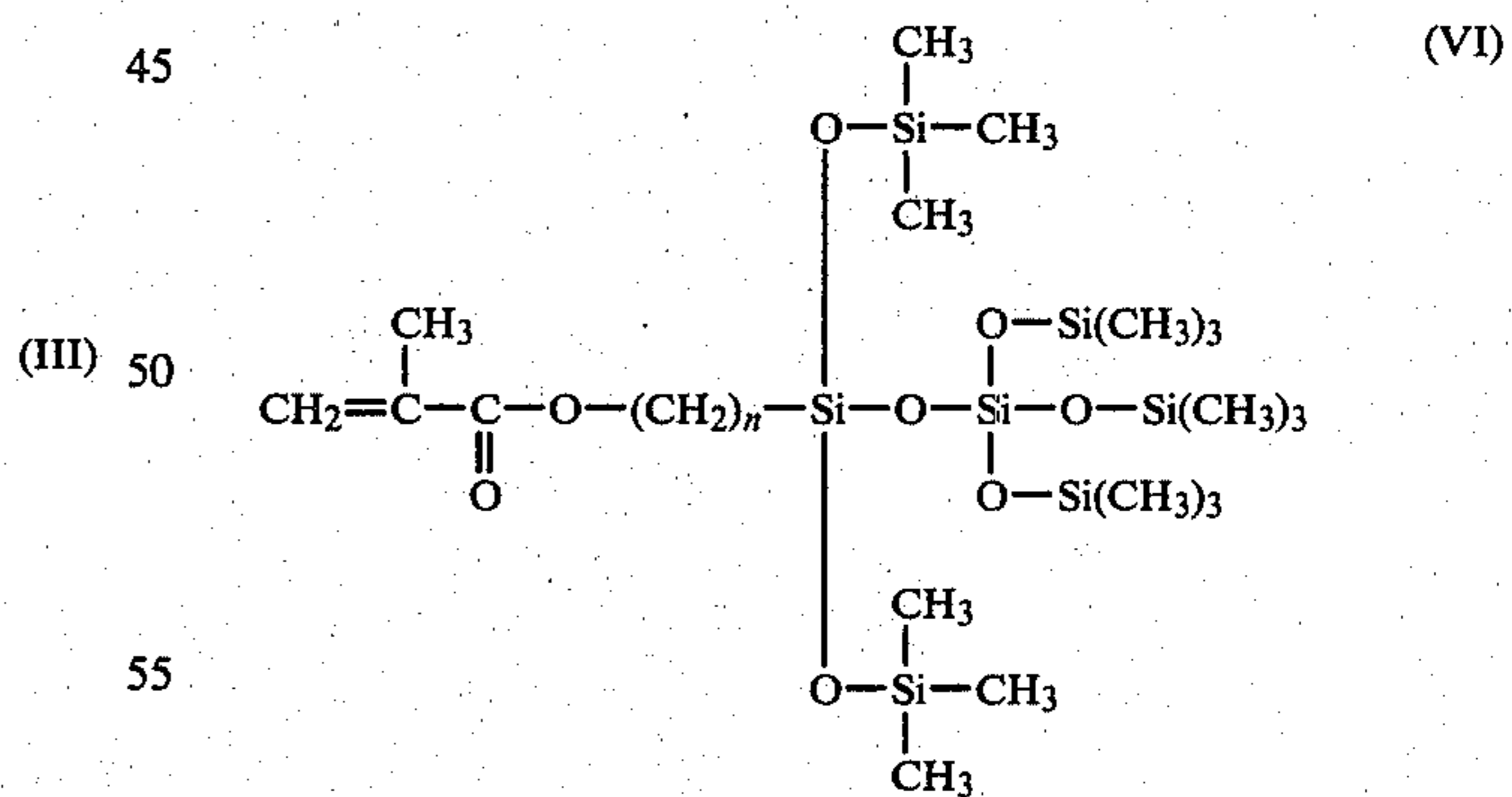
mono(tris-trimethylsiloxy-siloxanyl)bis(trimethylsiloxy)monopentamethyldisiloxanylmethacryloxyalkylsilane
