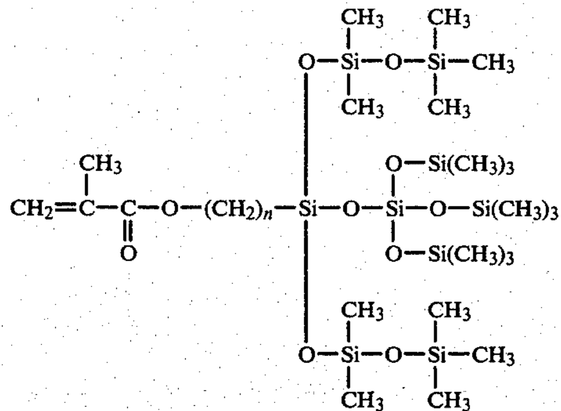
mono(tris-trimethylsiloxy-siloxanyl)bis(pentamethyldisiloxanyl)methacryloxyalkylsilane
