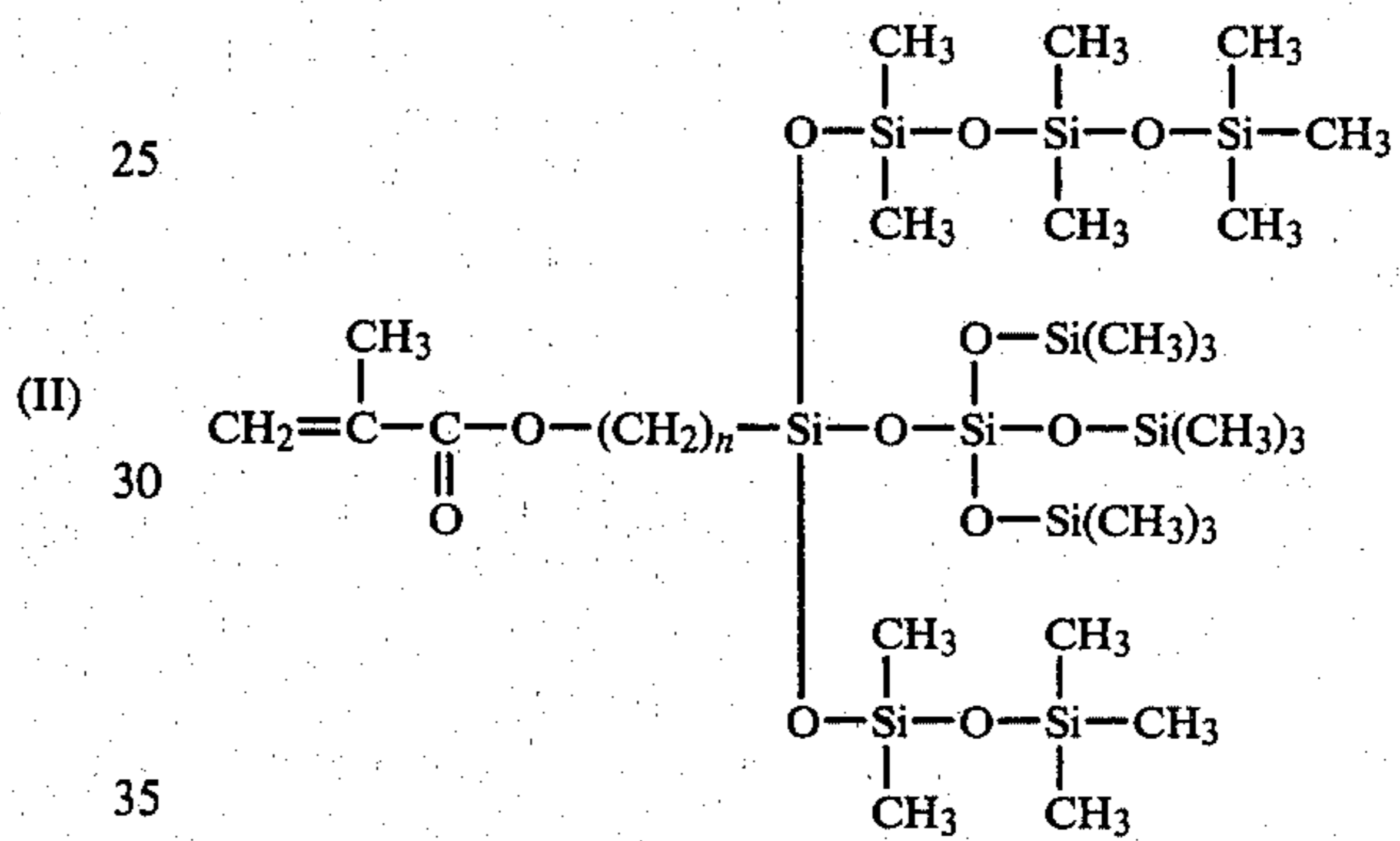
mono(tris-trimethylsiloxy-siloxanyl)mono(heptamethyl-trisiloxanyl)monopentamethyldisiloxanylemethacryloxyalkylsilane
