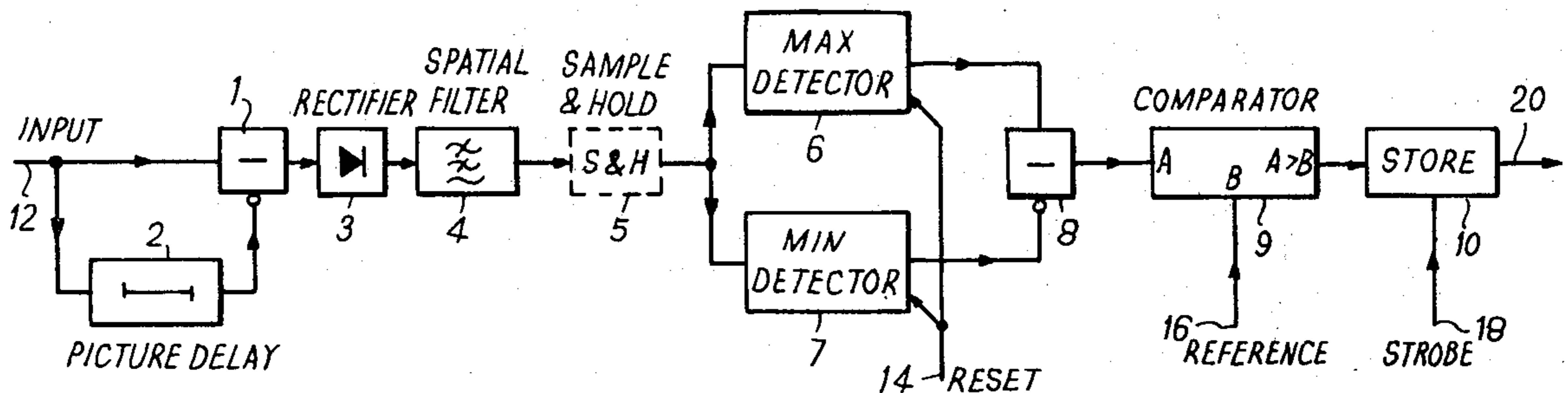
GENERAL REALISATION OF THE MOVEMENT DETECTOR
