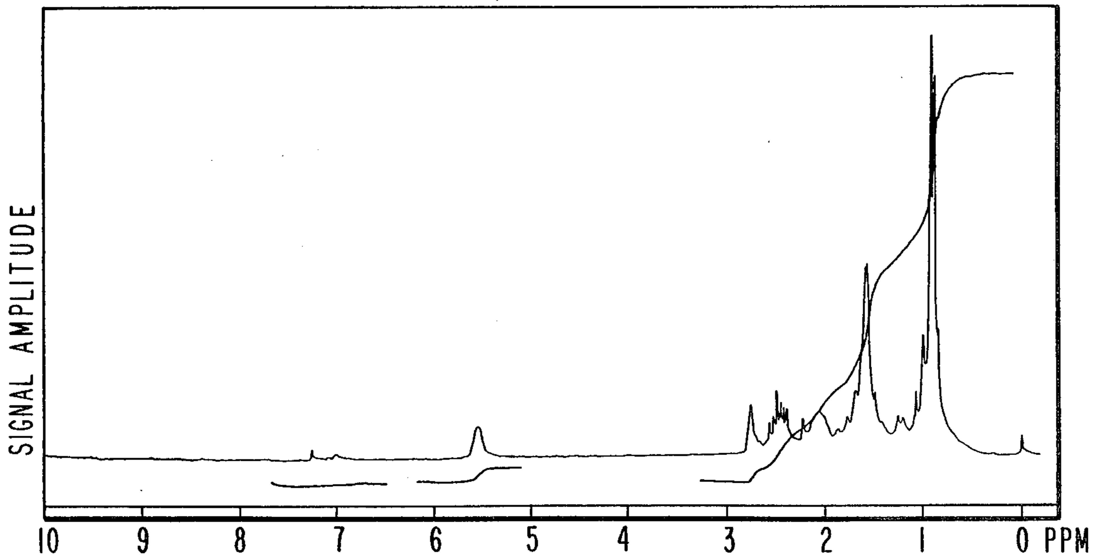
N M R SPECTRUM FOR EXAMPLE I, PEAK I .
