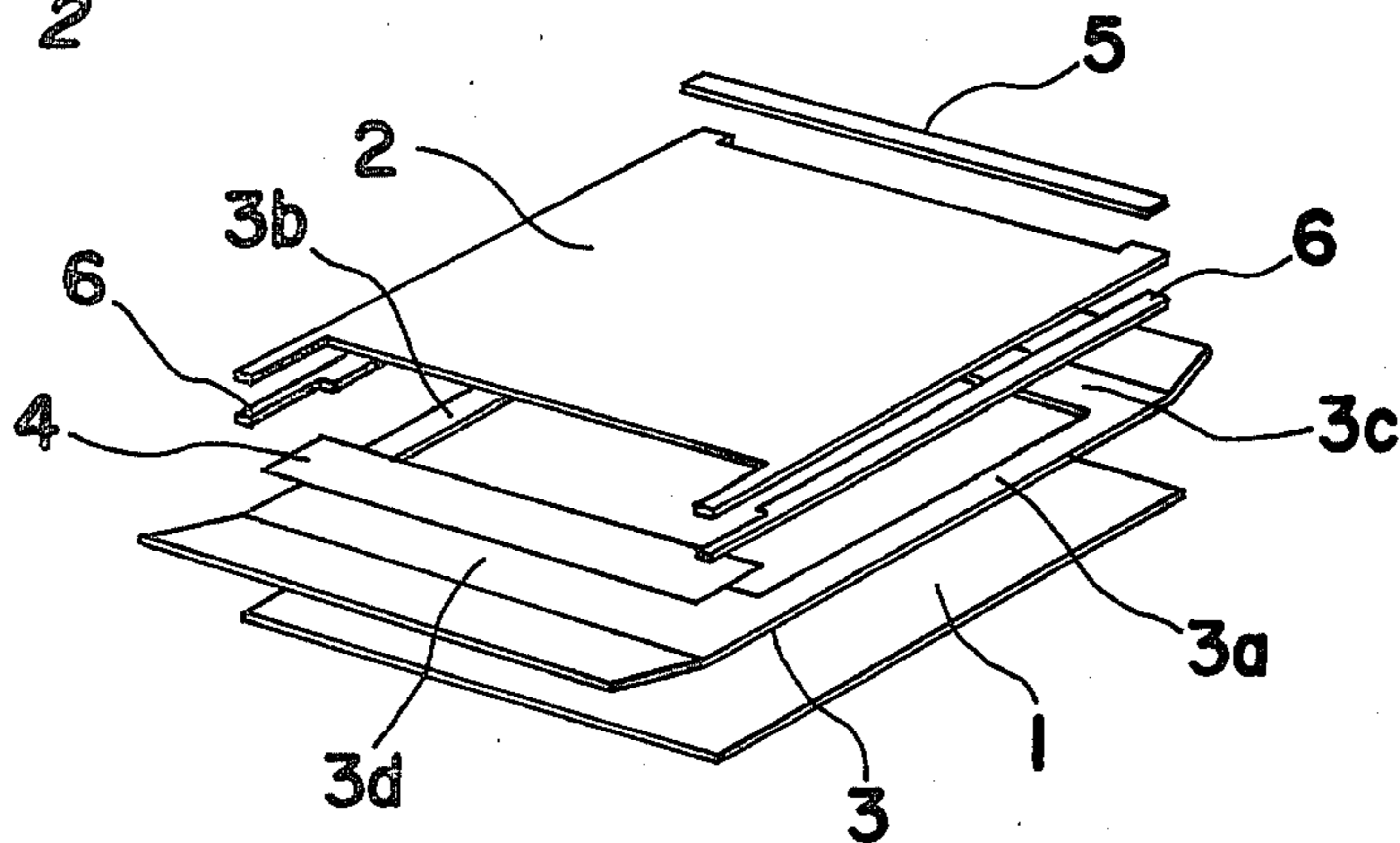
Fig. 3 (PRIOR ART)
