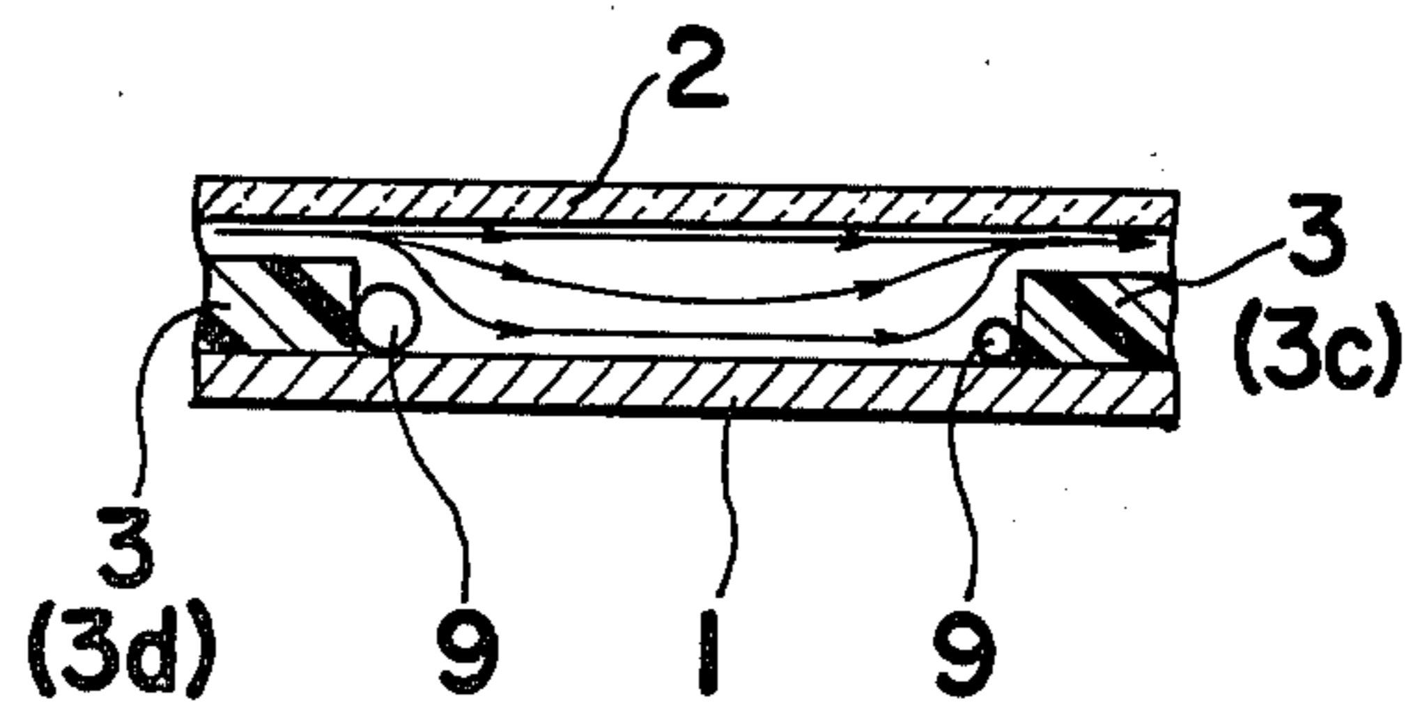
Fig. 5 (PRIOR ART)
