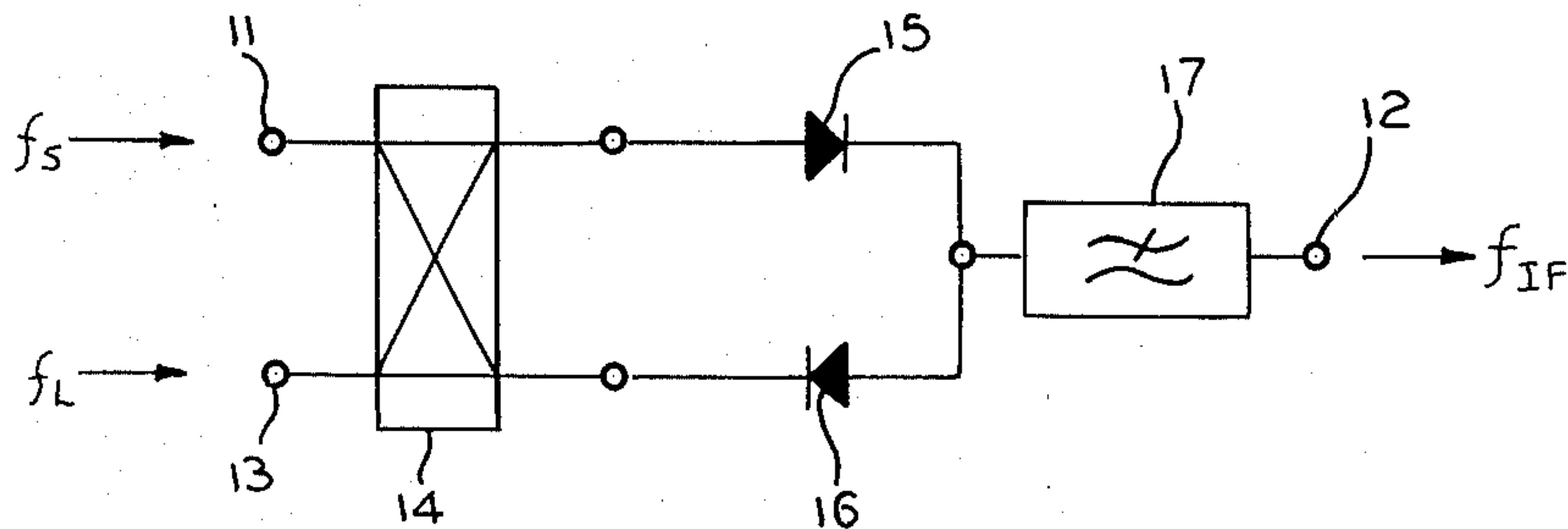
FIG. 3 (PRIOR ART)
