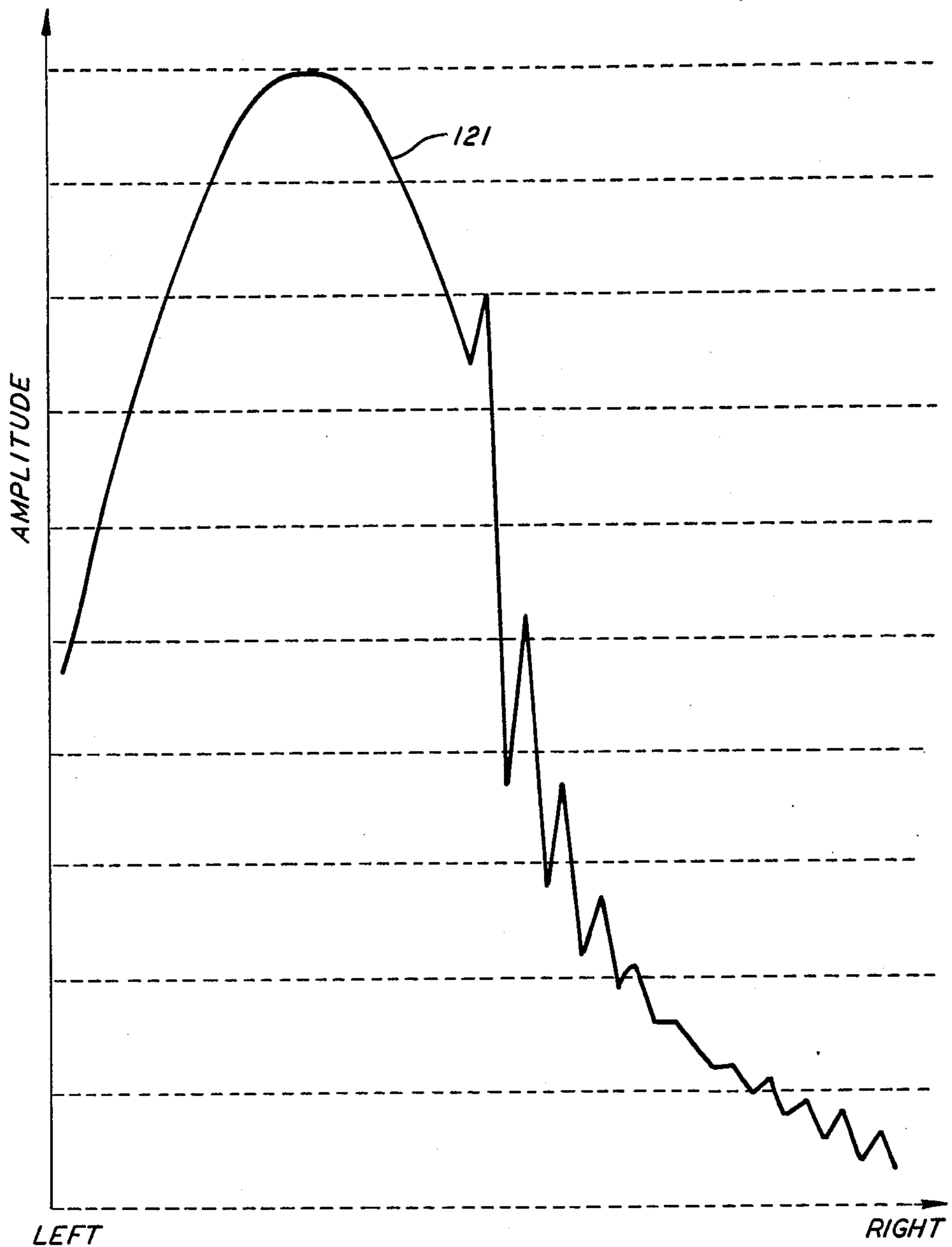
AMPLITUDE FUNCTION IN THE PLANE OF THE FEED ARRAY (SUMMED ALONG THE RADIATING ARRAYS), WHEN FED FROM LEFT (PORT A).
