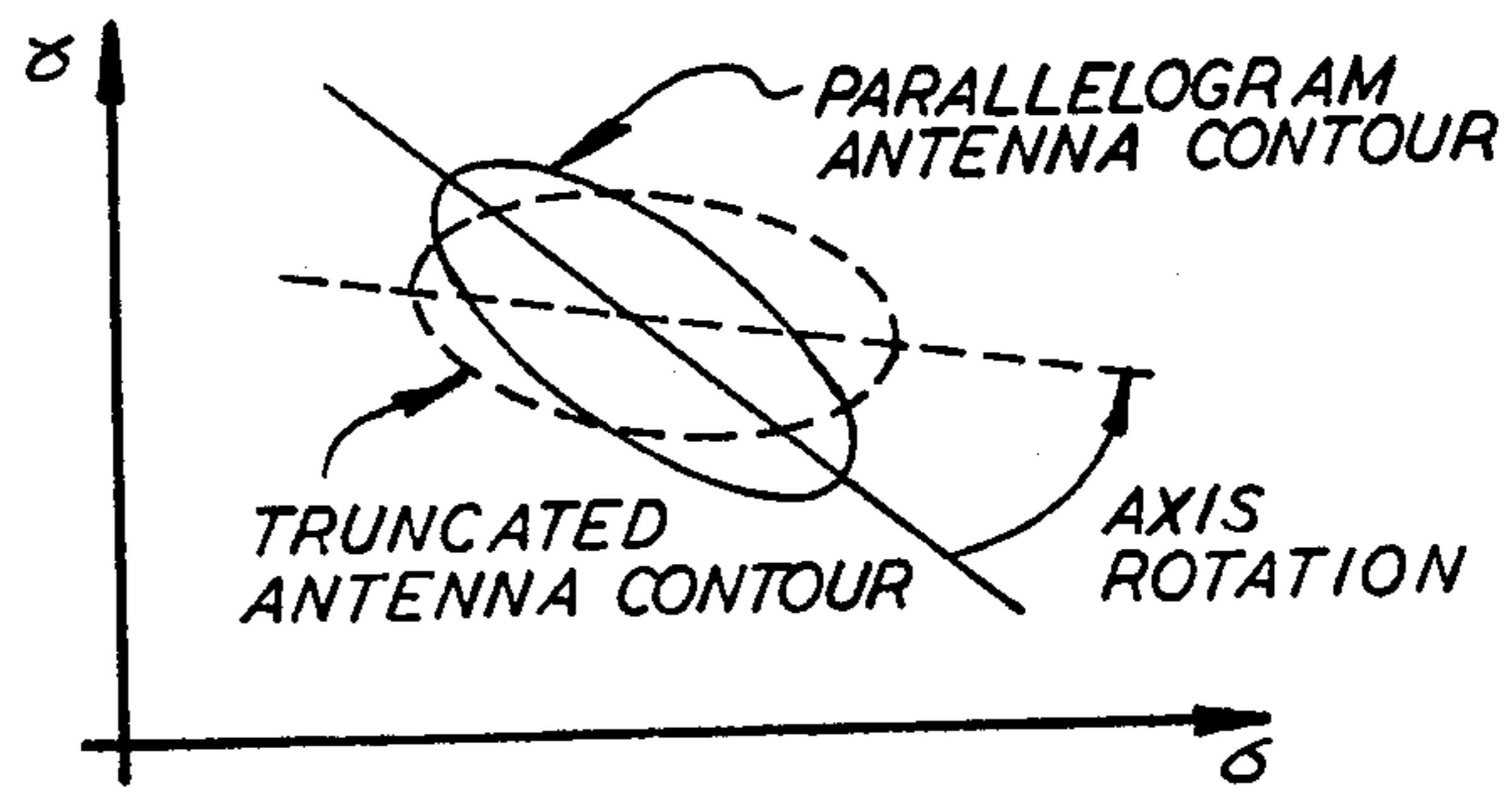
CONTOUR ROTATION EFFECTS RESULTING FROM APERTURE TRUNCATION
