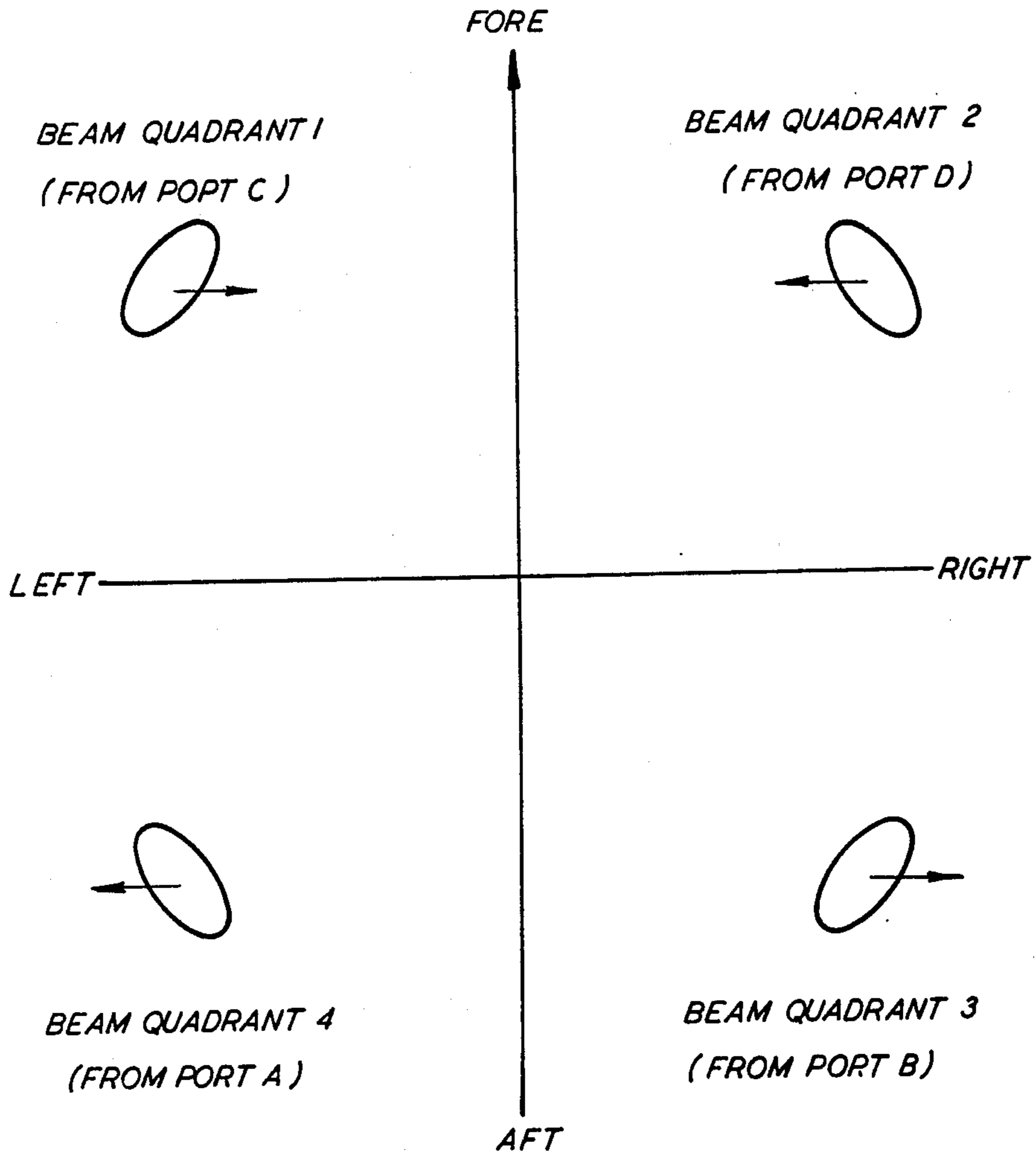
BEAM GROUND FOOTPRINT SHOWING DIRECTION OF MOTION WITH INCREASING FREQUENCY
