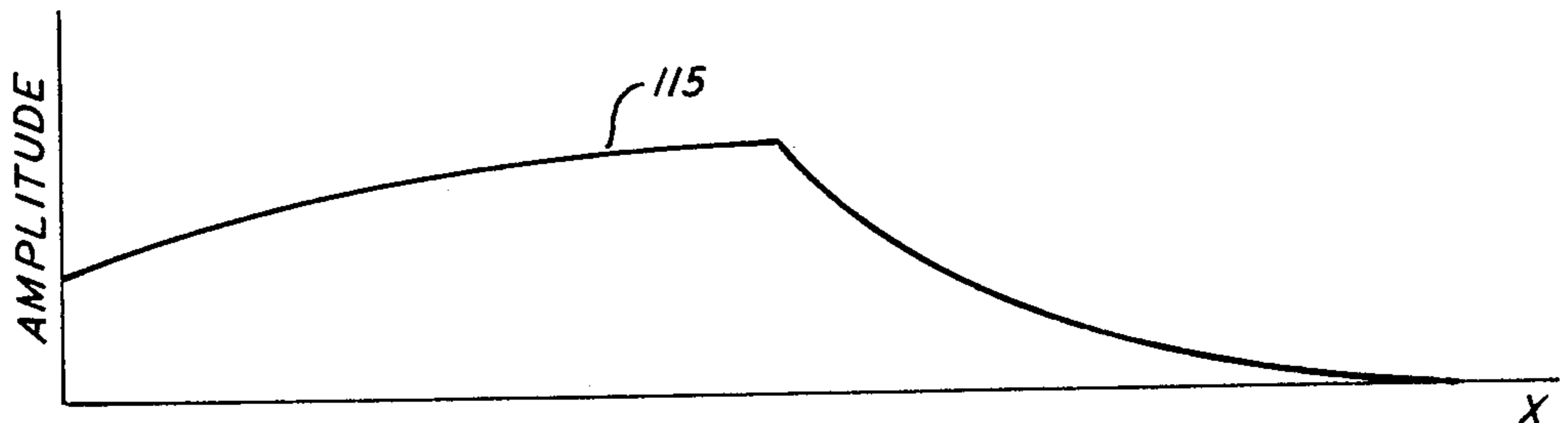
FORWARD FIRING ARRAY FED FROM LEFT FIG. 16a
