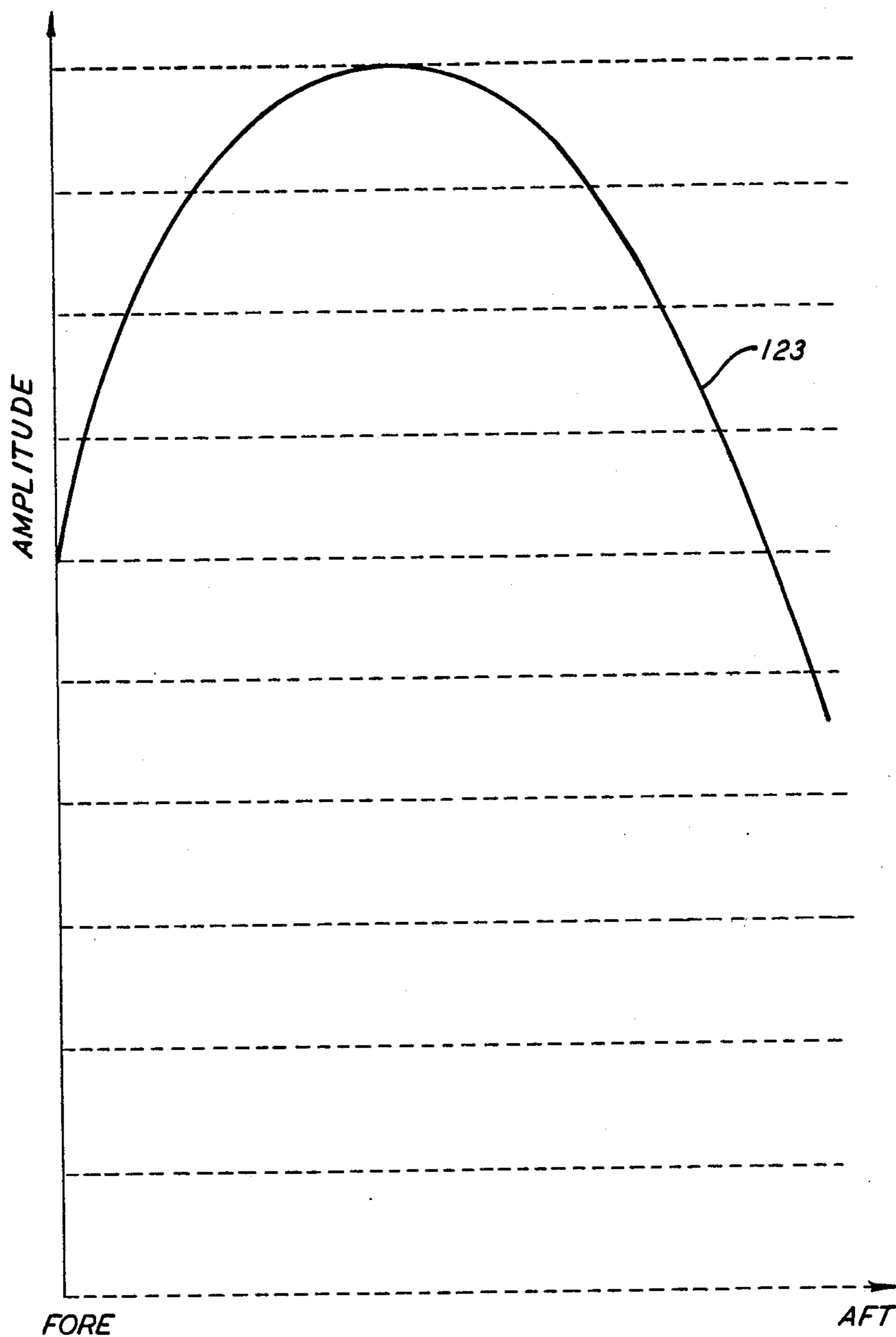
AMPLITUDE FUNCTION IN THE PLANE OF THE RADIATING ARRAYS, (SUMMED ACROSS THE APERTURE), WHEN FED FROM TOP (PORT A).
