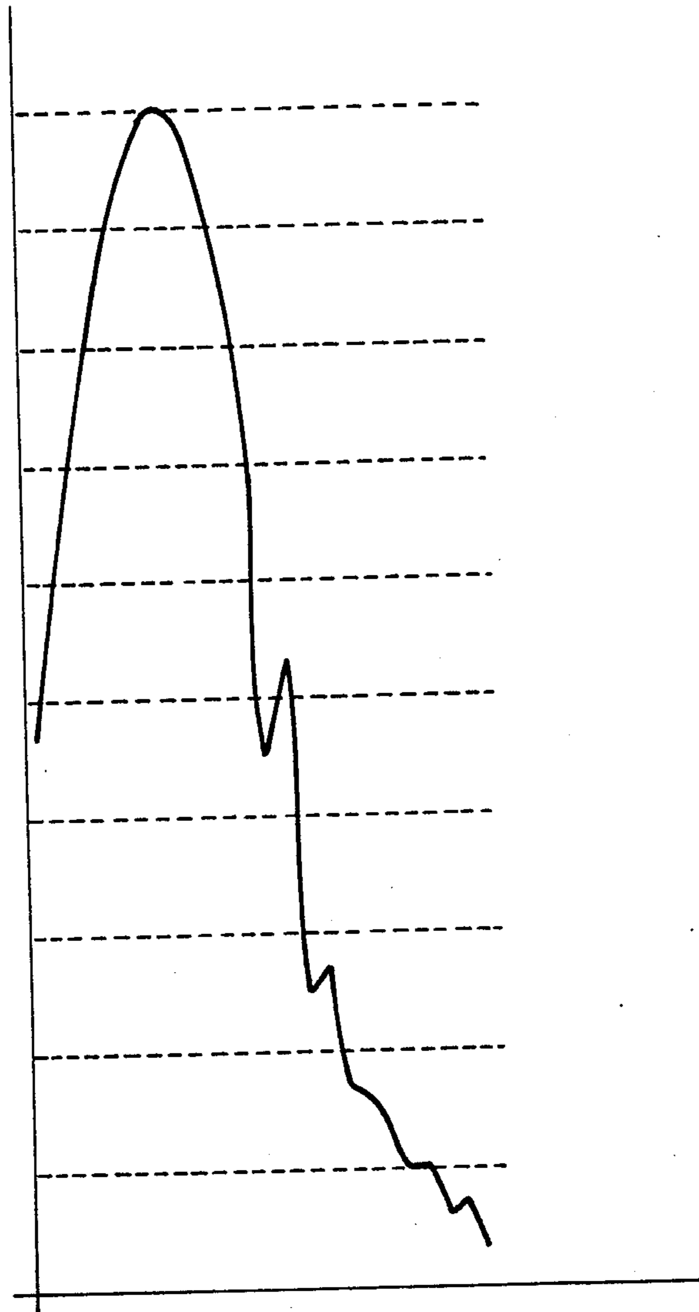
AMPLITUDE FUNCTION IN THE PLANE OF THE FEED ARRAY (SUMMED ALONG THE RADIATING ARRAYS), WHEN FED FROM LEFT (PORT A OR E)
