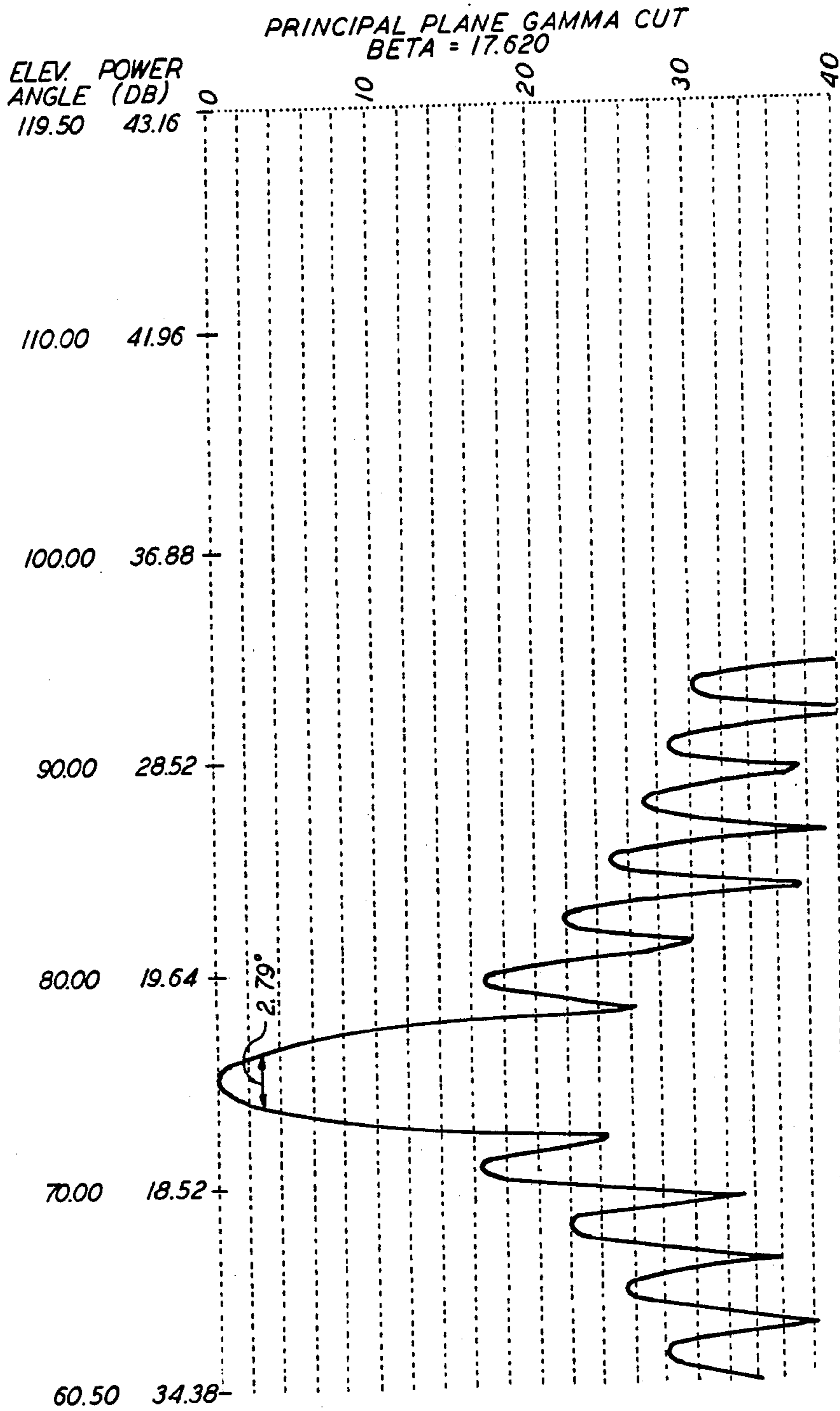
PRINCIPAL GAMMA PLANE FAR FIELD PATTERN
