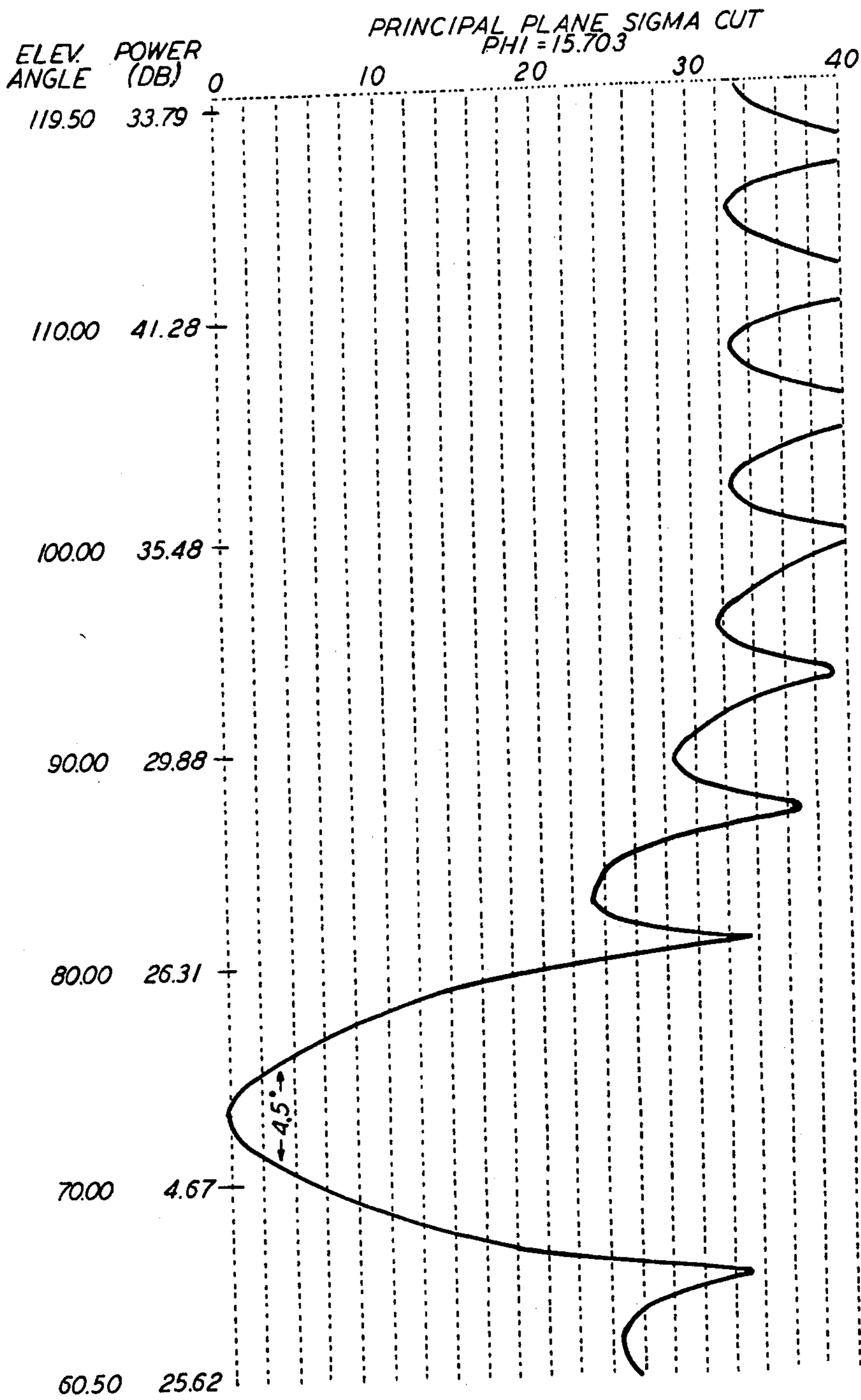
PRINCIPAL SIGMA PLANE FAR FIELD PATTERN
