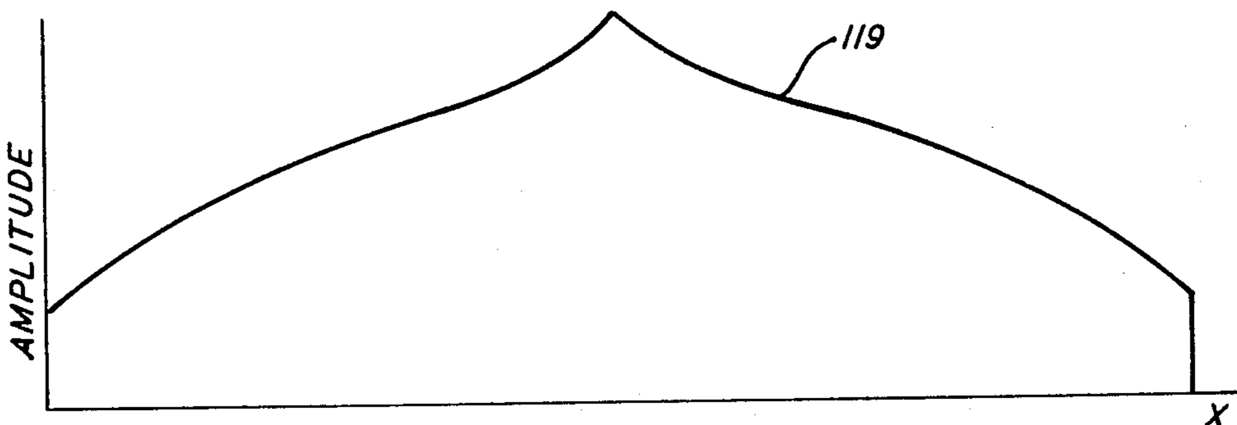
COMBINED AMPLITUDE FUNCTION FROM a & b FIG. 16c
