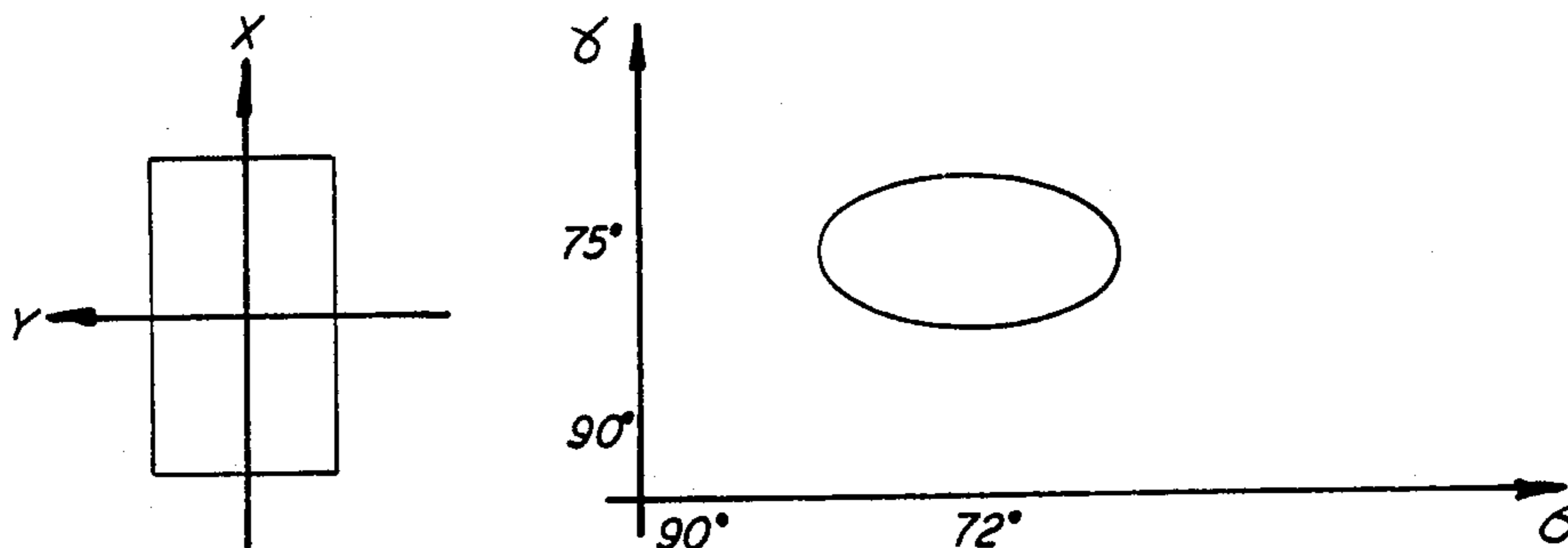
RECTANGULAR APERTURE PATTERN IN A GAMMA-SIGMA COORDINATE SYSTEM FIG. 5a
