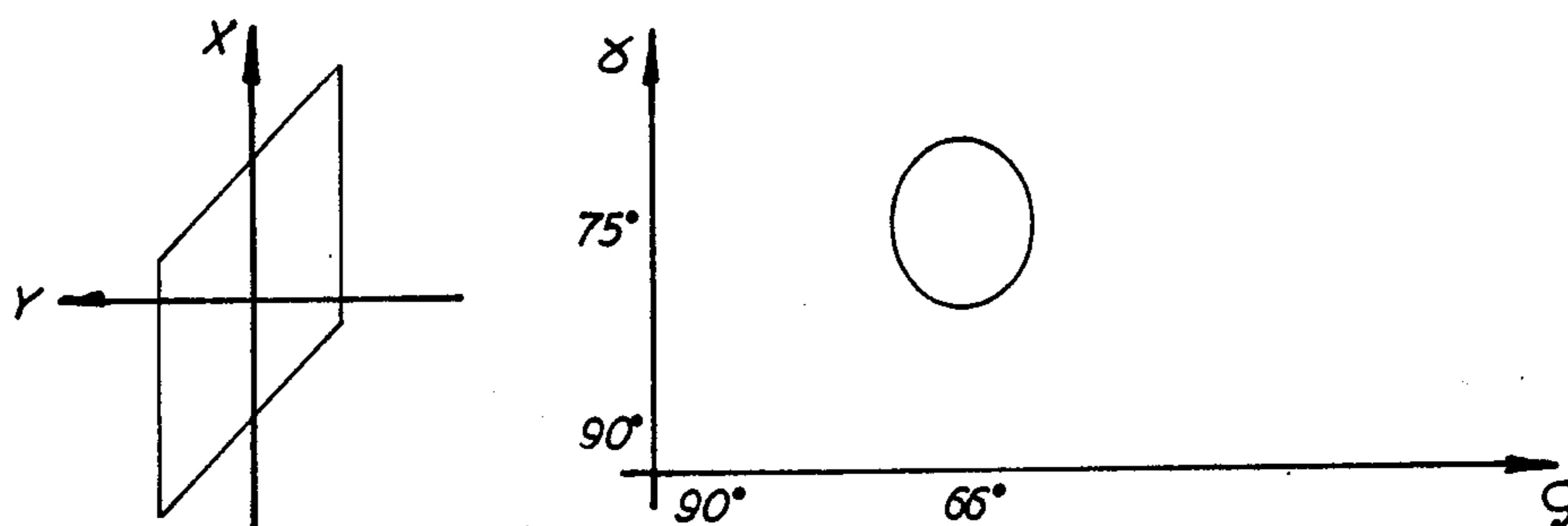
SLANTED APERTURE PATTERN IN A GAMMA-ZETA COORDINATE SYSTEM FIG. 5b
