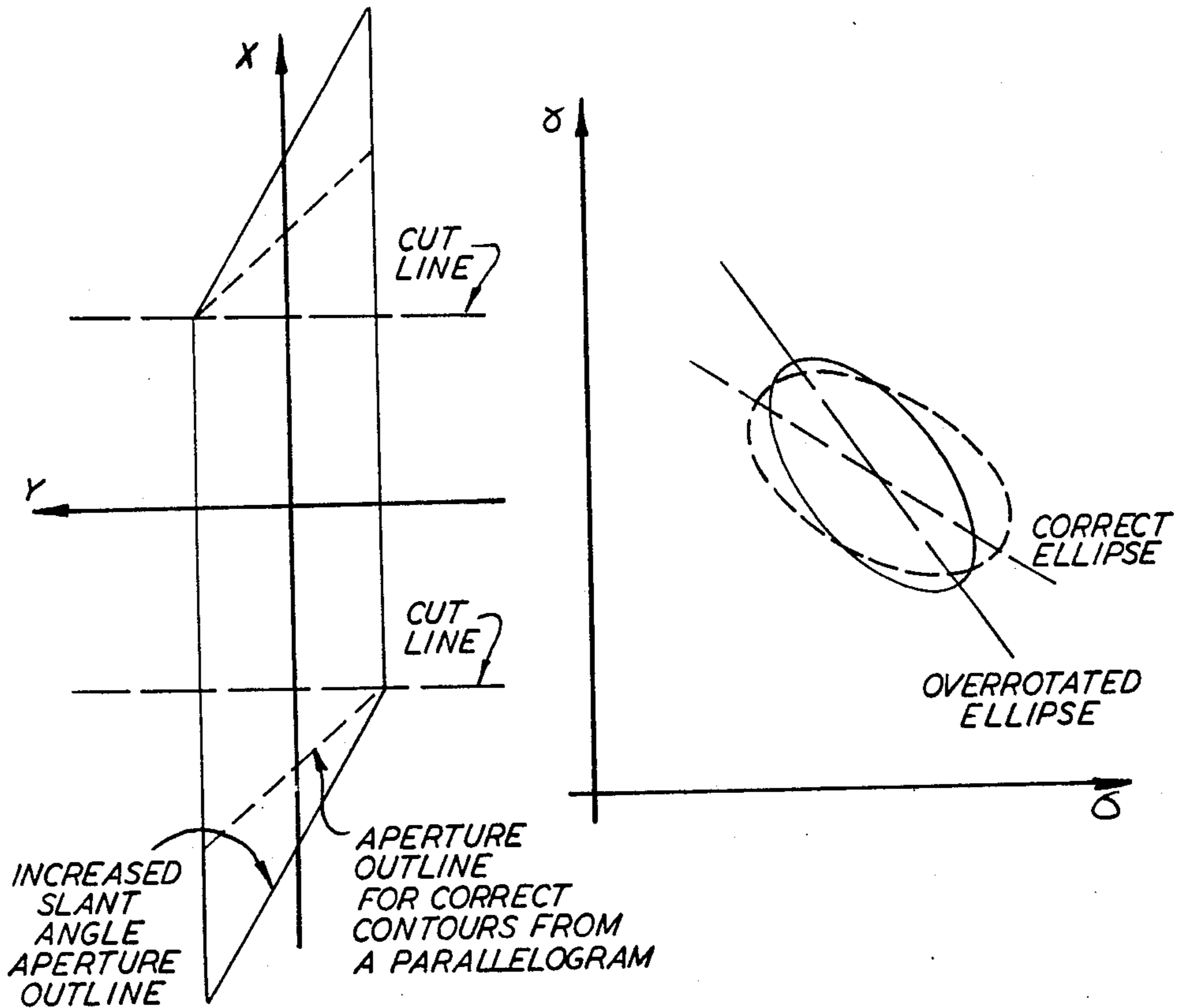
OVERROTATION OF CONTOUR-ELLIPSE AXIS BY A LARGE SLANT ANGLE
