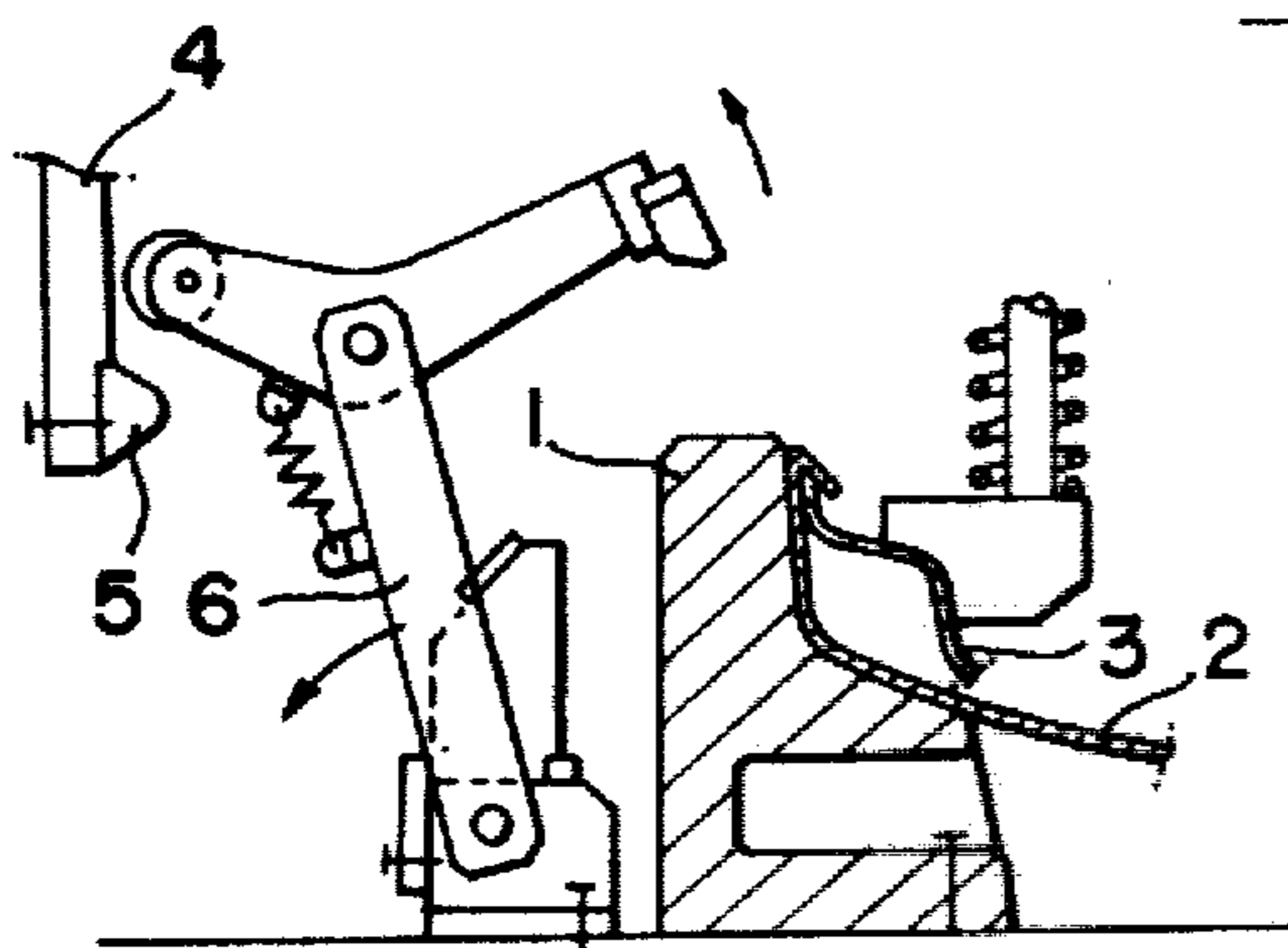
FIG. 3 PRIOR ART
