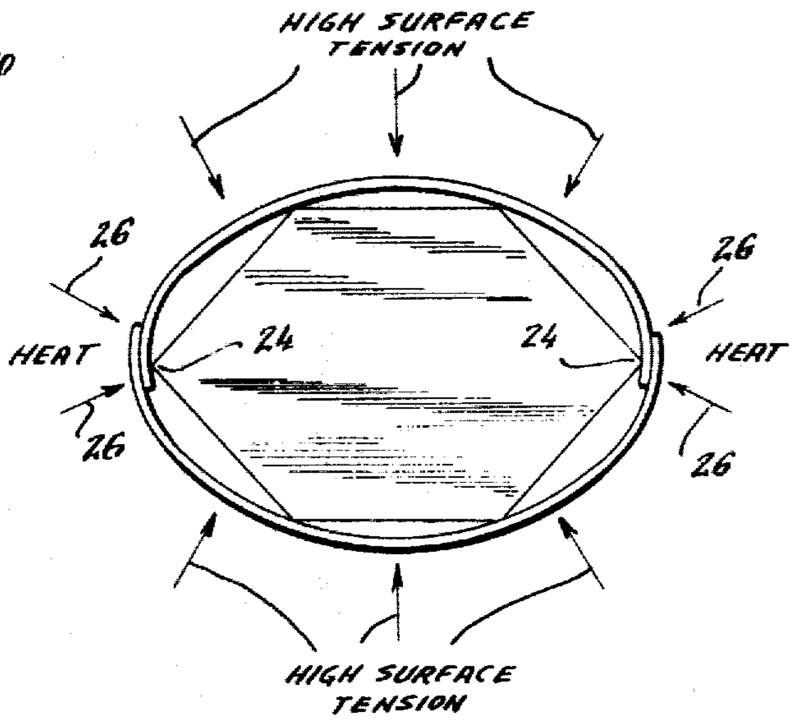
Fig. 2. (PRIOR ART)
