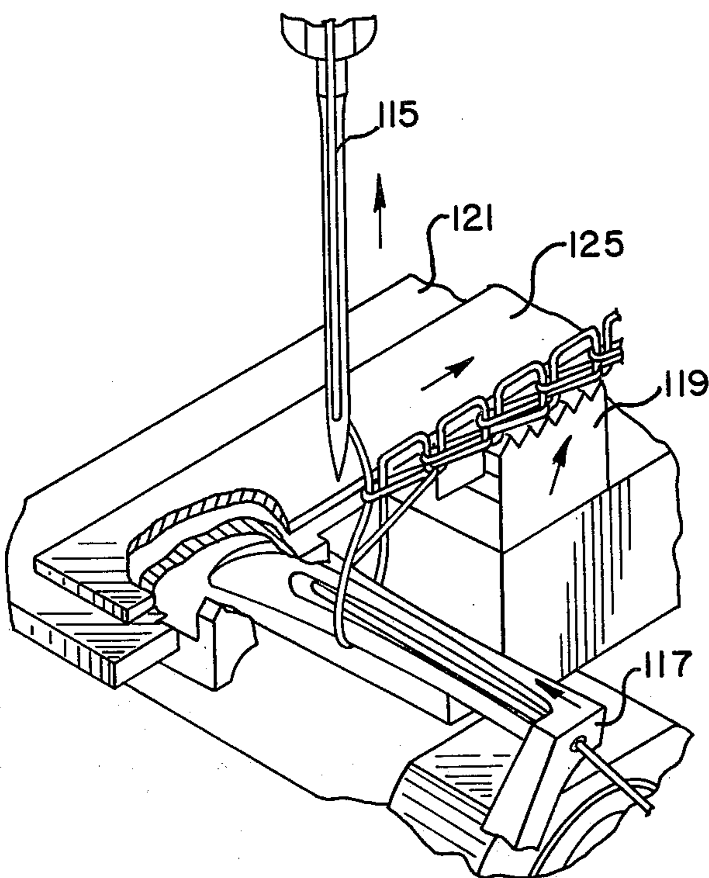
FIG 12 PRIOR ART
