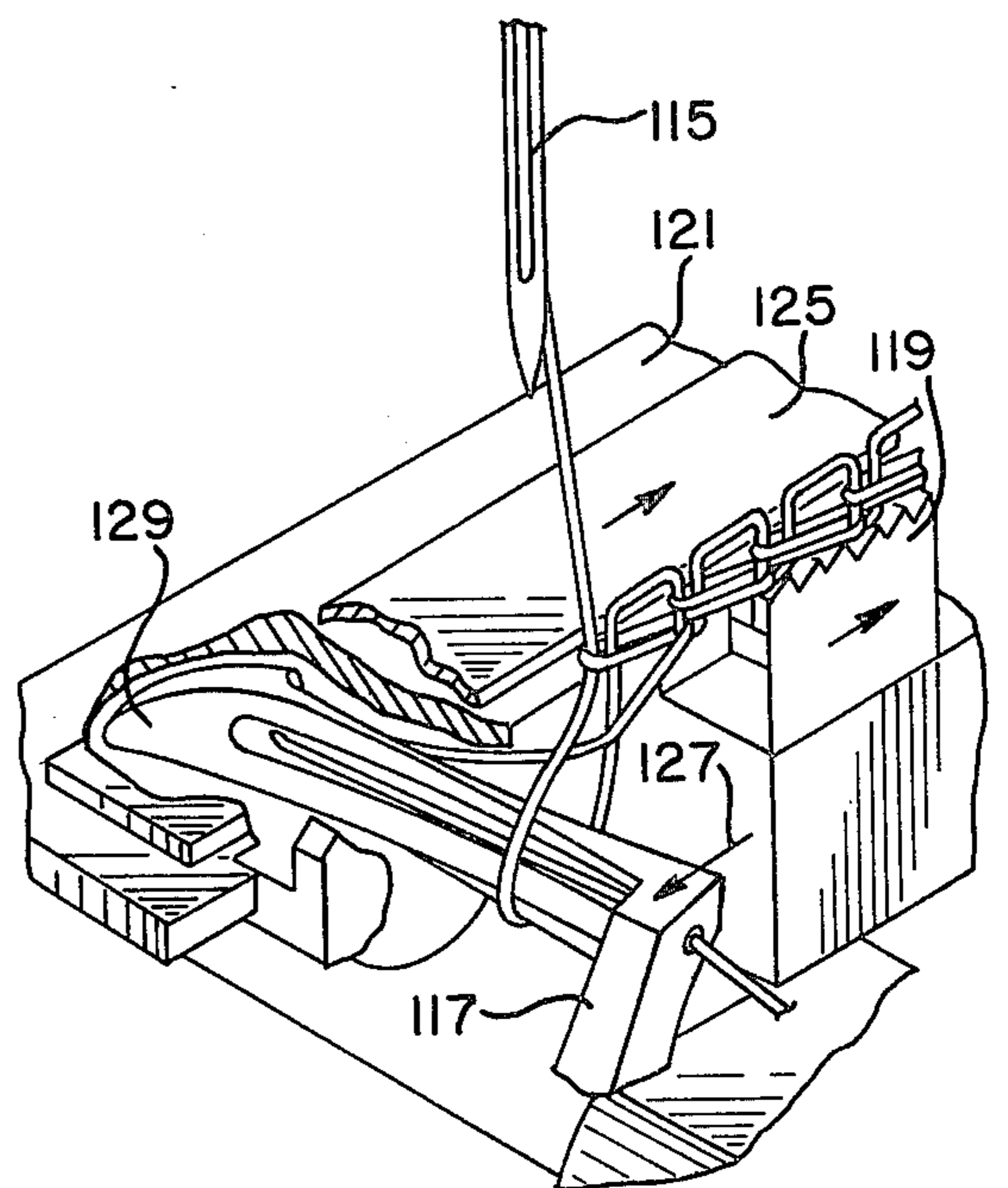
FIG 13 PRIOR ART
