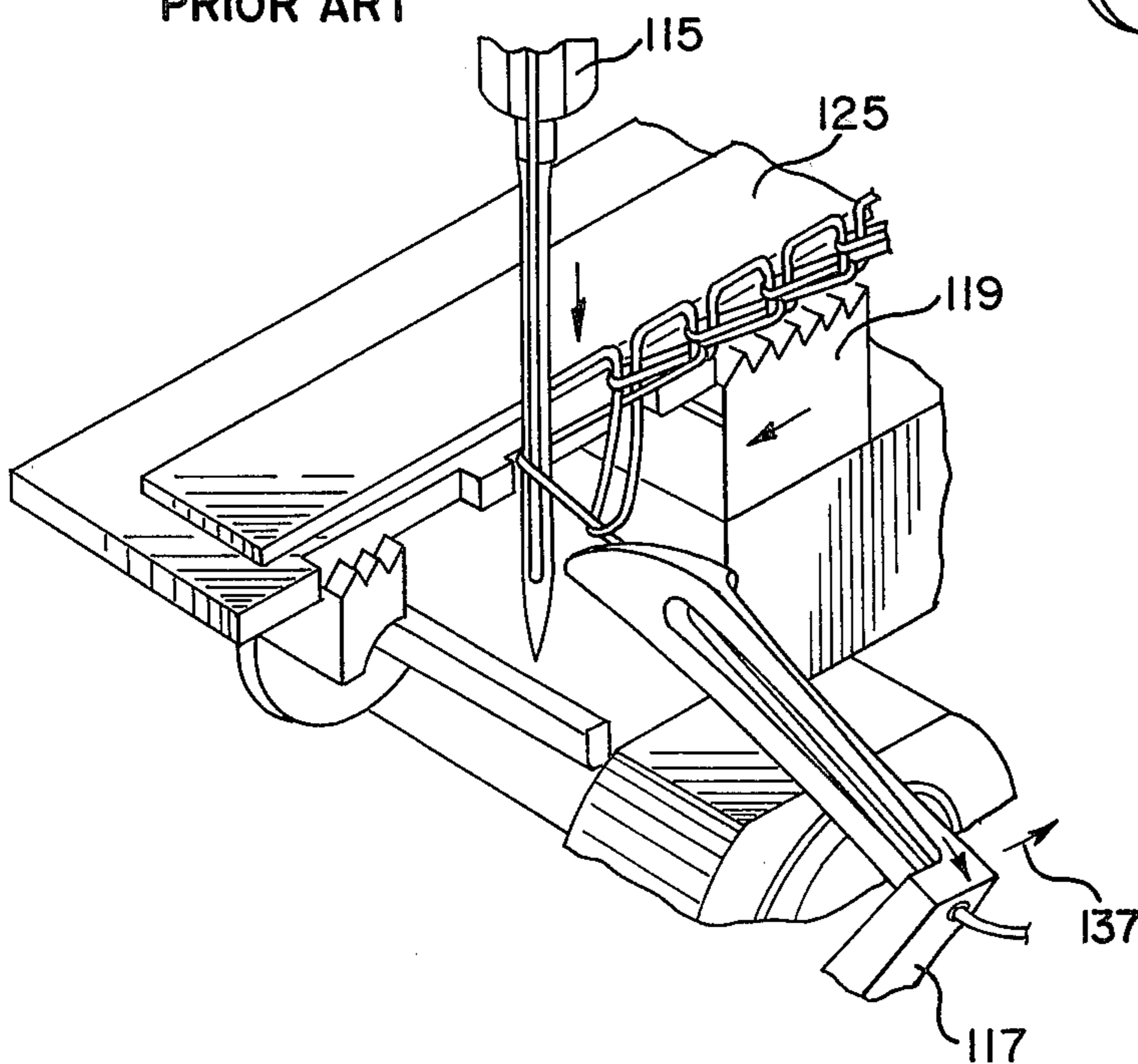
FIG. 16 PRIOR ART
