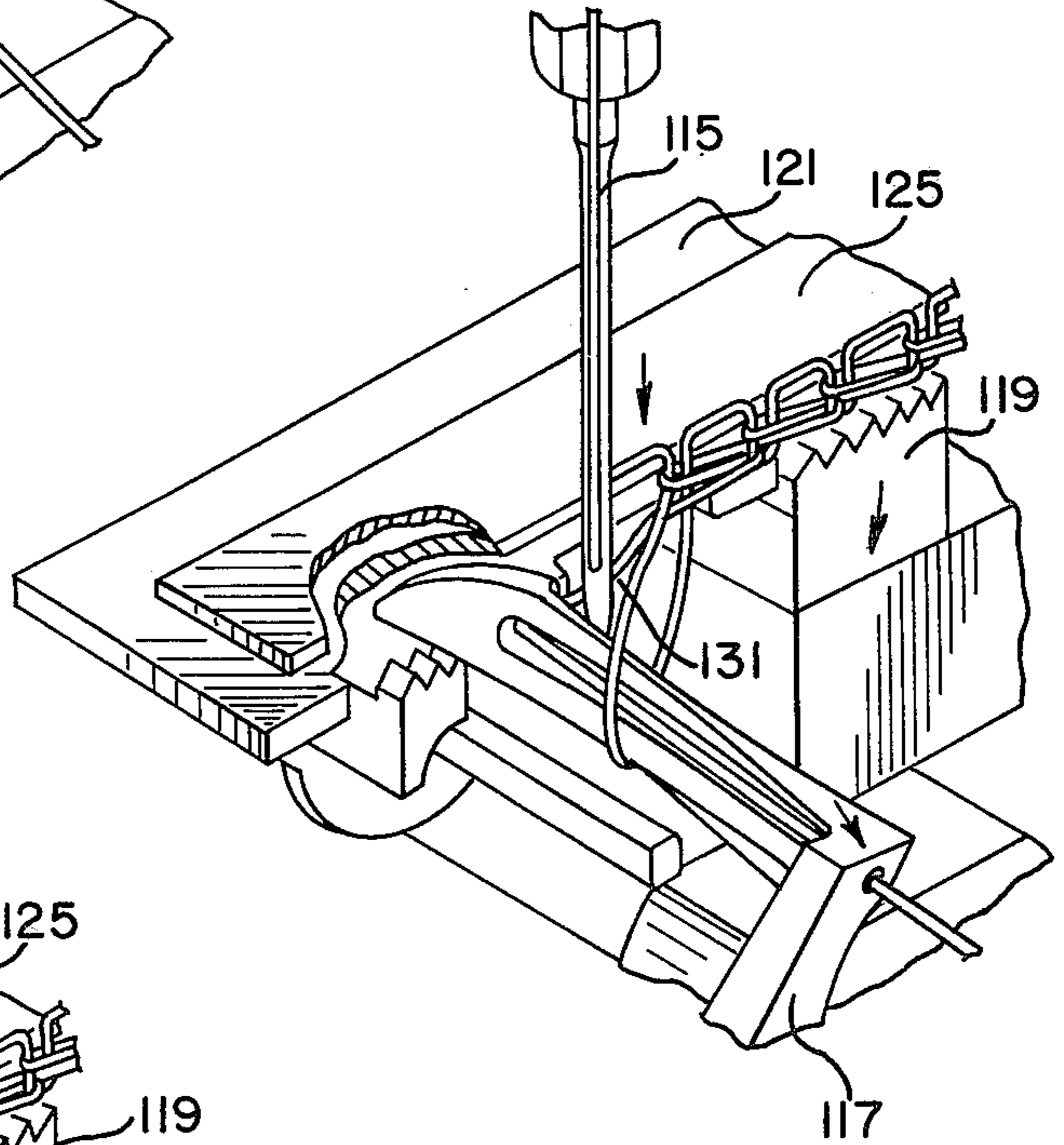
FIG. 15 PRIOR ART
