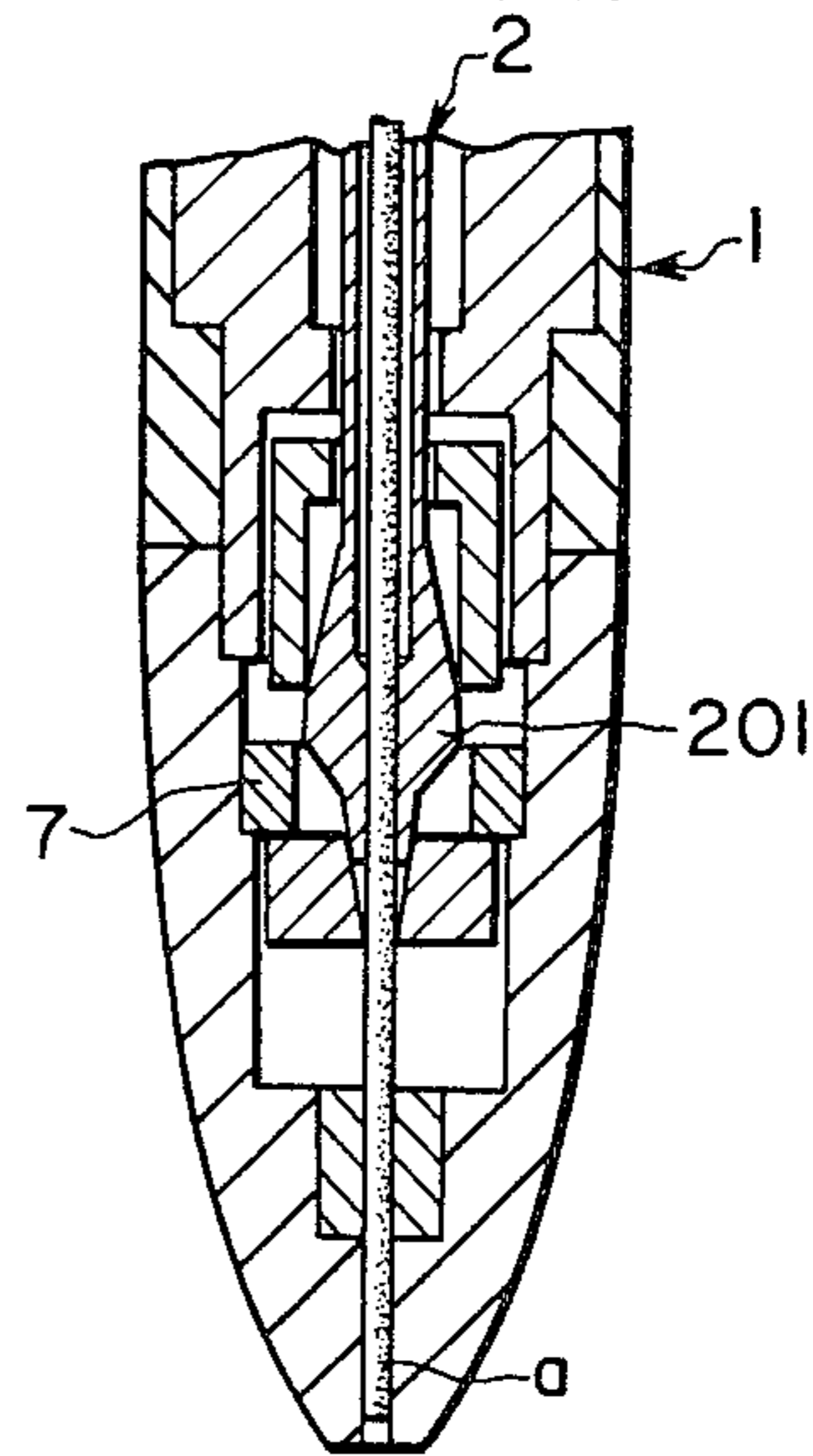
FIG. 17 PRIOR ART
