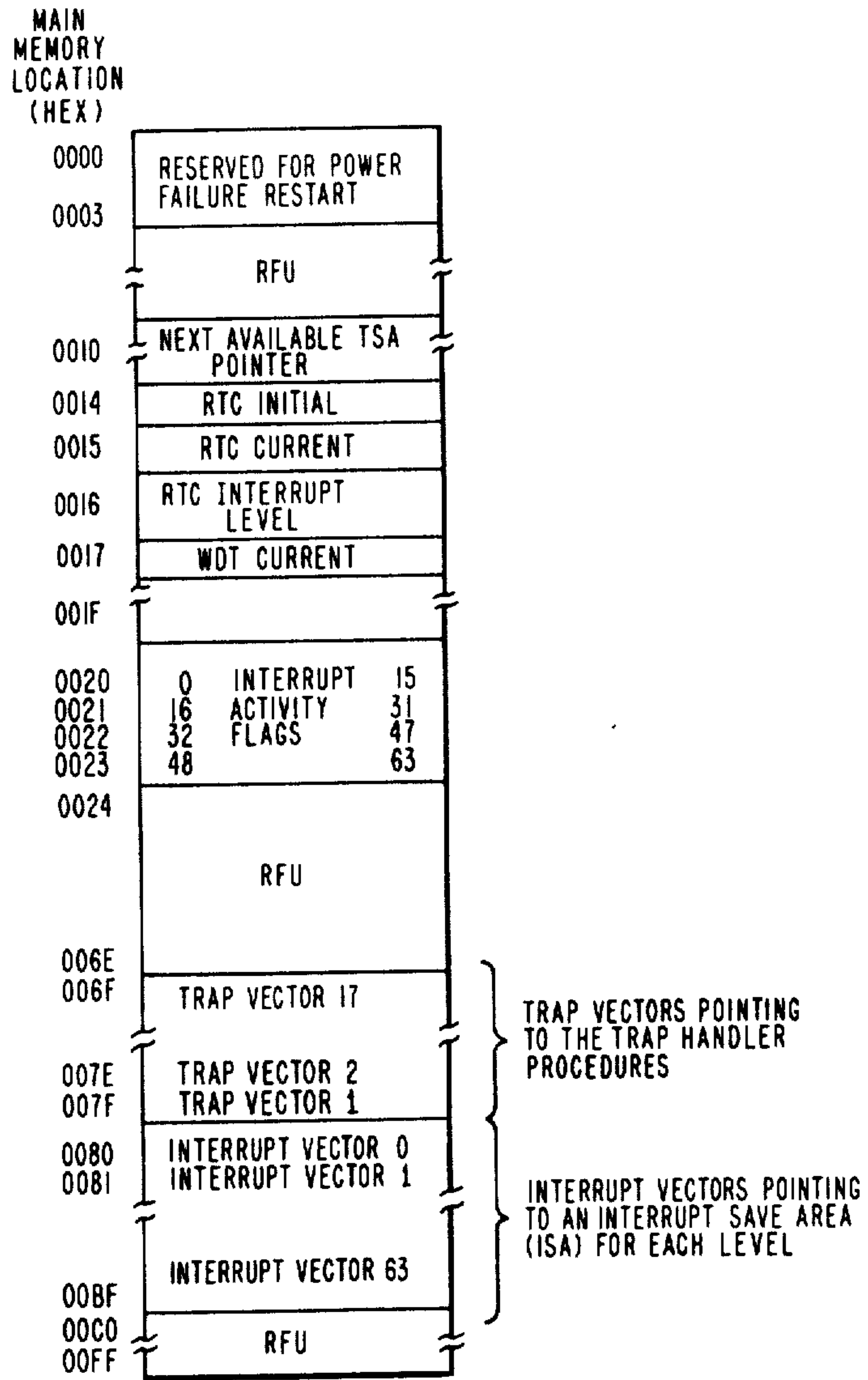
DEDICATED MAIN MEMORY LOCATIONS
