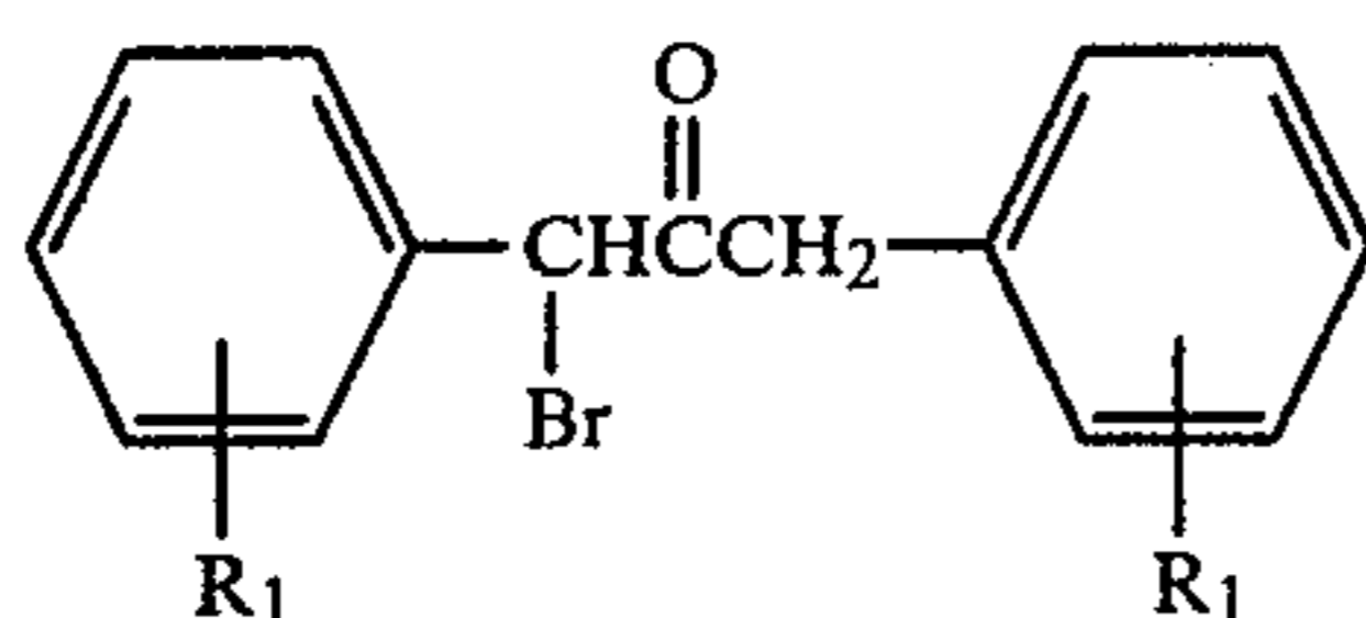
1,3-Diaryl-2-propanone
