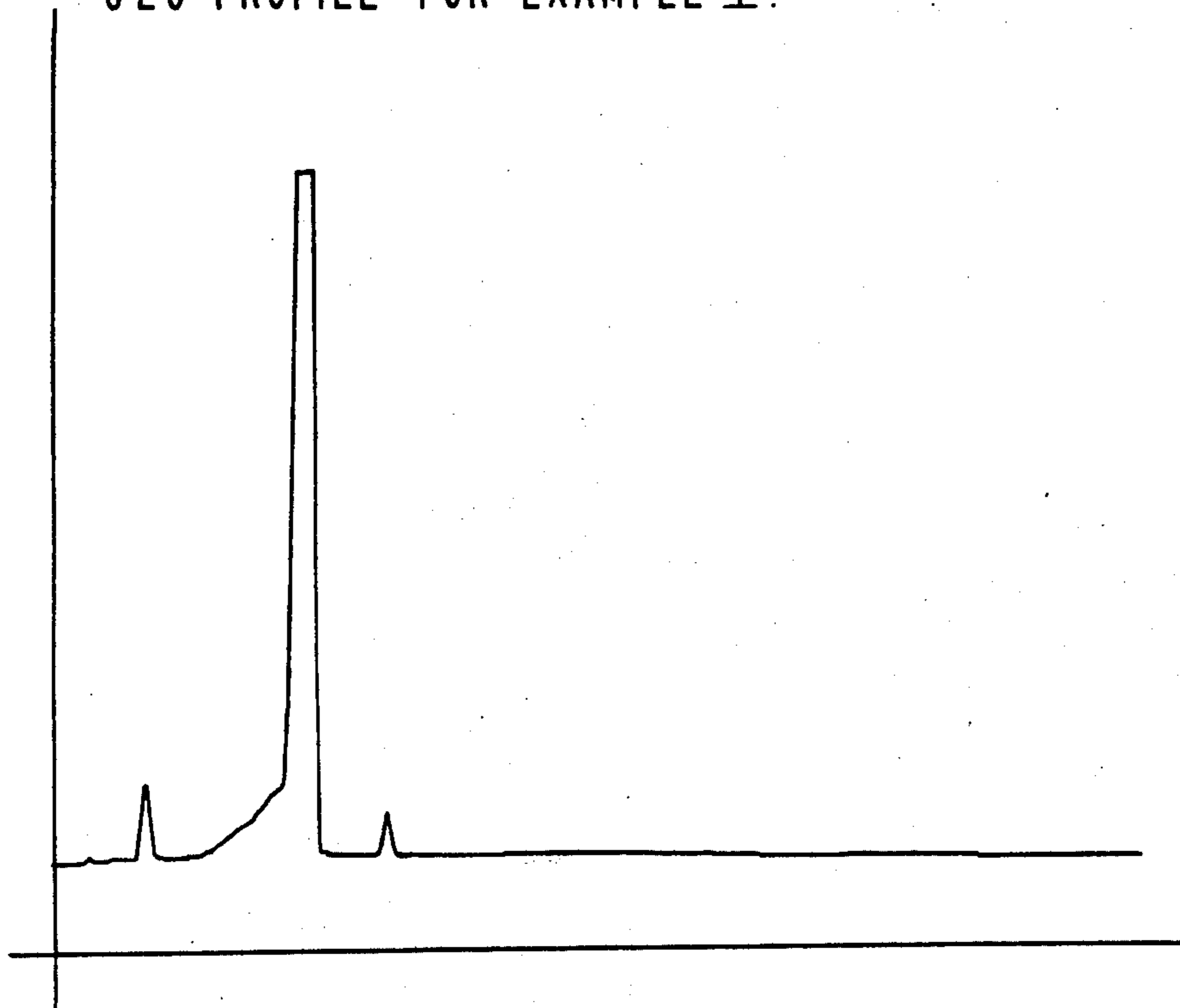
GLC PROFILE FOR EXAMPLE I.
