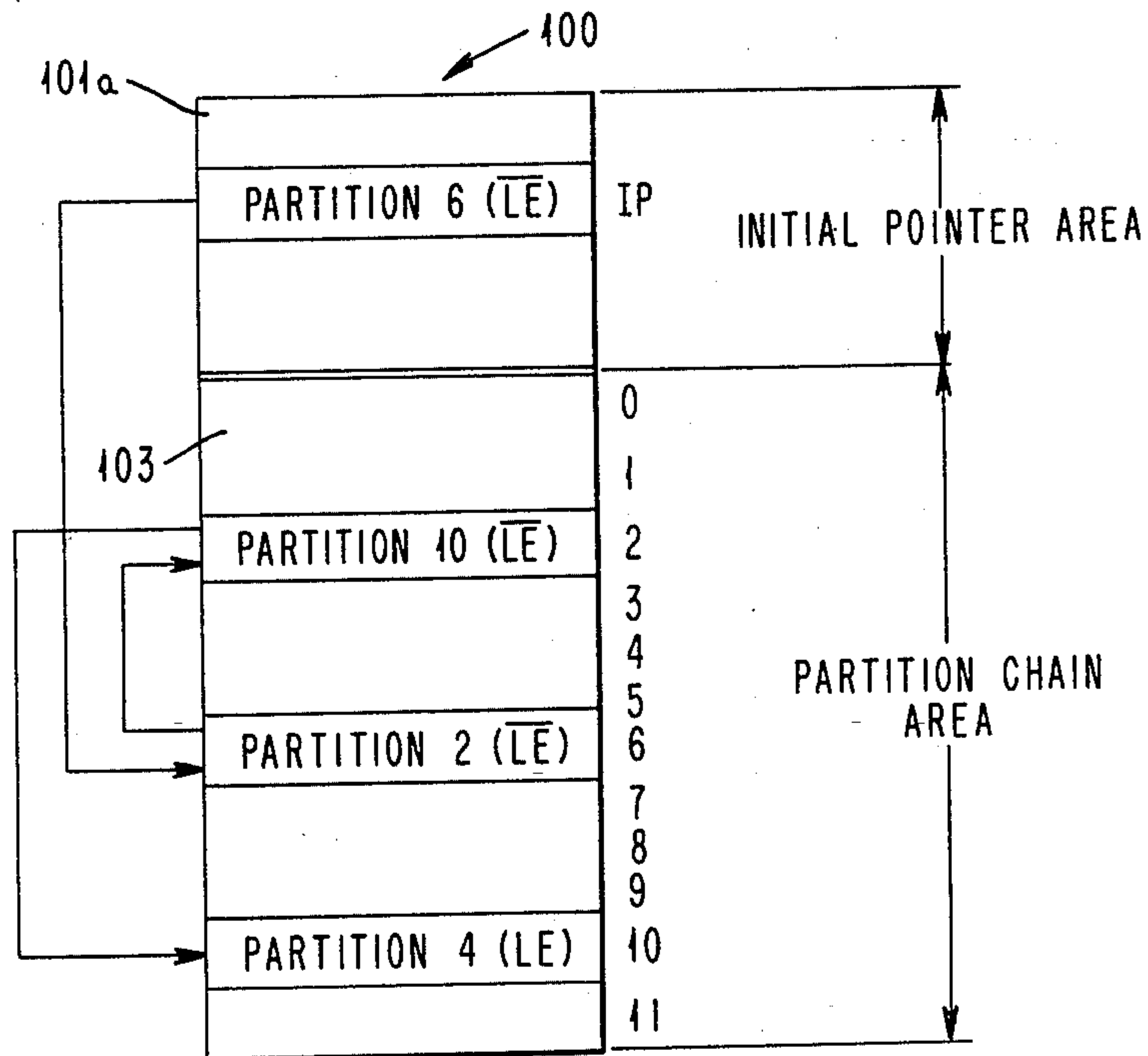
FIG. 46 TRANSMIT LIST STRUCTURE IN BURST PRIORITY RAM
