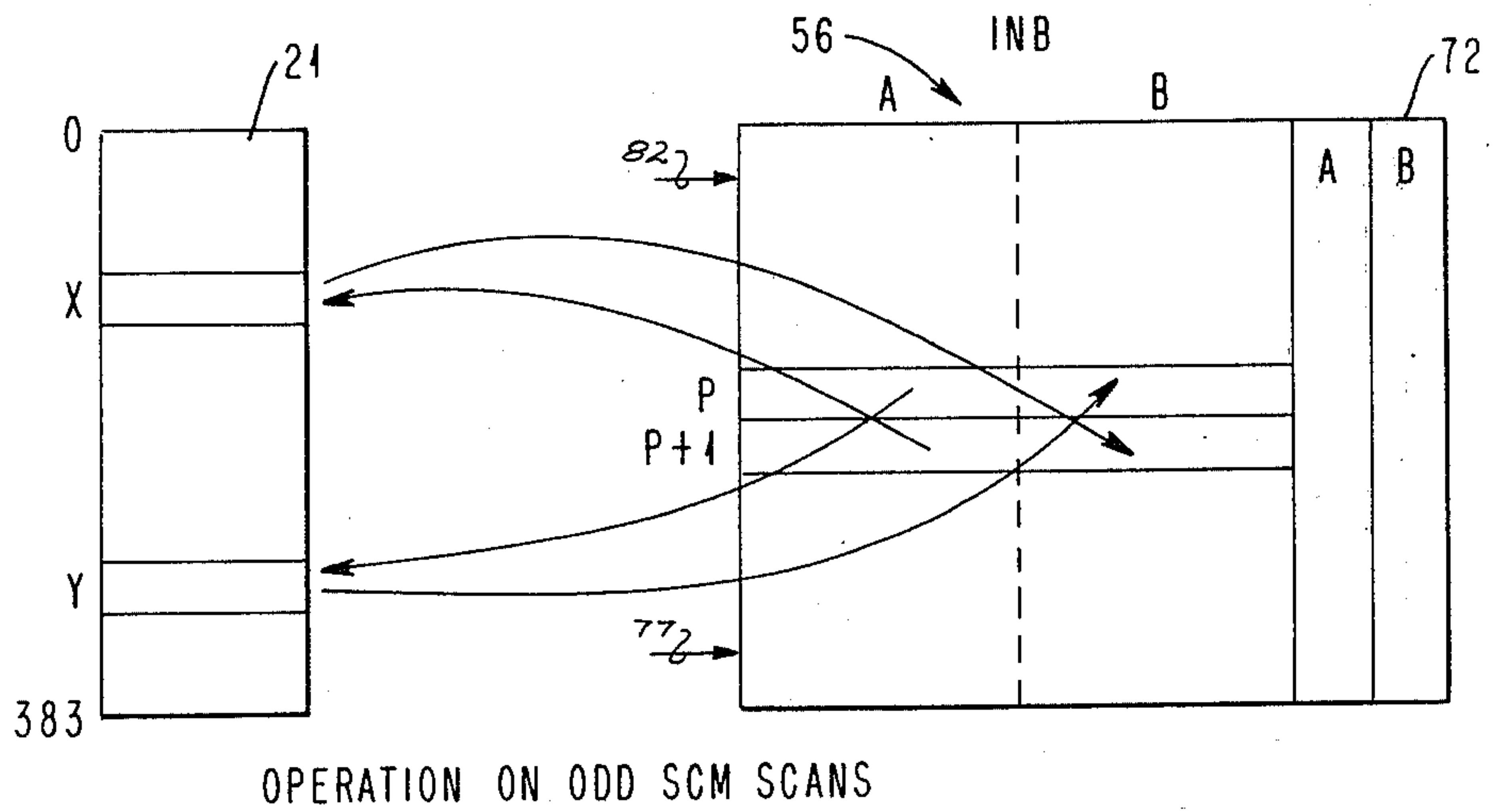
PORTS X & Y COMMUNICATING INTRANODALLY
