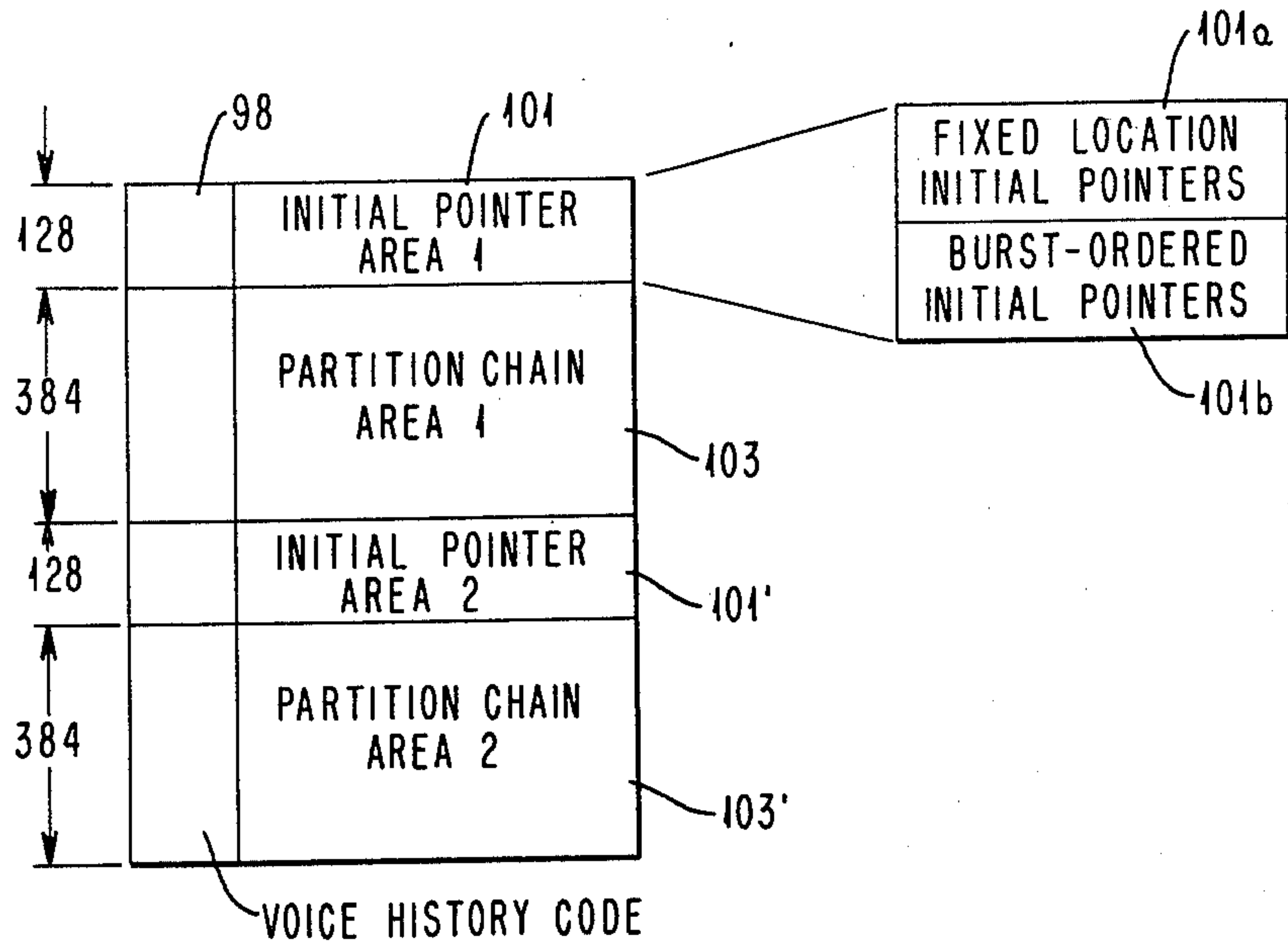
FIG. 45 BURST PRIORITY RAM 100
