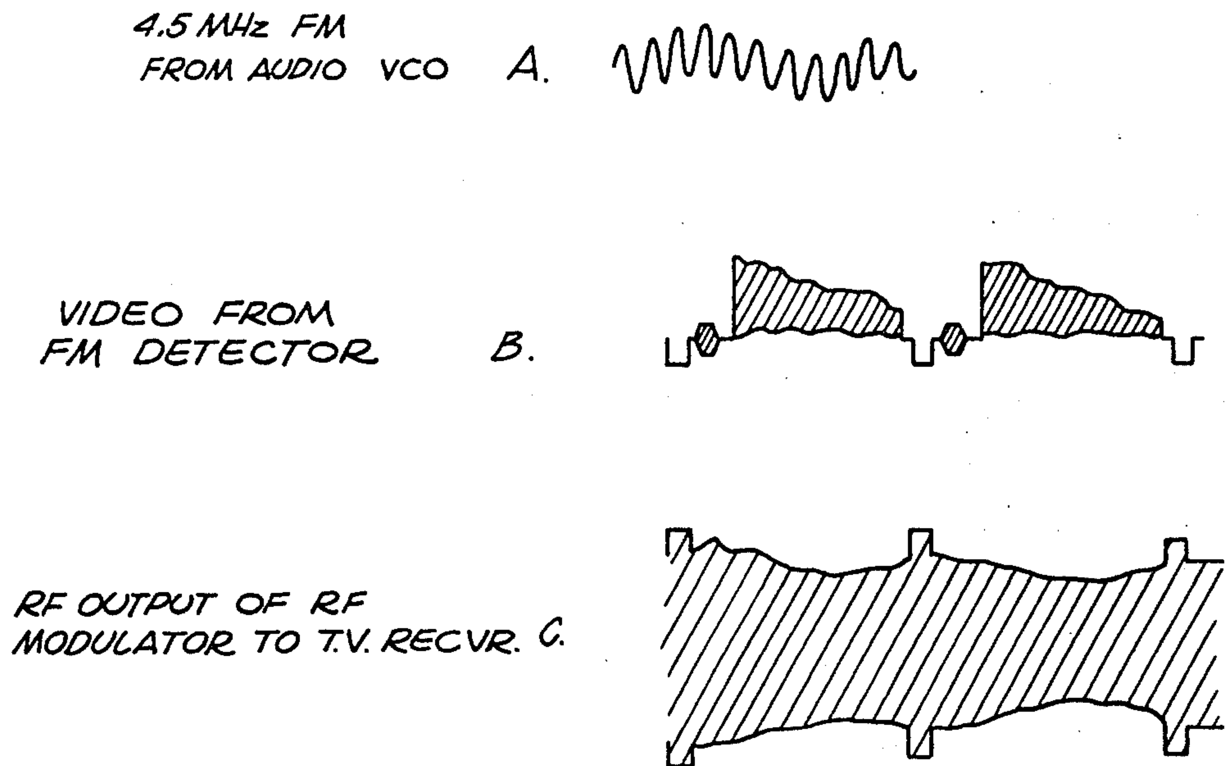
FIG. 25 RF MODULATOR
