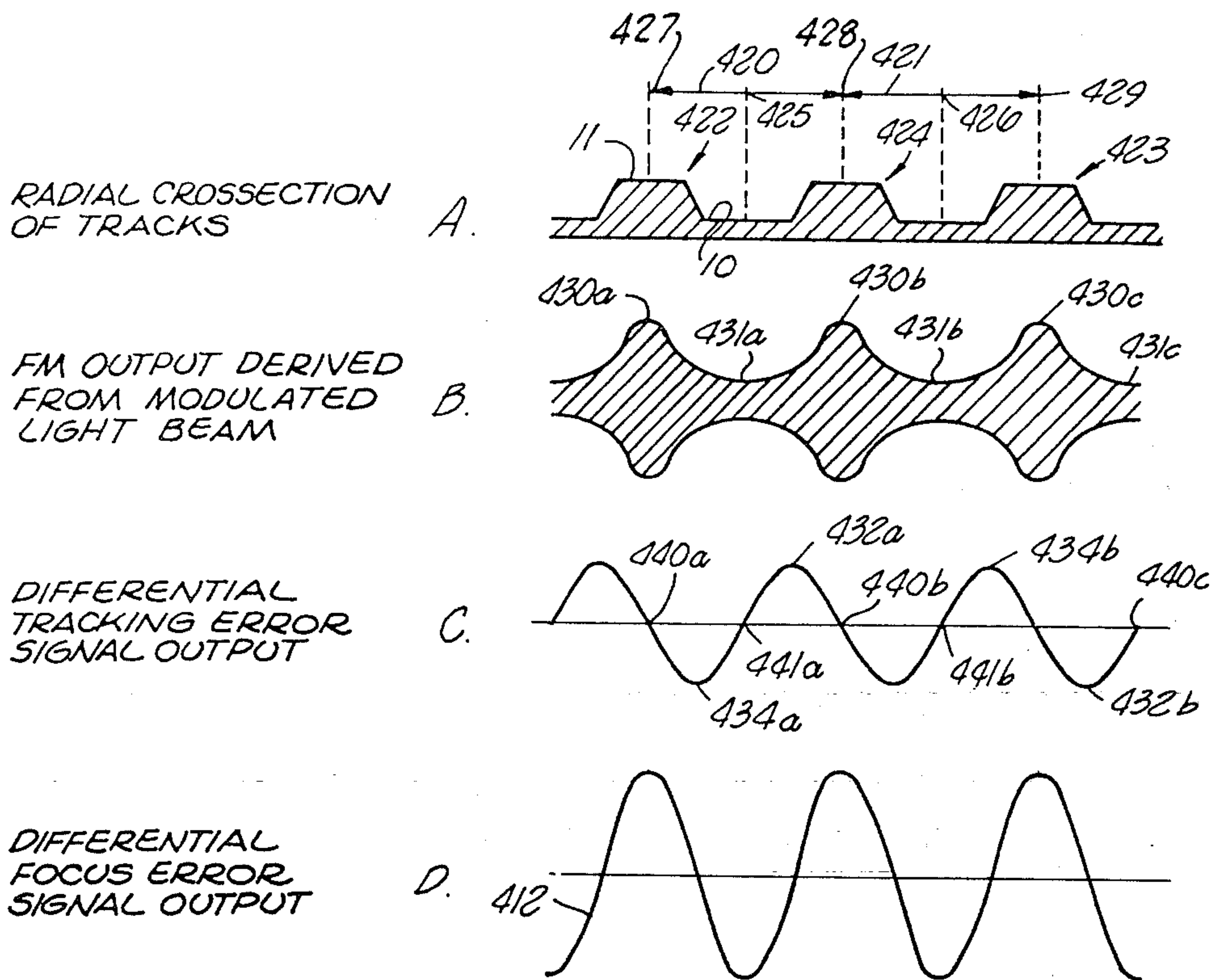
FIG. 8 SIGNAL RECOVERY
