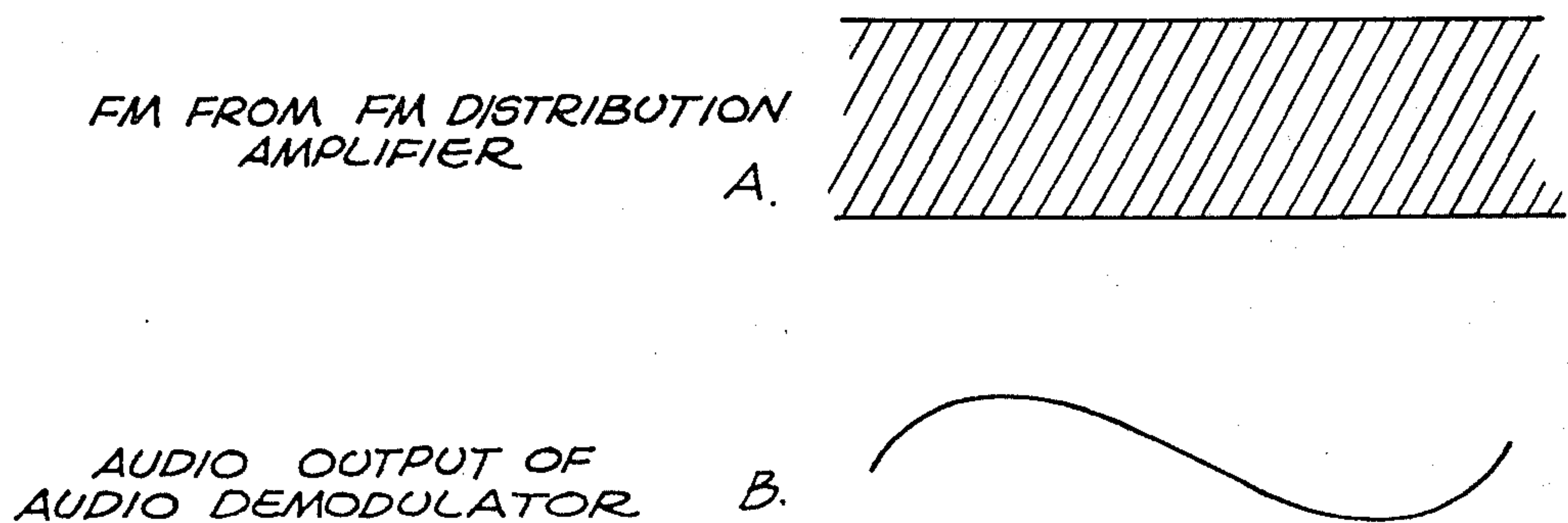
FIG. 21 AUDIO DEMODULATOR
