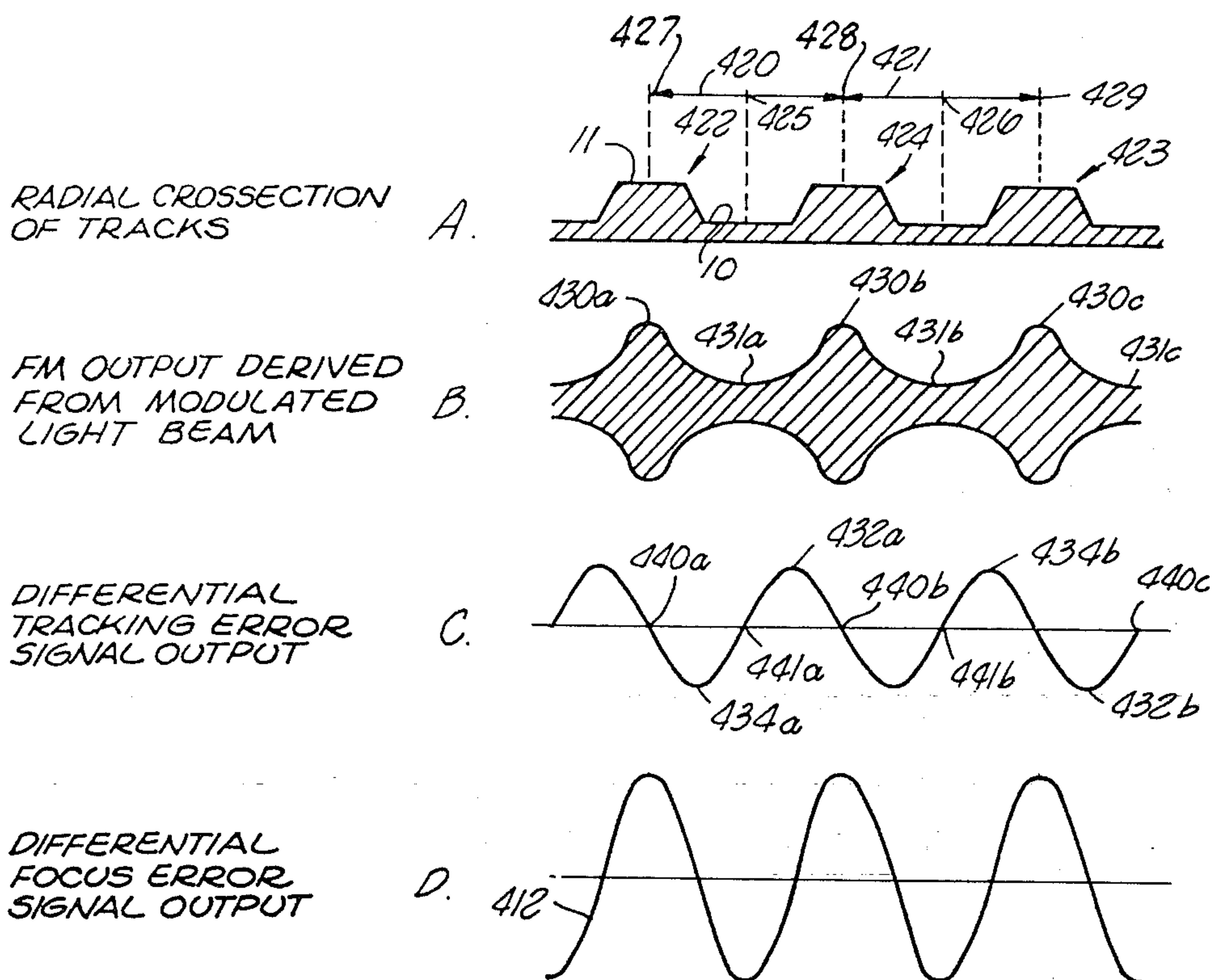
FIG. 8 SIGNAL RECOVERY
