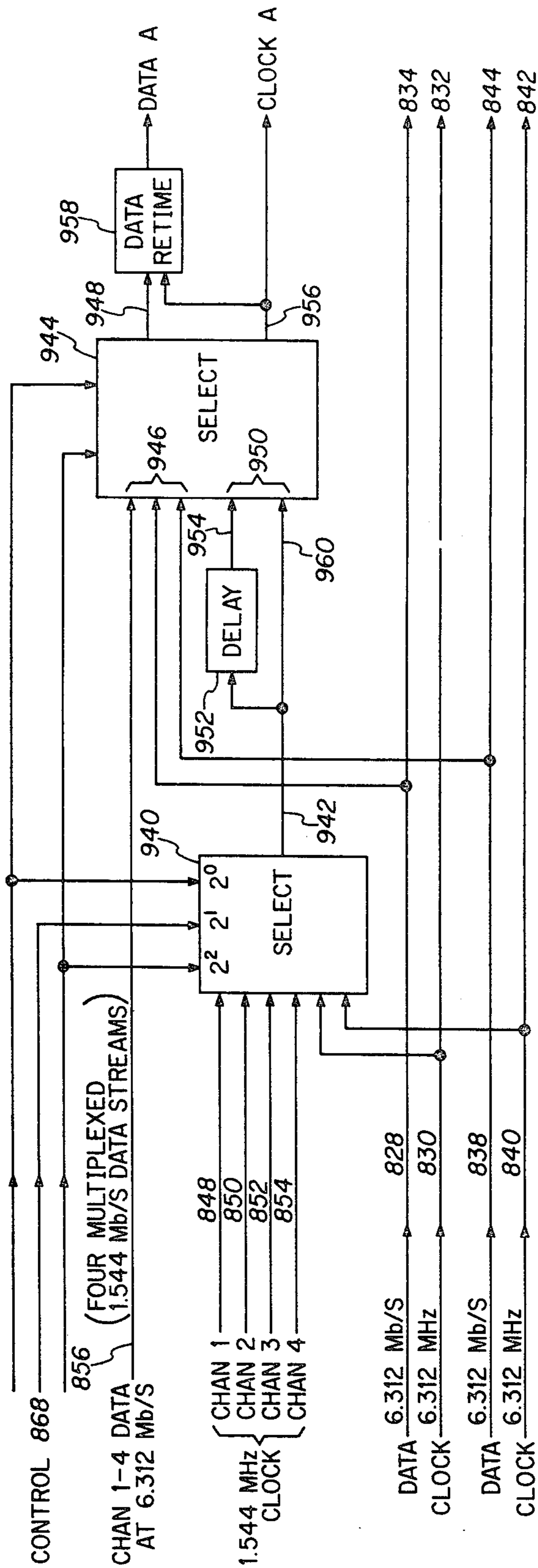
FIG. 15 810A SECTION A OF DATA COMPARATOR INTERFACE
