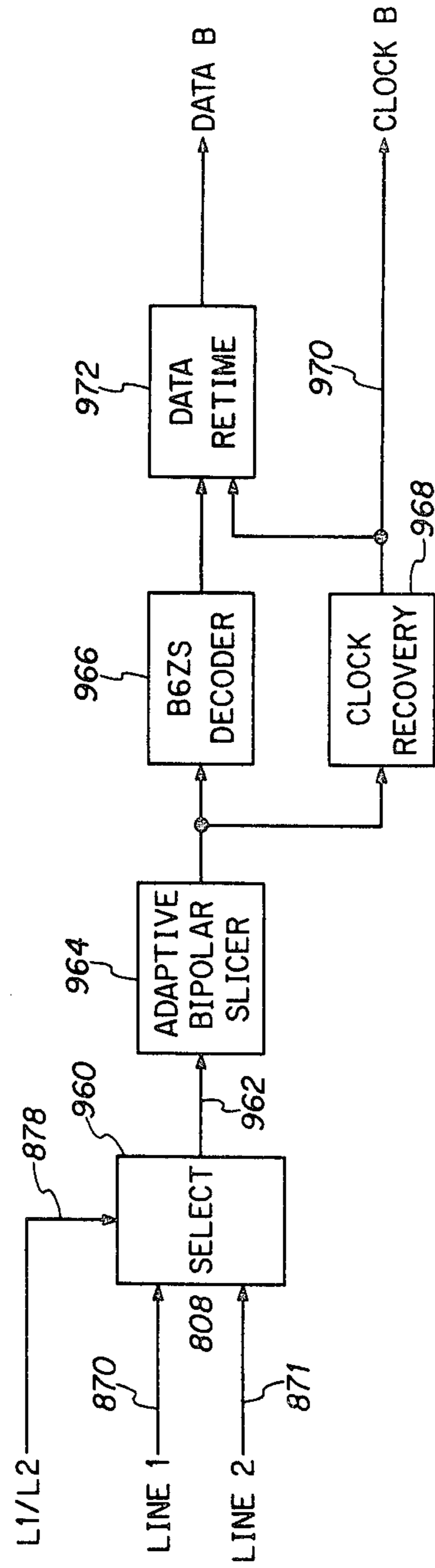
FIG. 16 810B SECTION B OF DATA COMPARATOR INTERFACE
