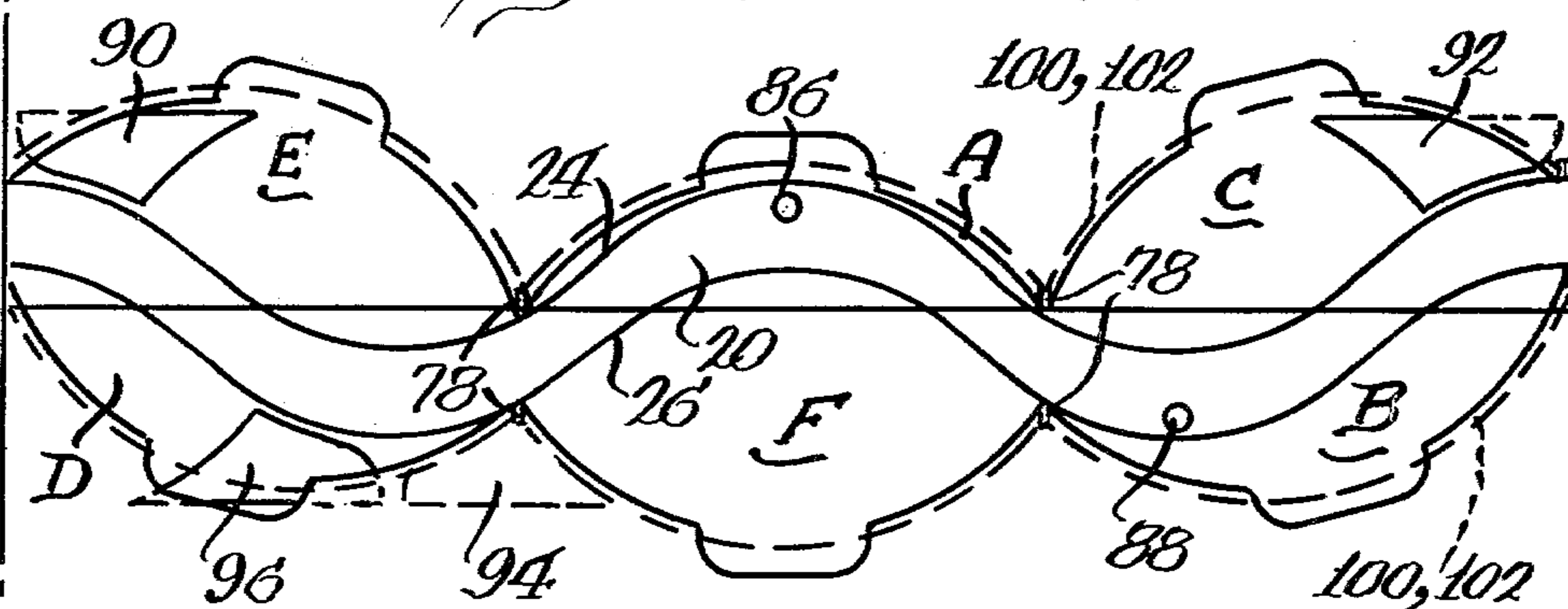
Fig. 4. TIMING SCHEMATIC +60° ROTATION
