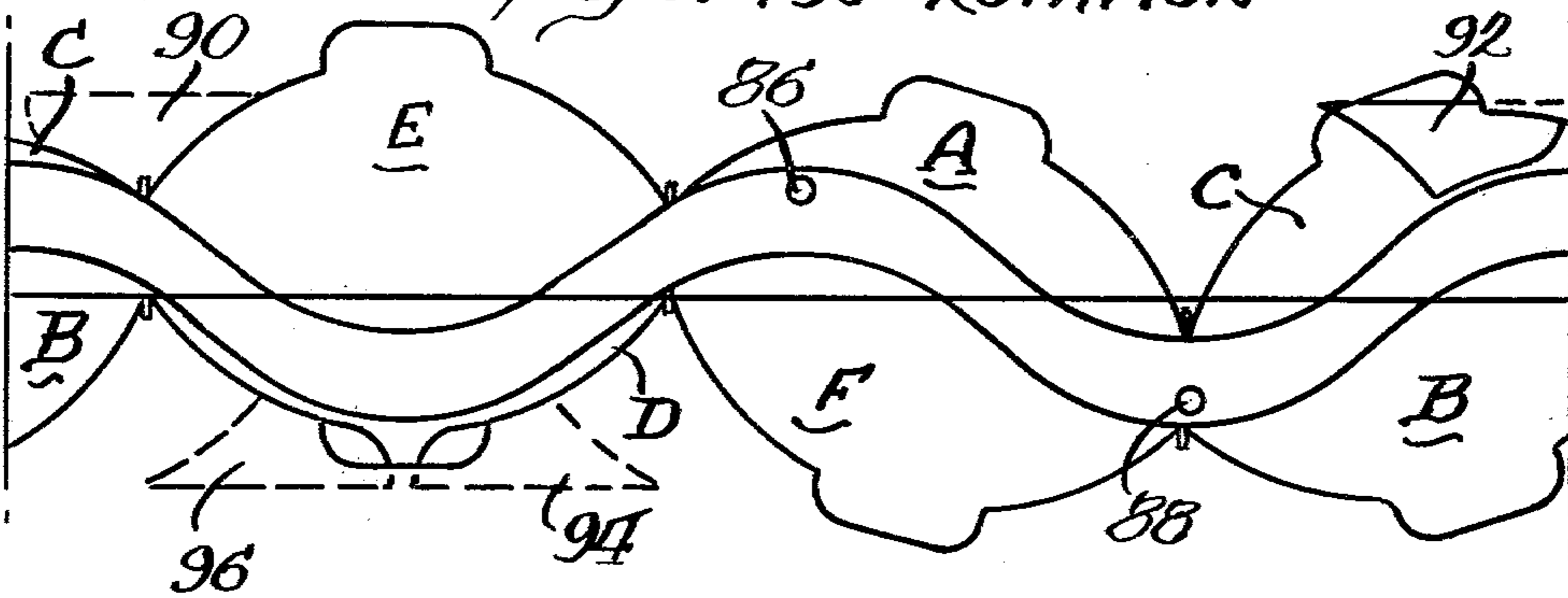
Fig. 3. TIMING SCHEMATIC +30° ROTATION
