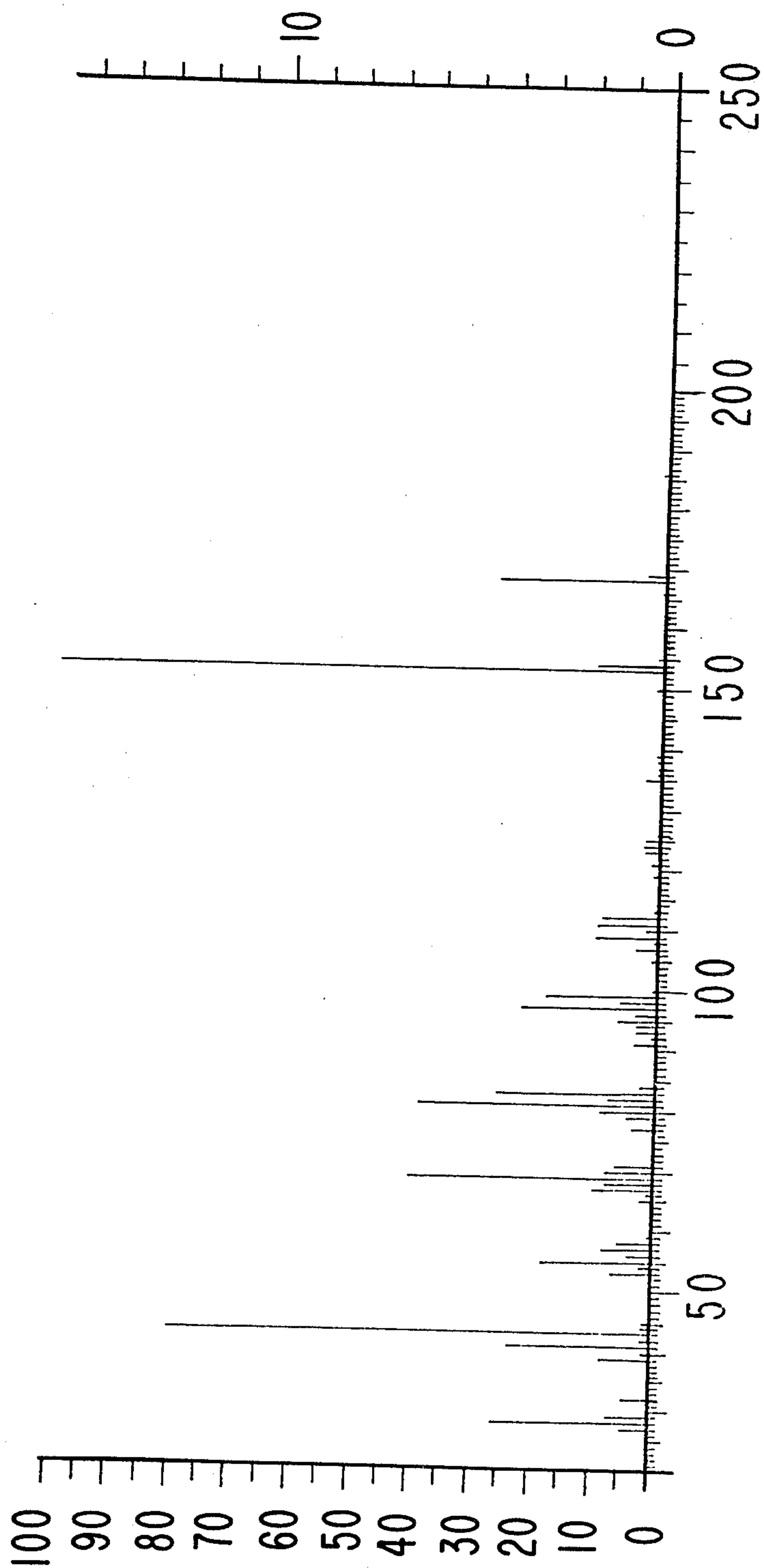
MASS SPECTRUM FOR EXAMPLE III.
