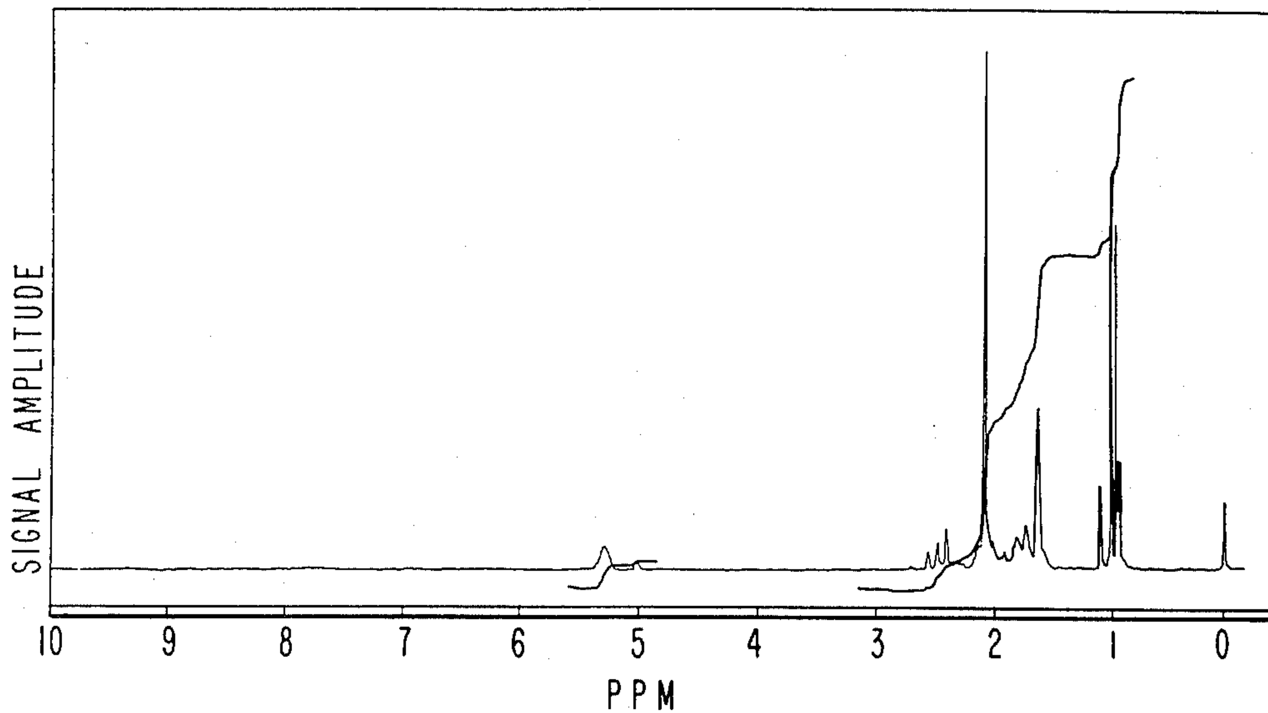
NMR SPECTRUM FOR EXAMPLE I, FRACTION B.
