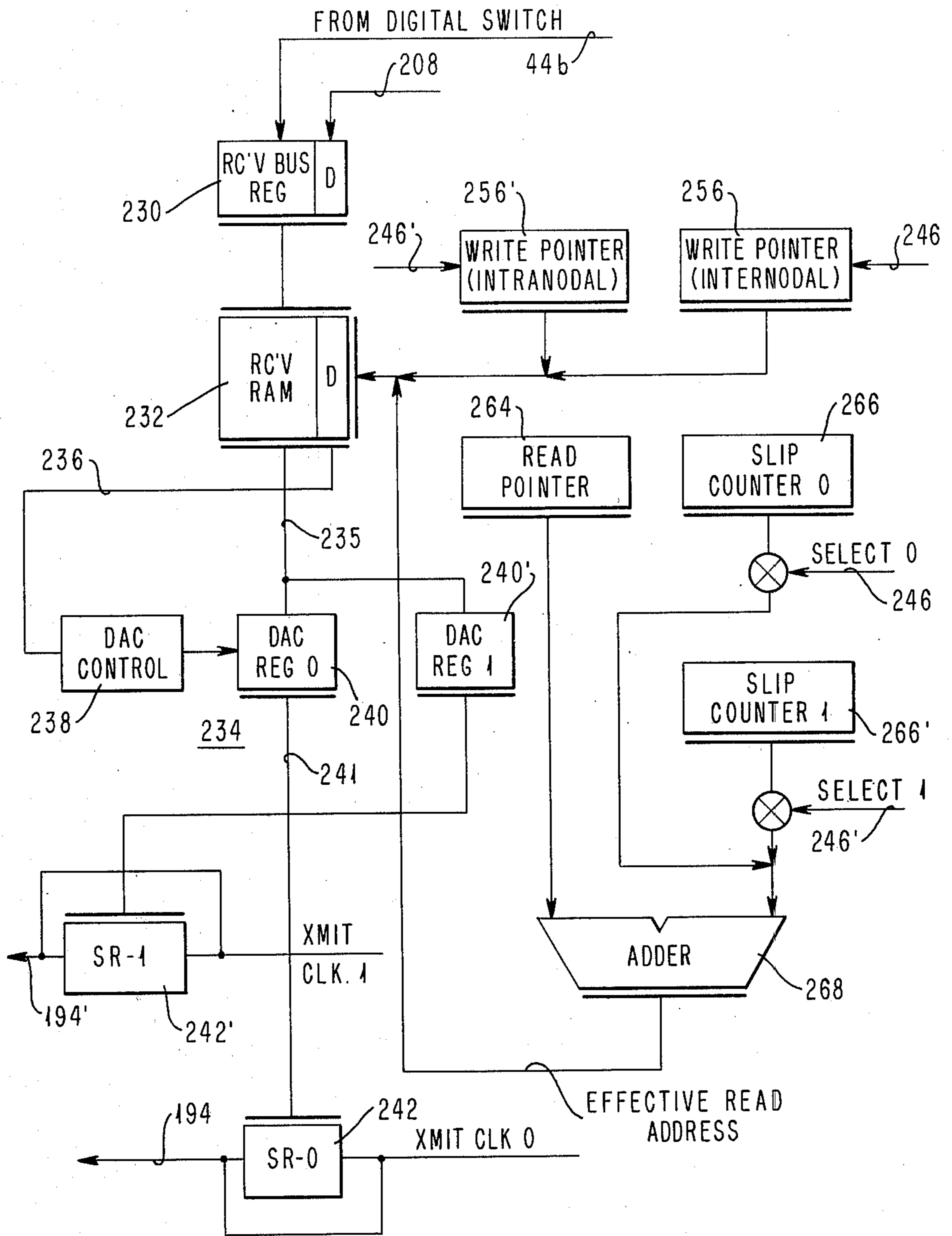
FIG. 27 DATA PORT RECEIVE MECHANISM
