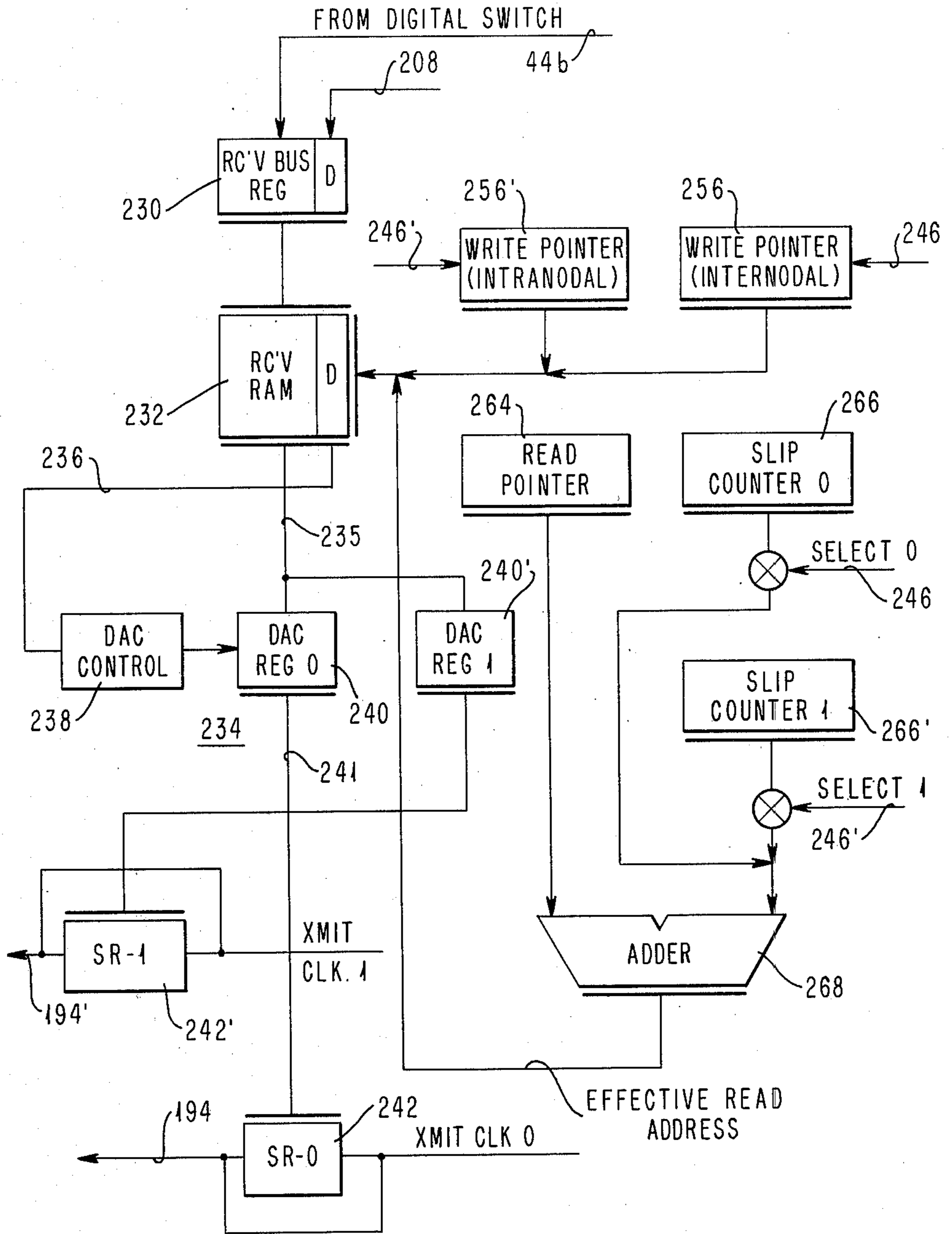
FIG. 27 DATA PORT RECEIVE MECHANISM
