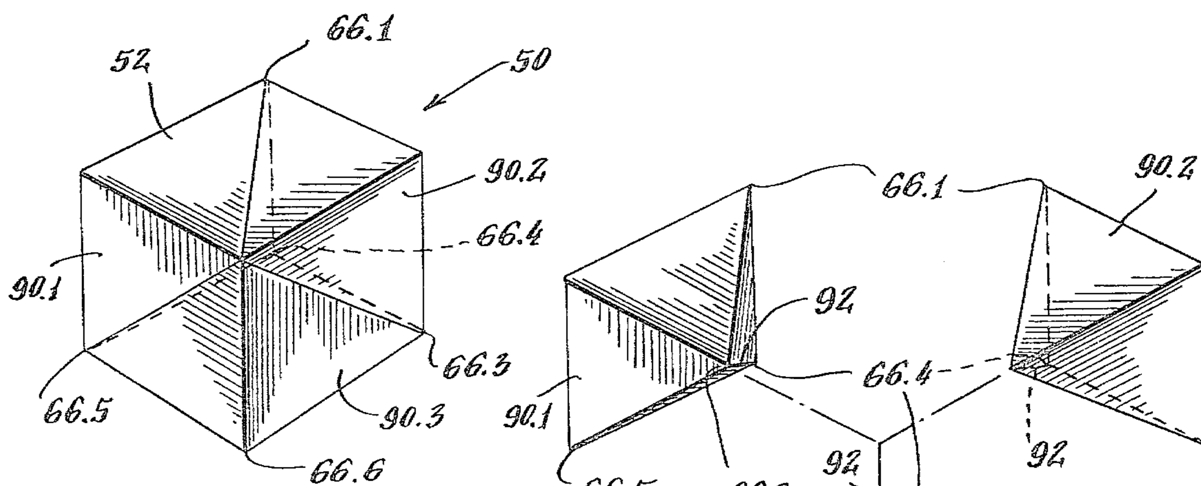
Fig. 12. TRISECTED CUBE
