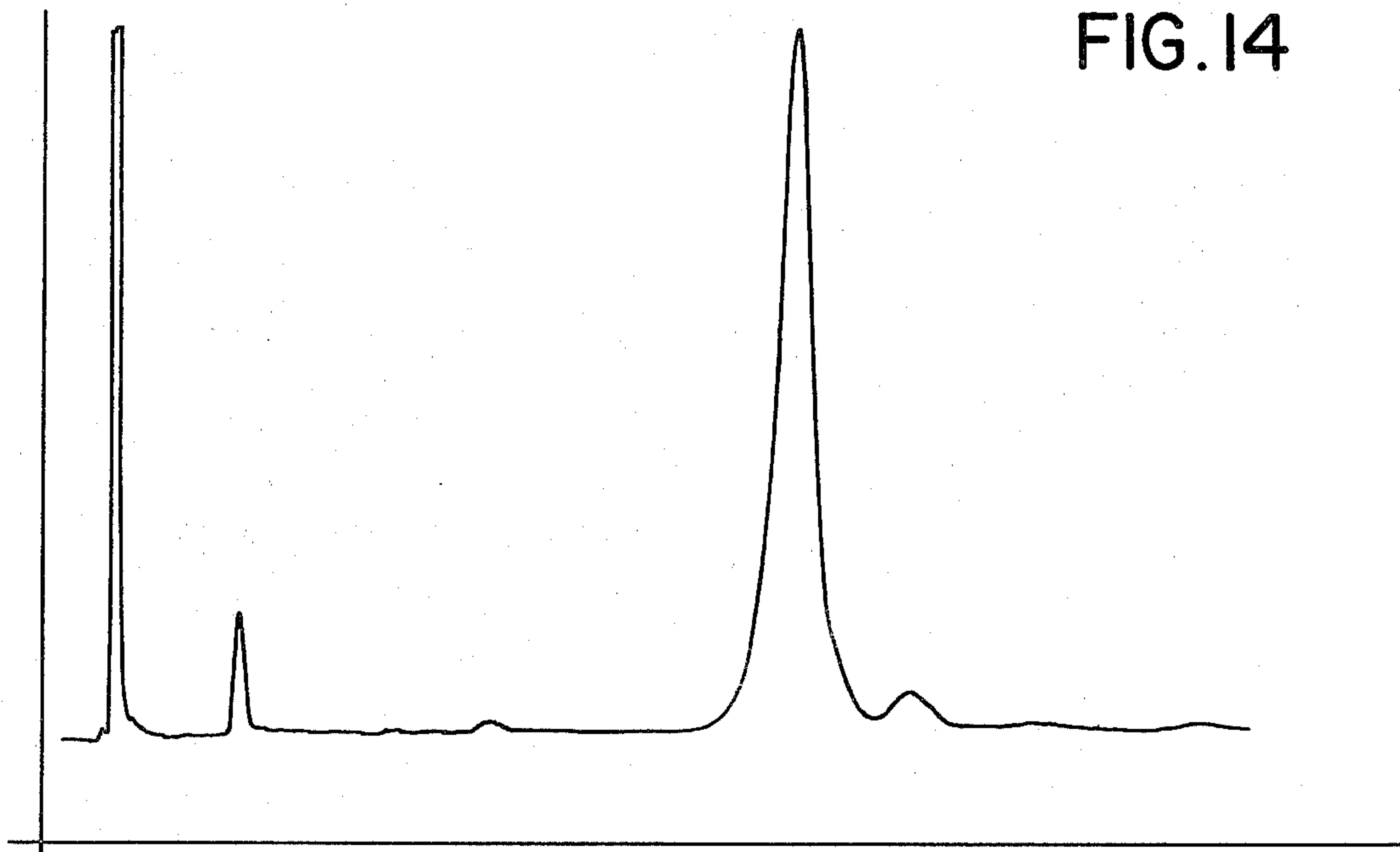
GLC PROFILE FOR EXAMPLE V.
