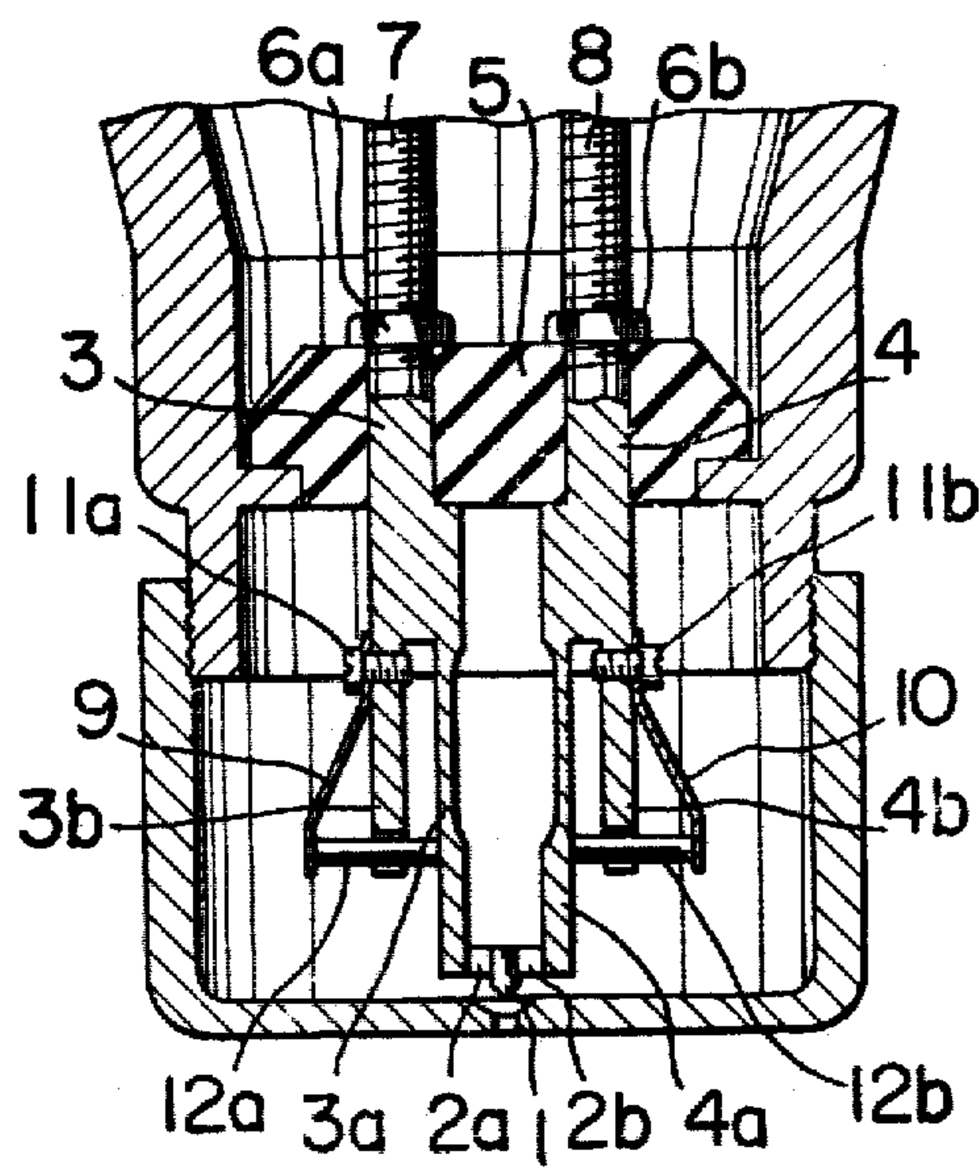
FIG. 1 PRIOR ART
