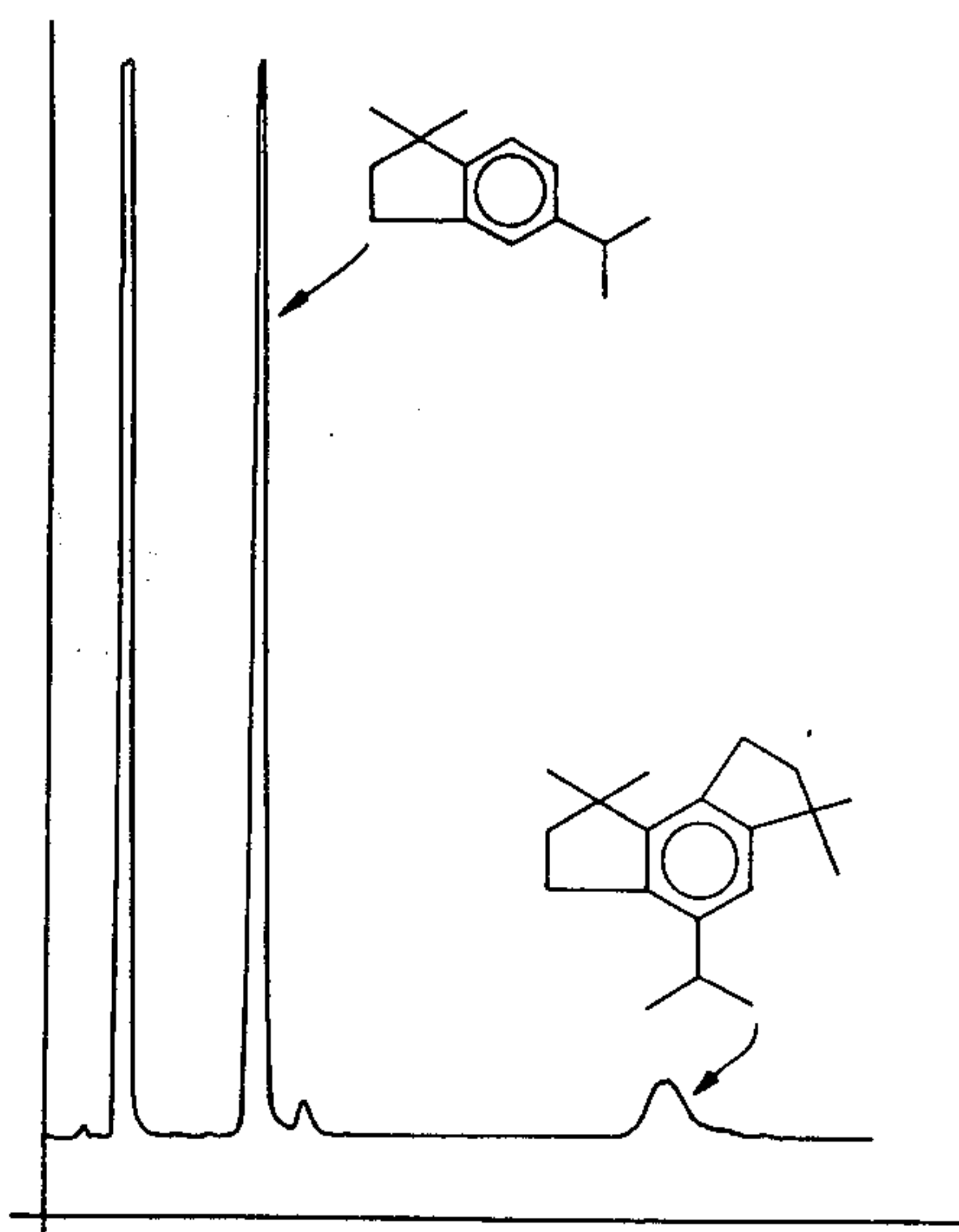
GLC PROFILE FOR EXAMPLE I.
