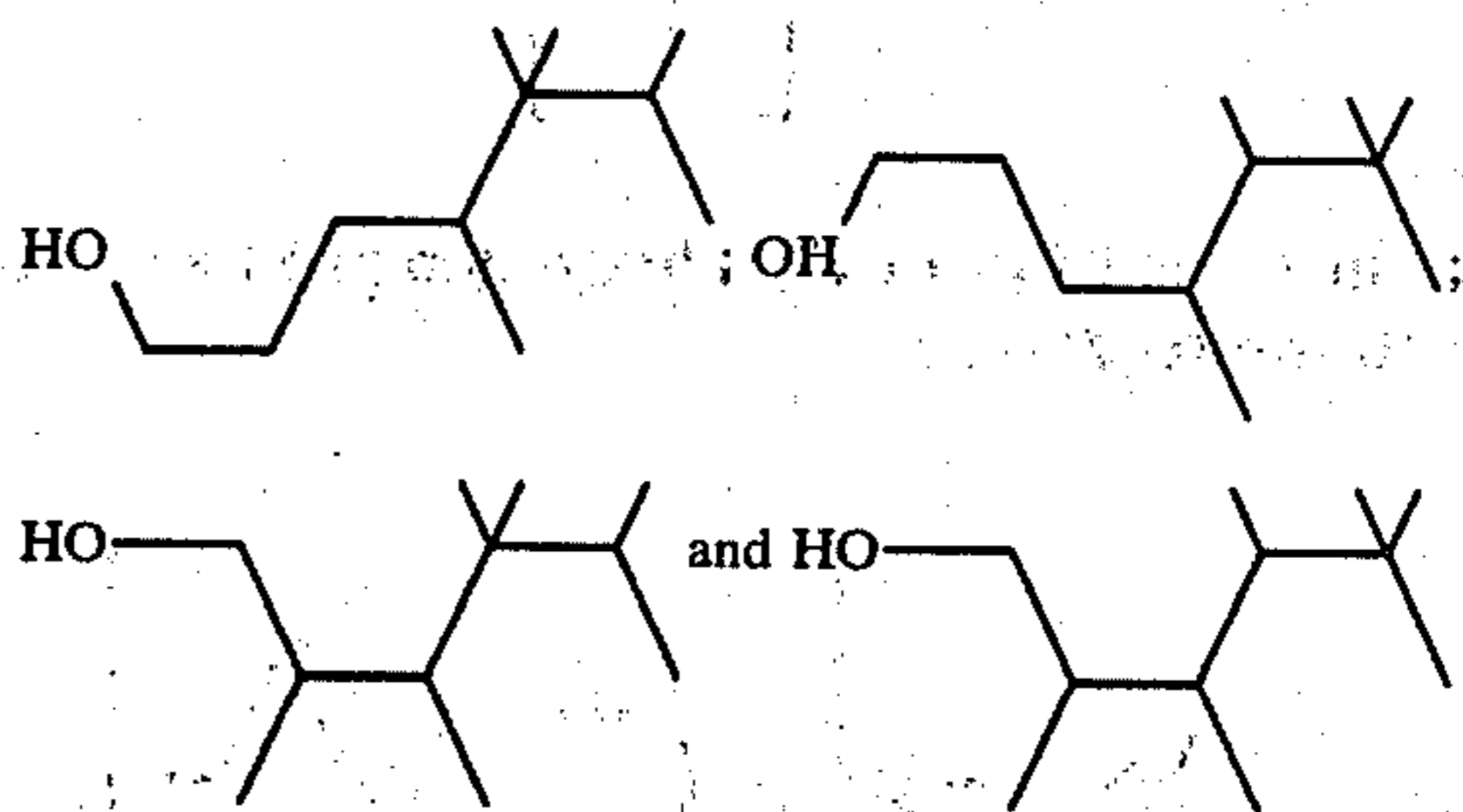
FIG. 10 is the NMR spectrum for the diisoundecanol compounds produced according to Example II having the structures:
