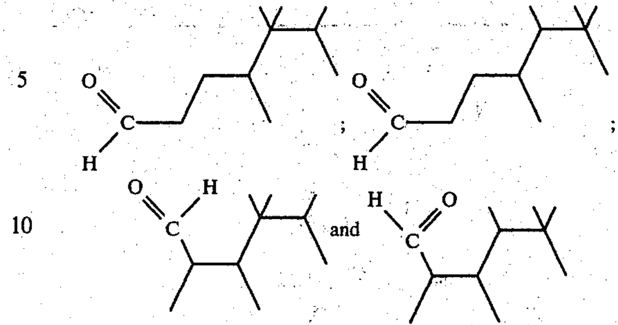
FIG. 9 is the GLC profile (conditions: SF-96, 6" x 1/4" 180° C. isothermal column) produced according to Example II containing the compounds having the structures:
