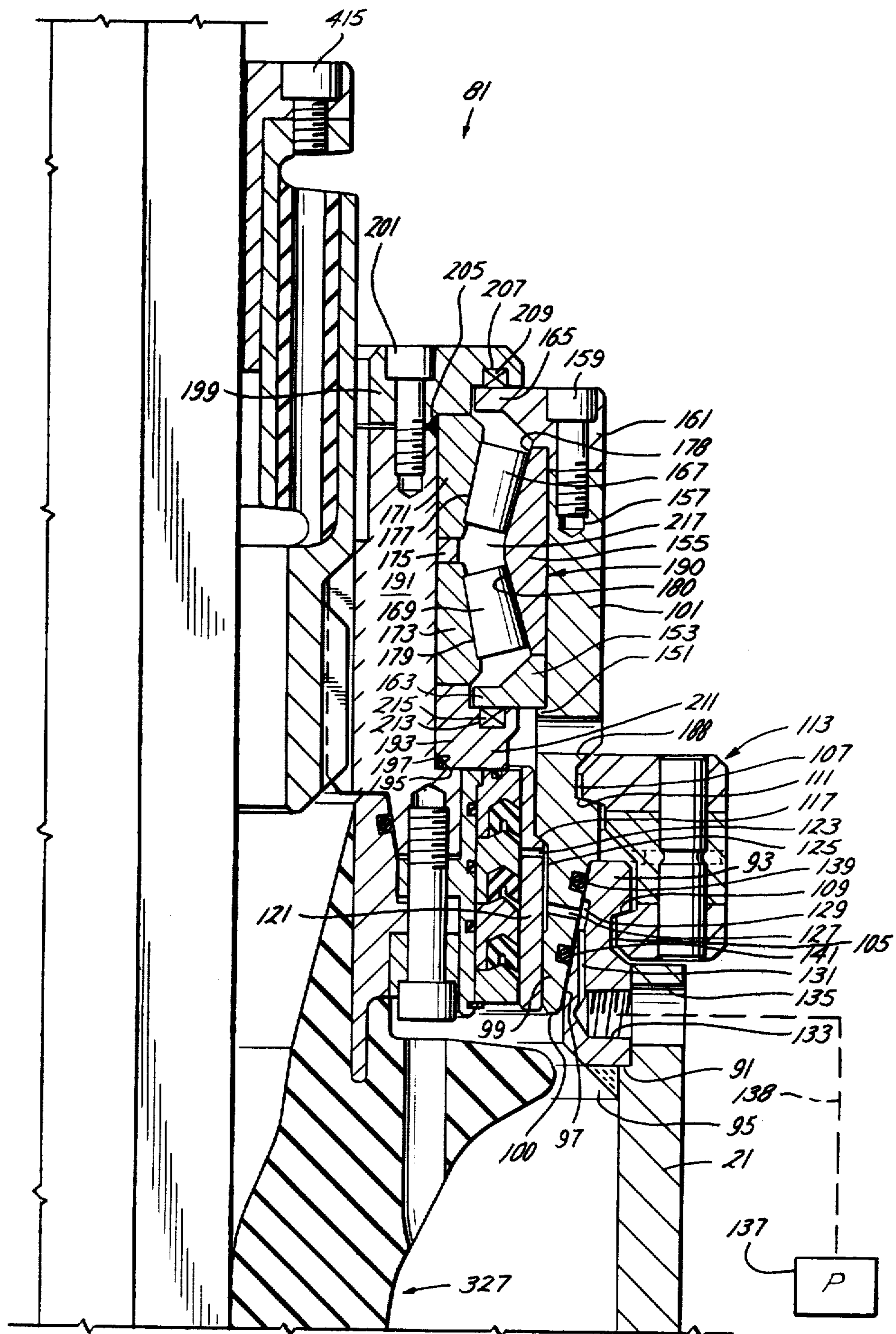
Fig. 4A (ROTATING SEAL LUBRICATION)
