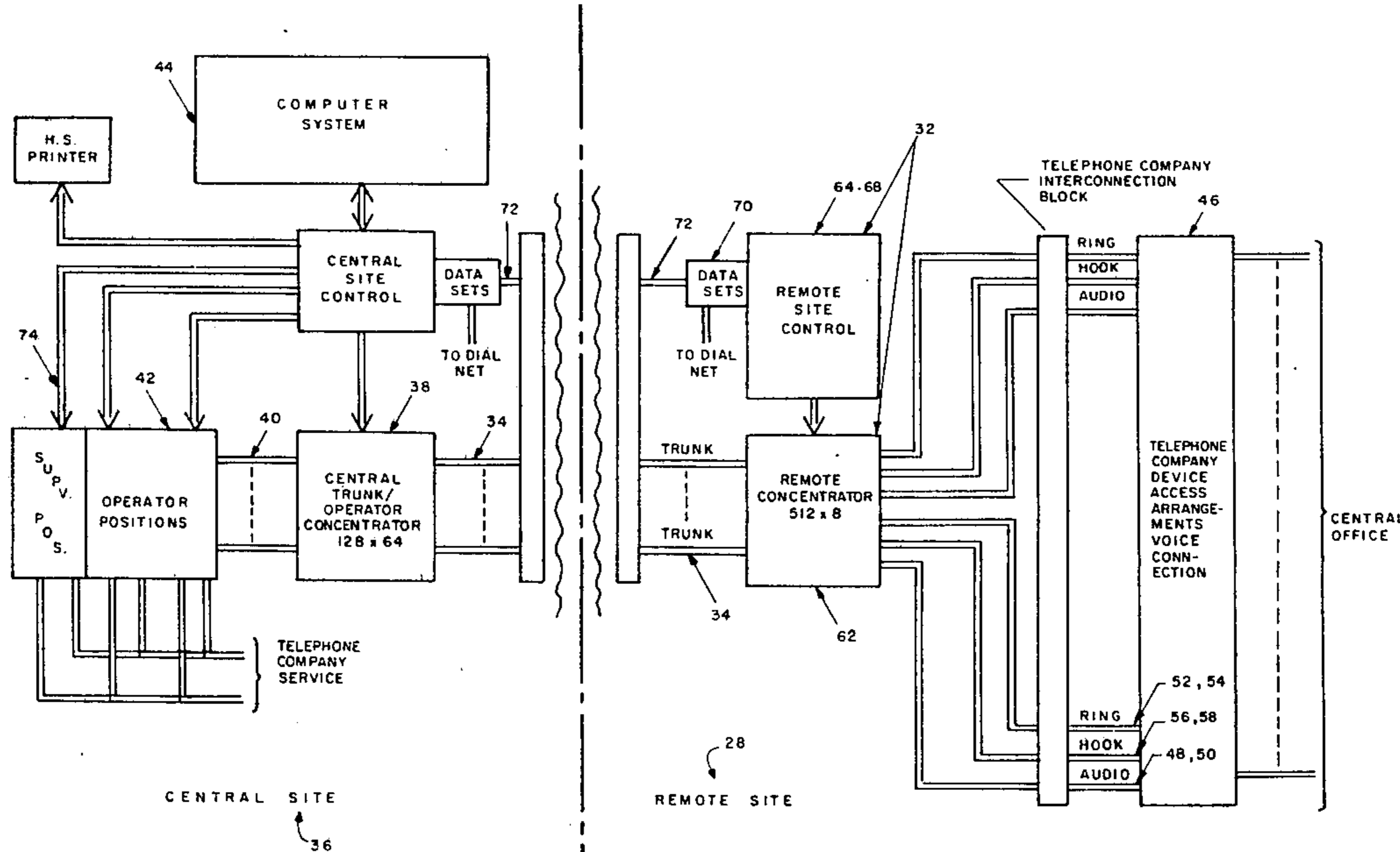
SYSTEM BLOCK DIAGRAM TELEPHONE ANSWERING SERVICE
