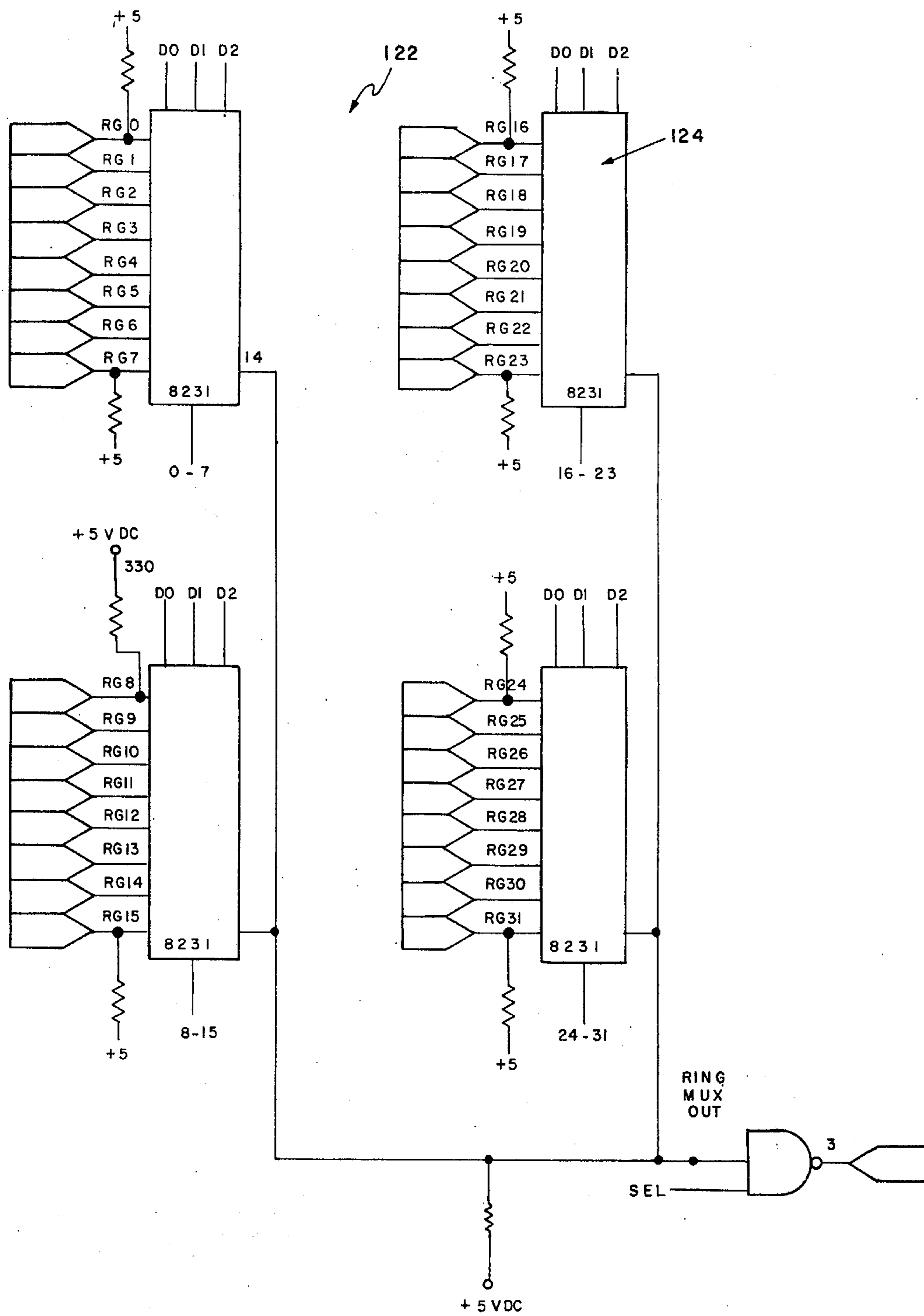
FIG. II RING MUX
