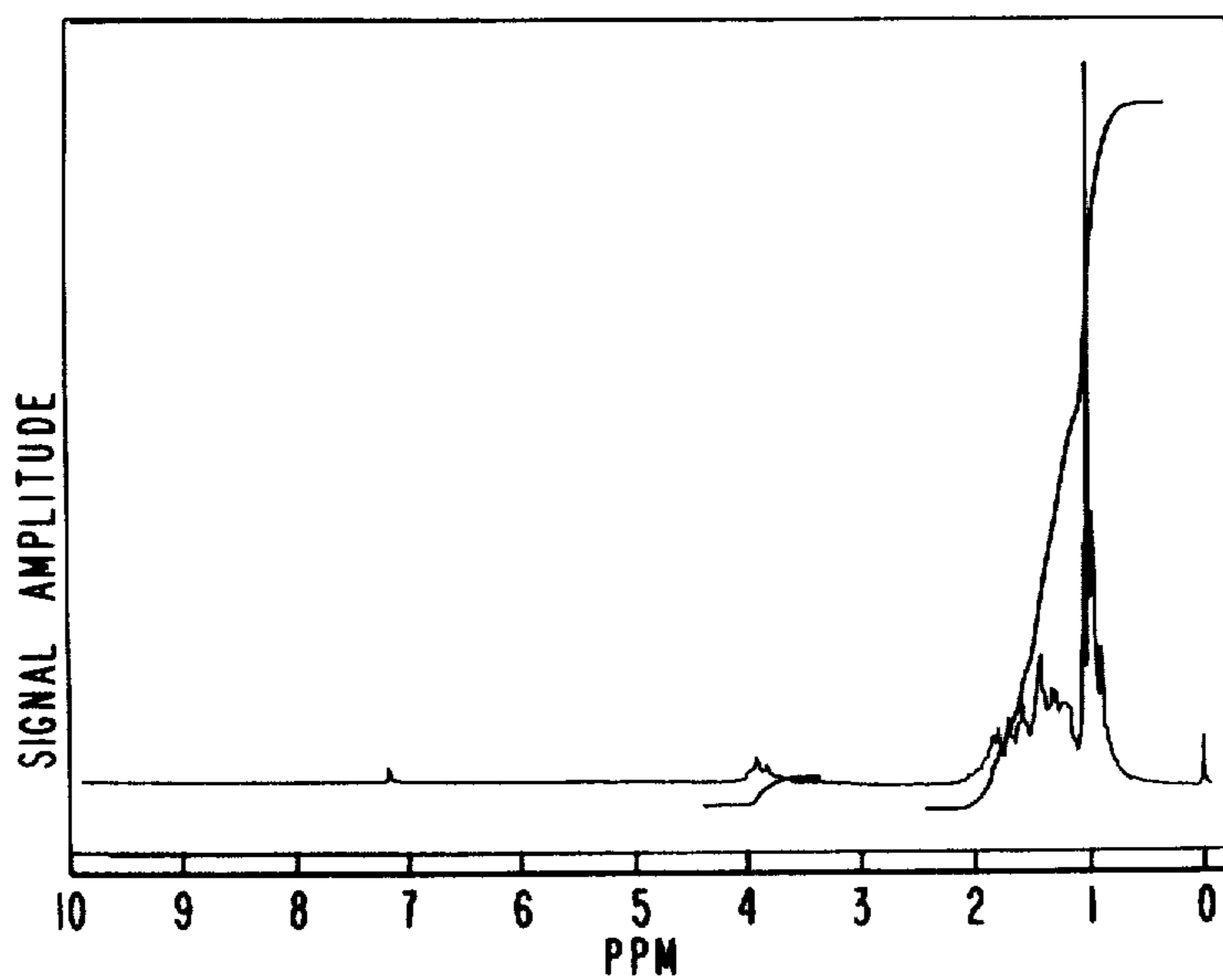
NMR SPECTRUM FOR EXAMPLE IX.
