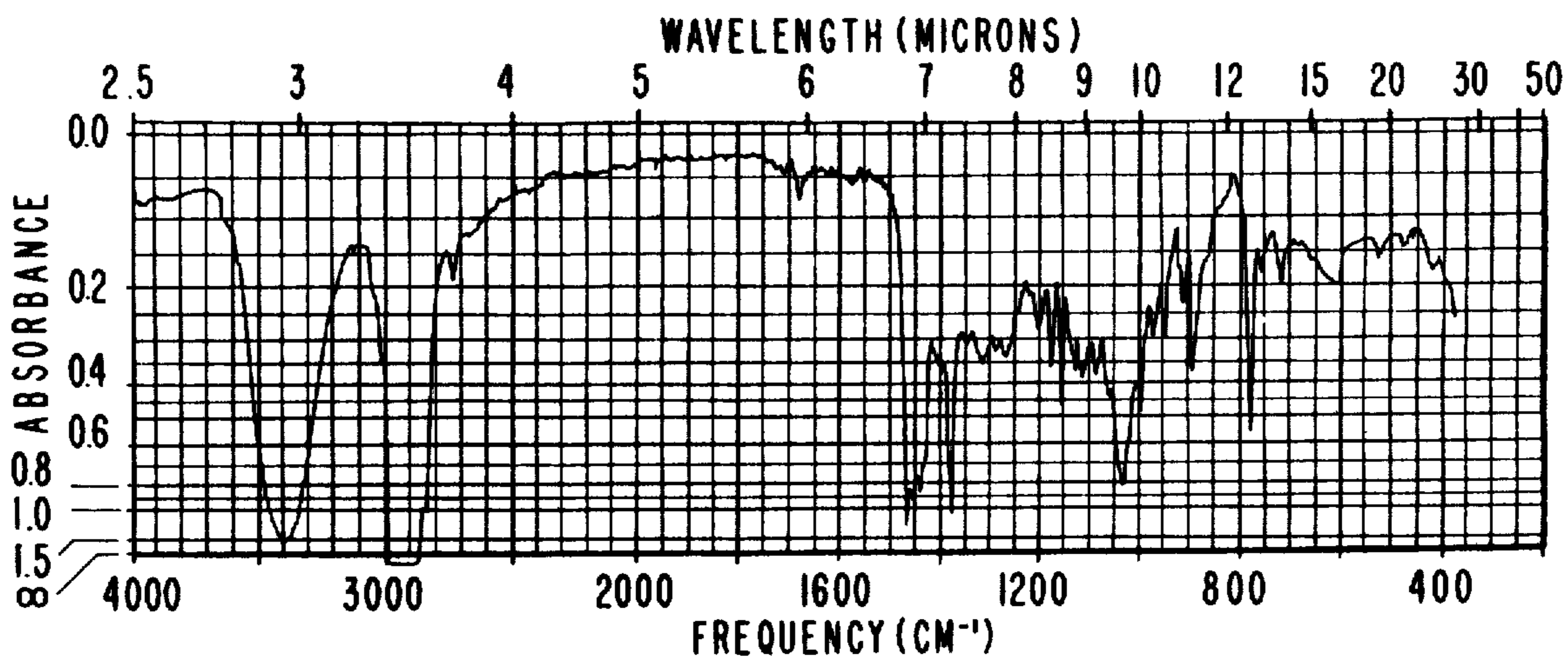
I R SPECTRUM FOR EXAMPLE VII(A).
