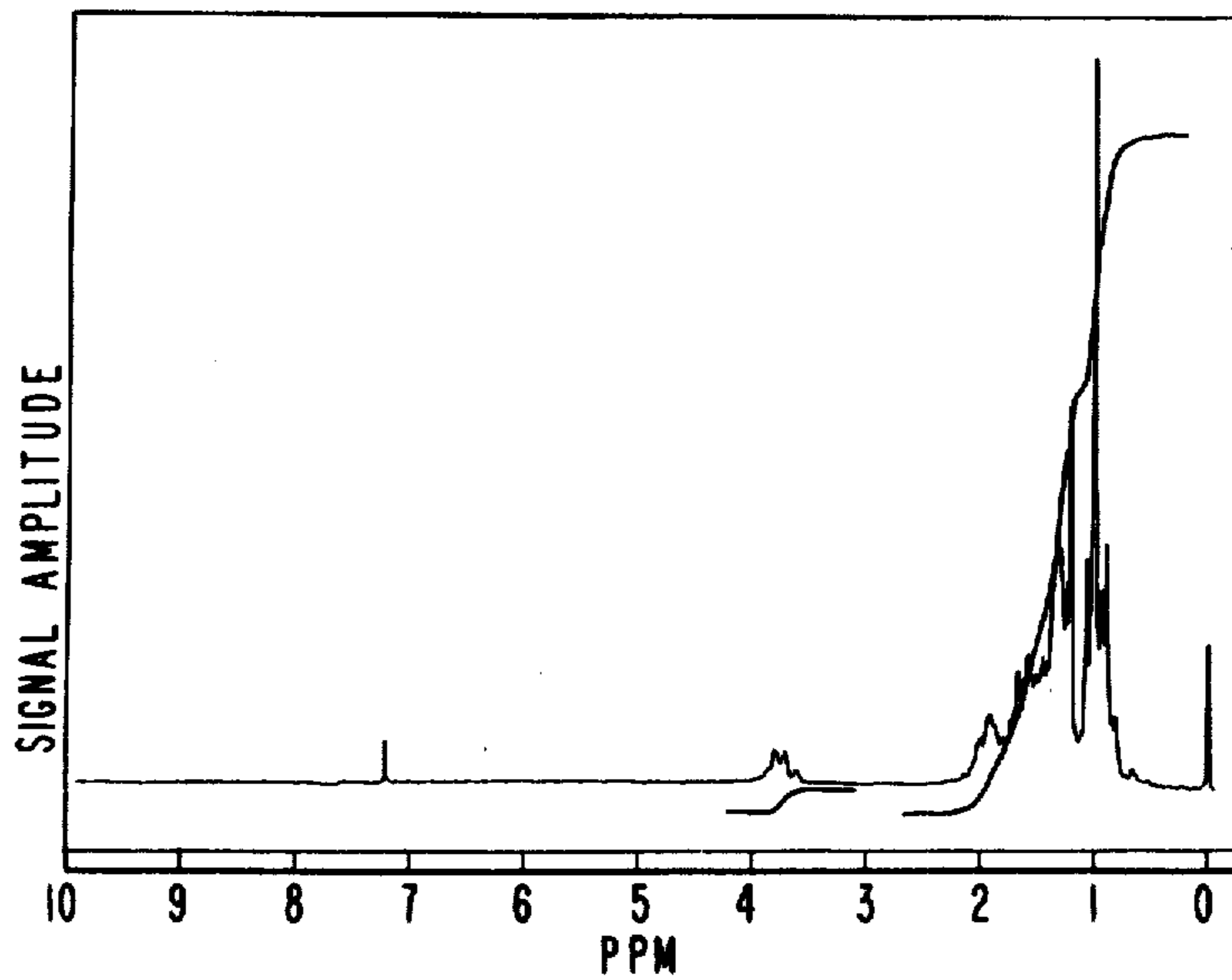
N M R SPECTRUM FOR EXAMPLE VII(B).
