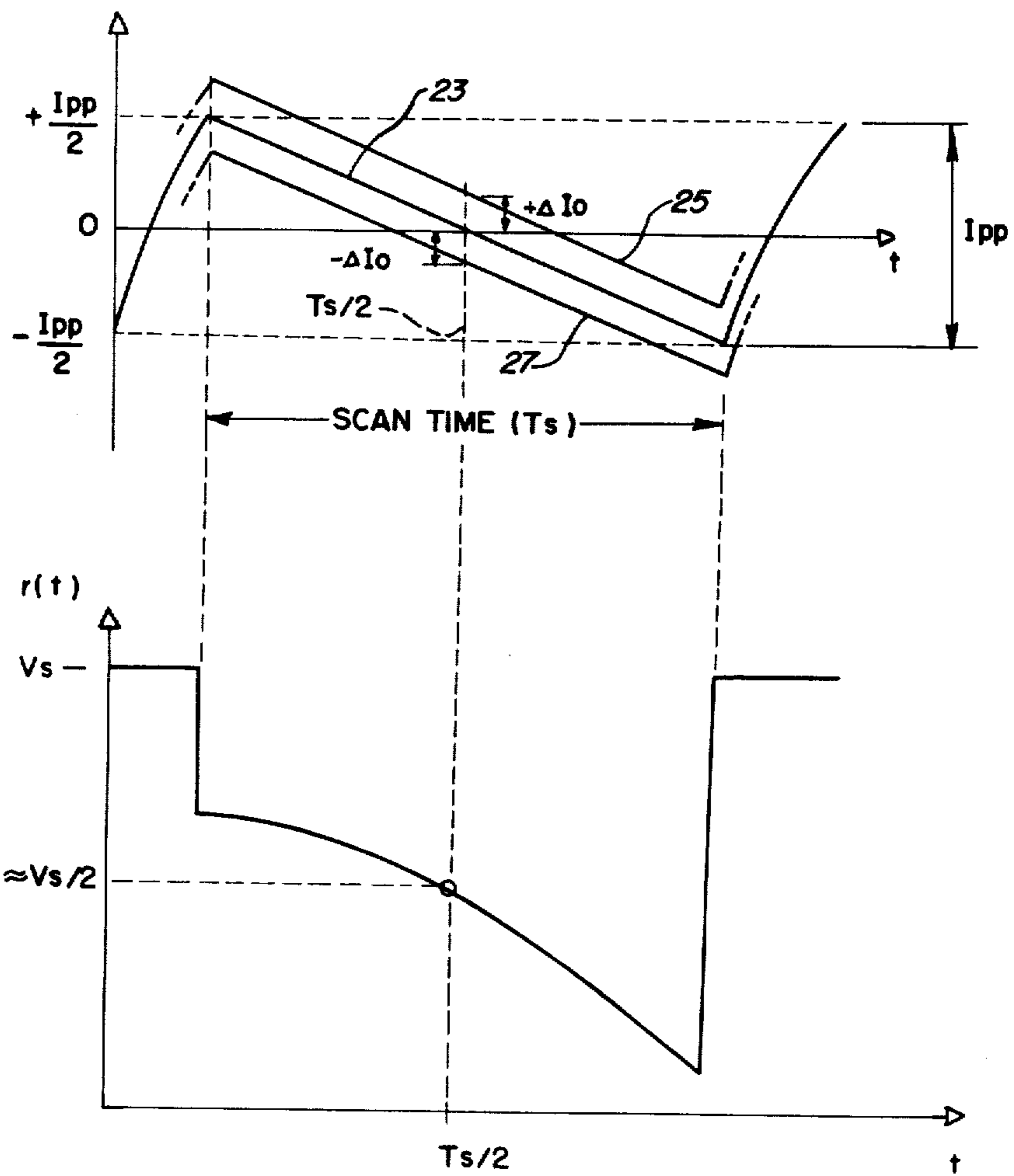
WAVEFORM OF VOLTAGE ACROSS YOKE LOAD
