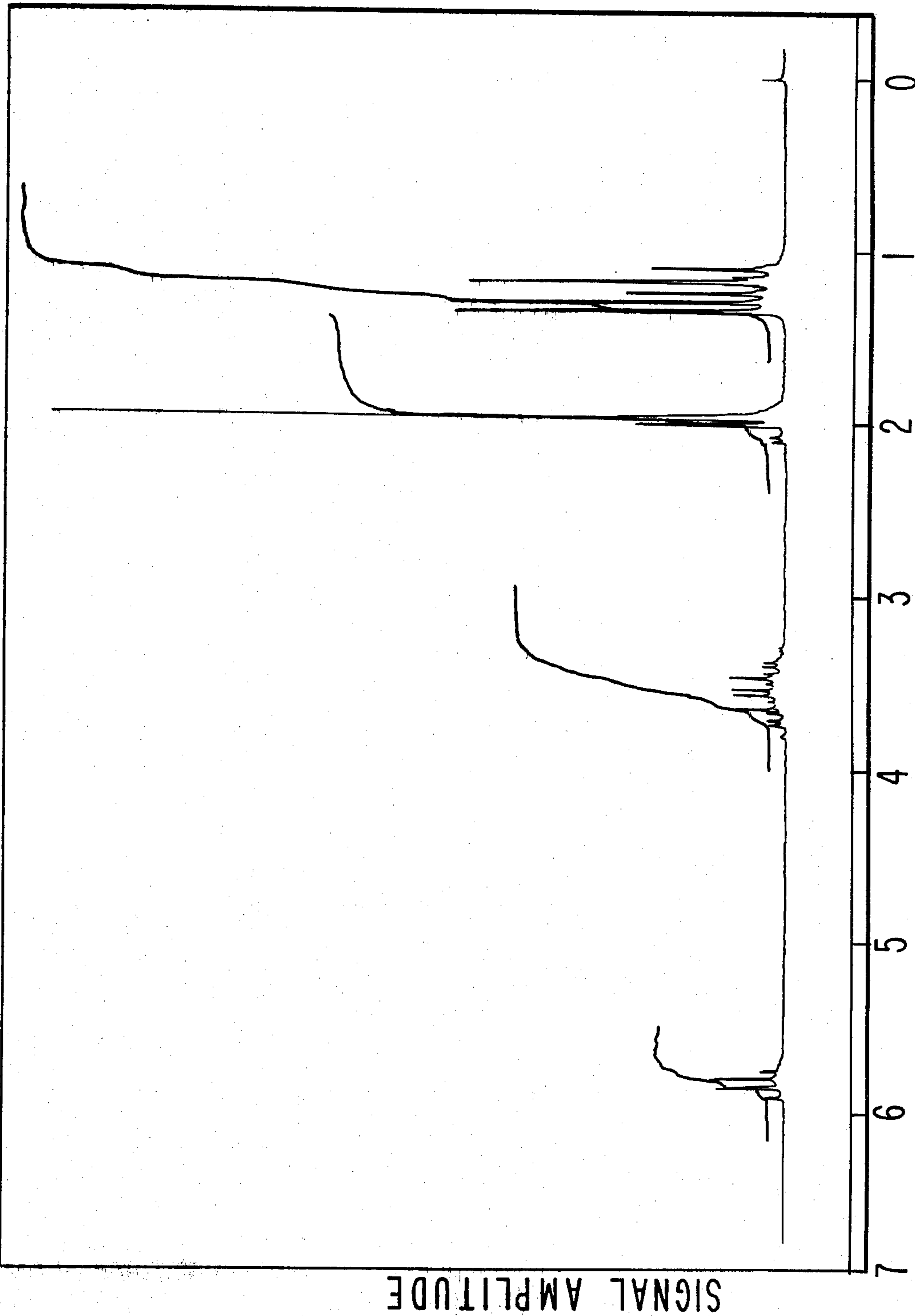
NMR SPECTRUM FOR EXAMPLE I.
