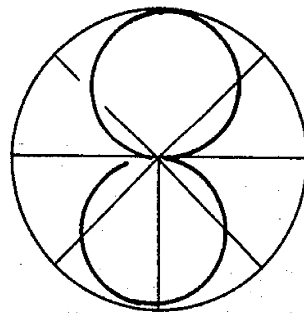
ANTENNA 10
