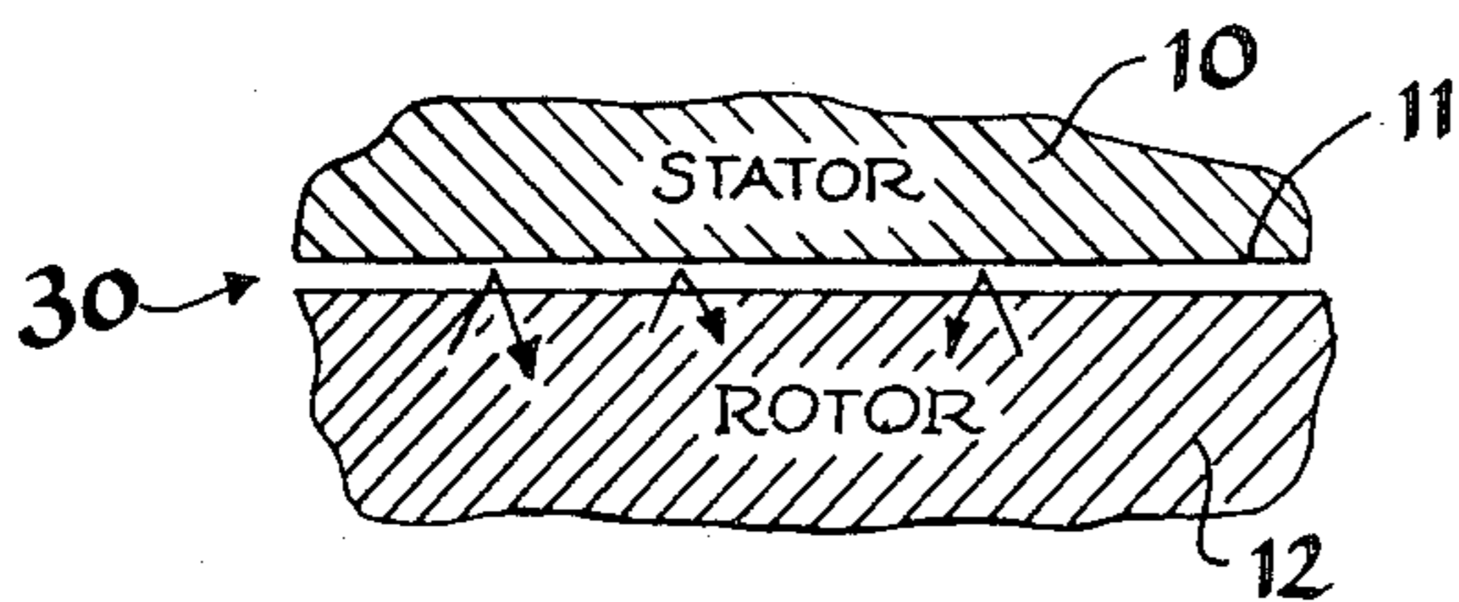
FIGURE 3 PRIOR ART
