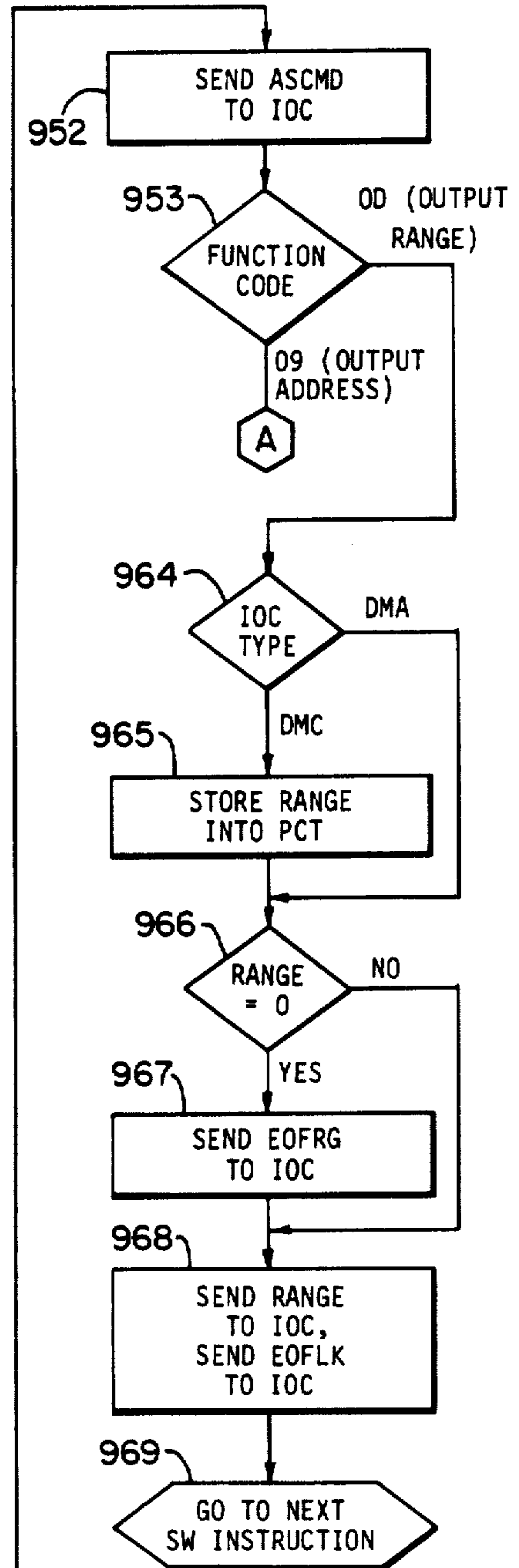
IOLD INSTRUCTION FLOW CHART
