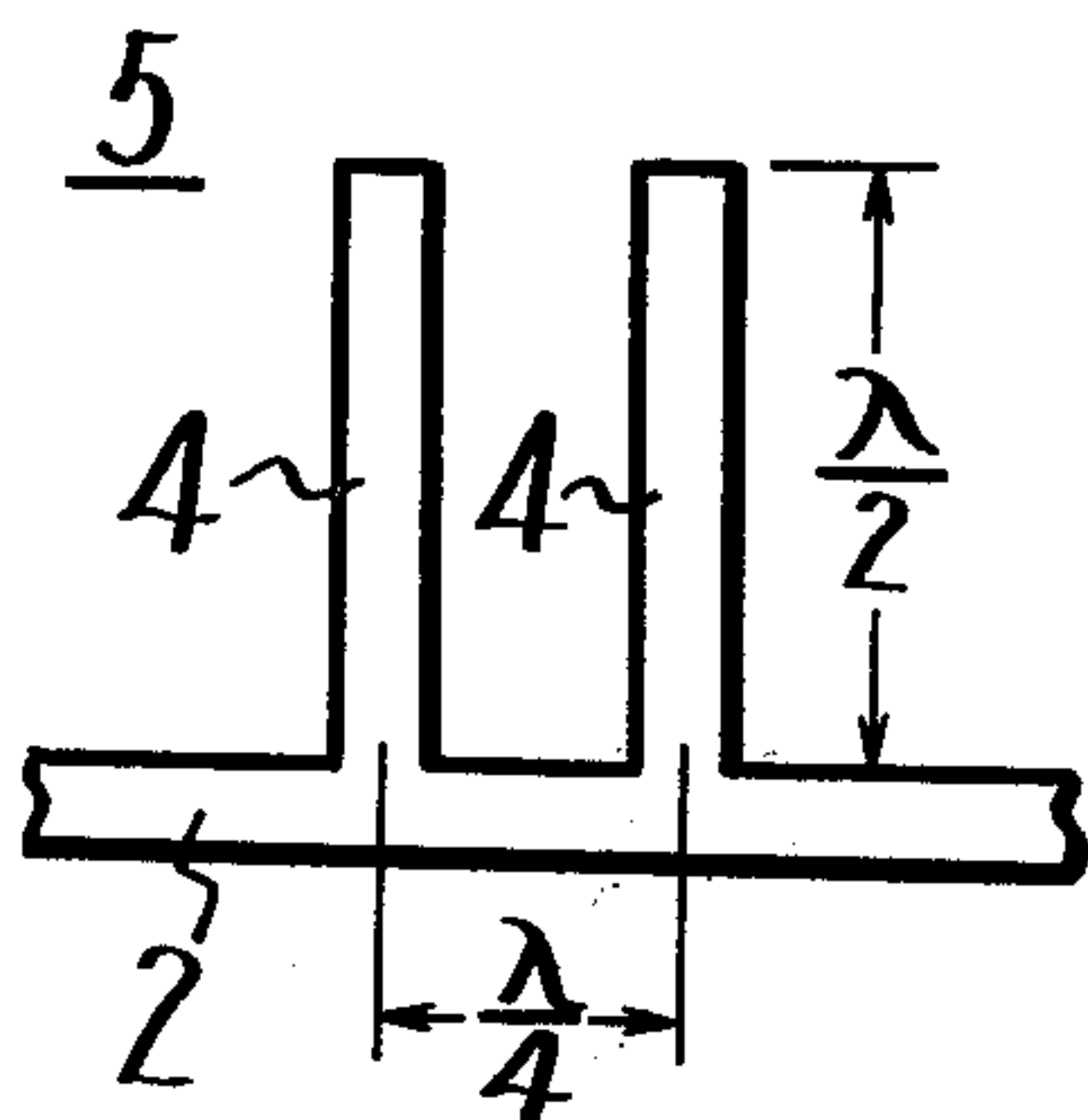
FIG. 2 PRIOR ART
