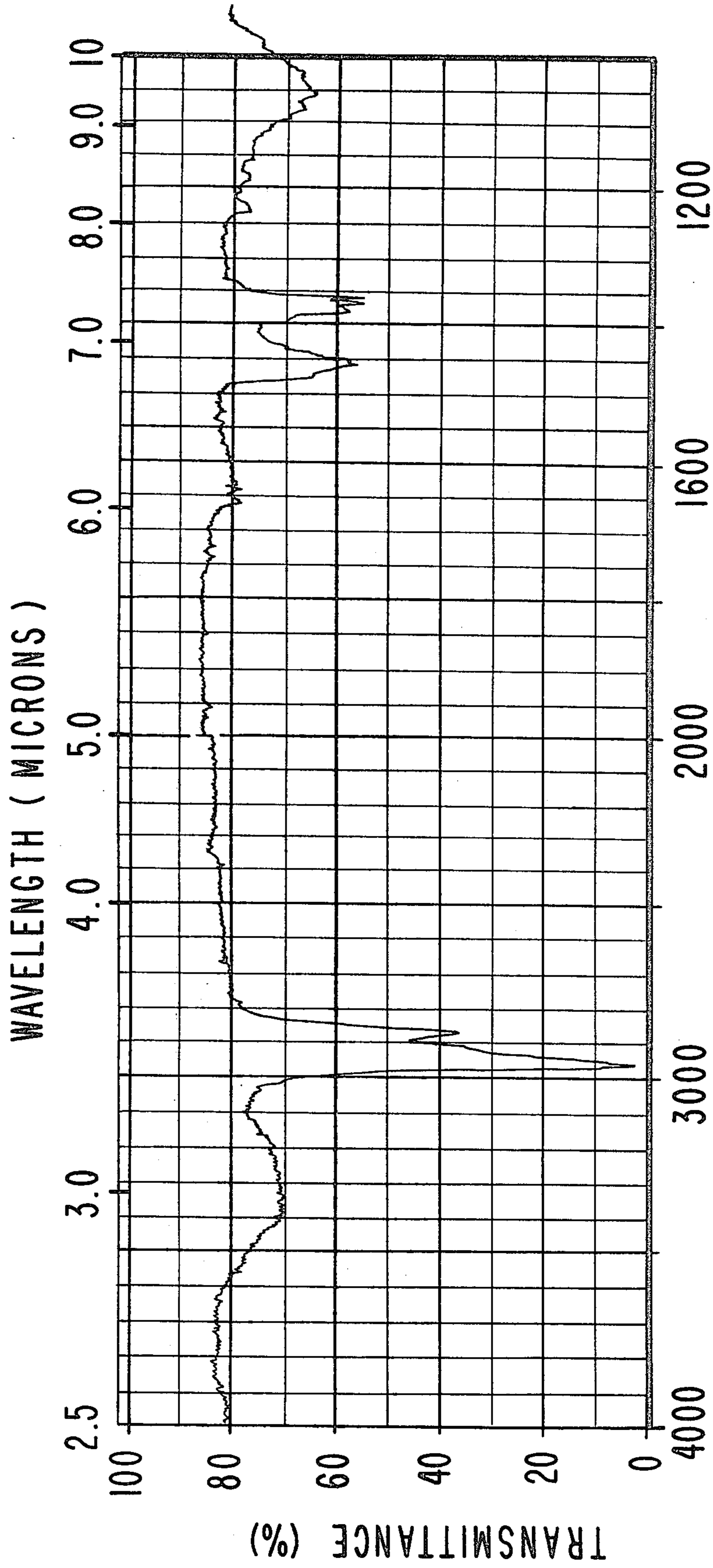
IR SPECTRUM FOR EXAMPLE I, PEAK I, OF GLC OF FIG. 1E.
