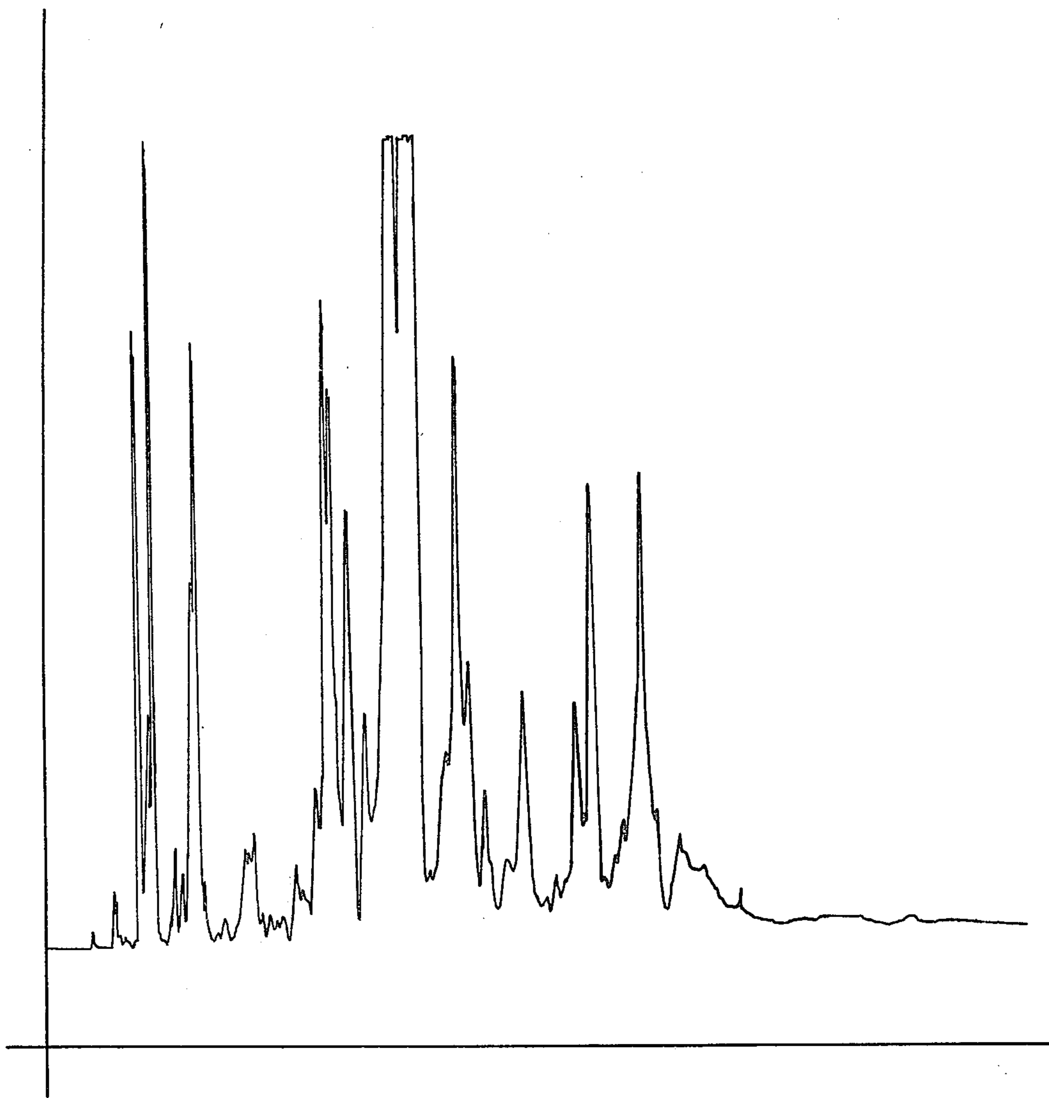
GLC PROFILE FOR EXAMPLE I .
