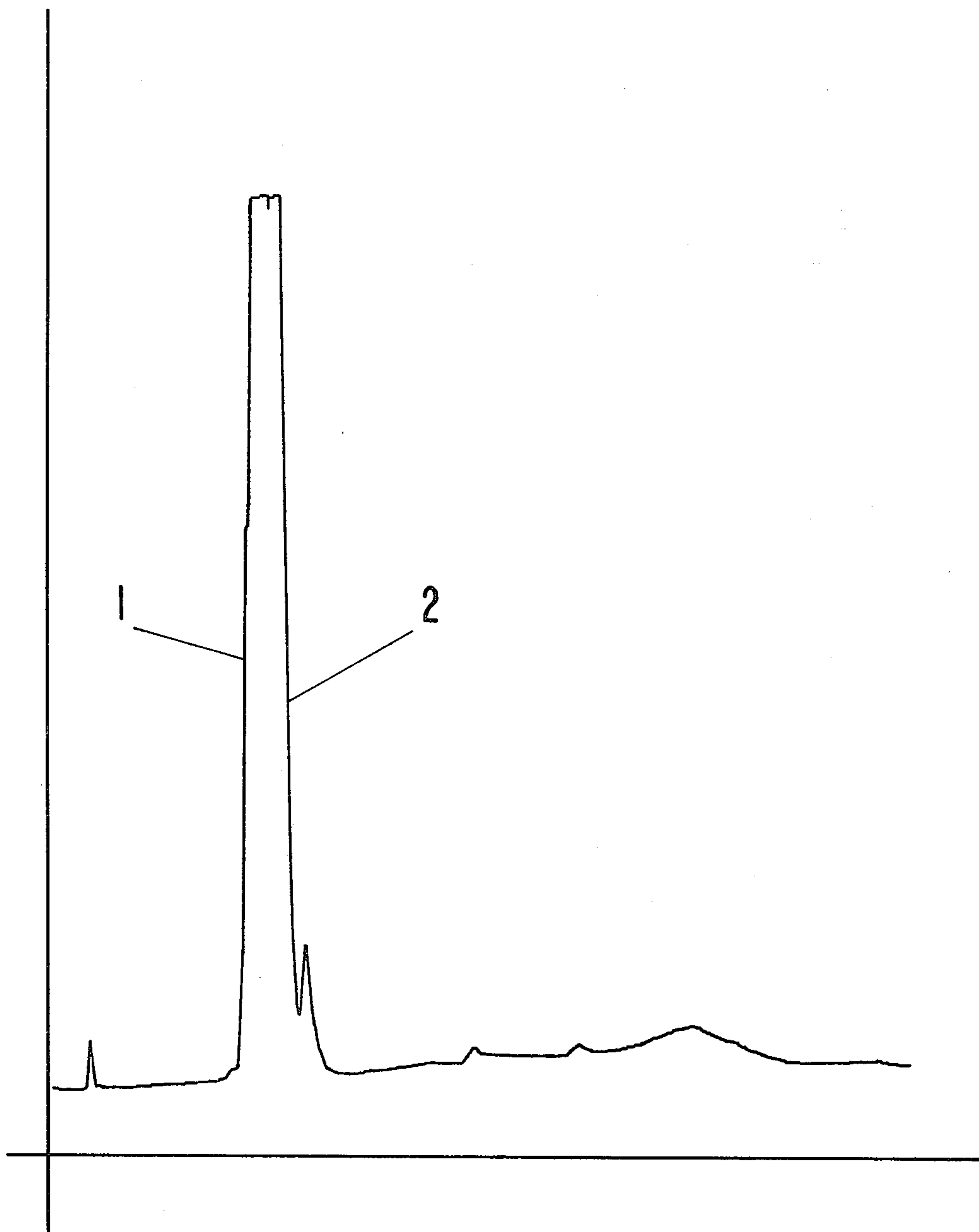
GLC PROFILE FOR EXAMPLE I. DISTILLATION PRODUCT
