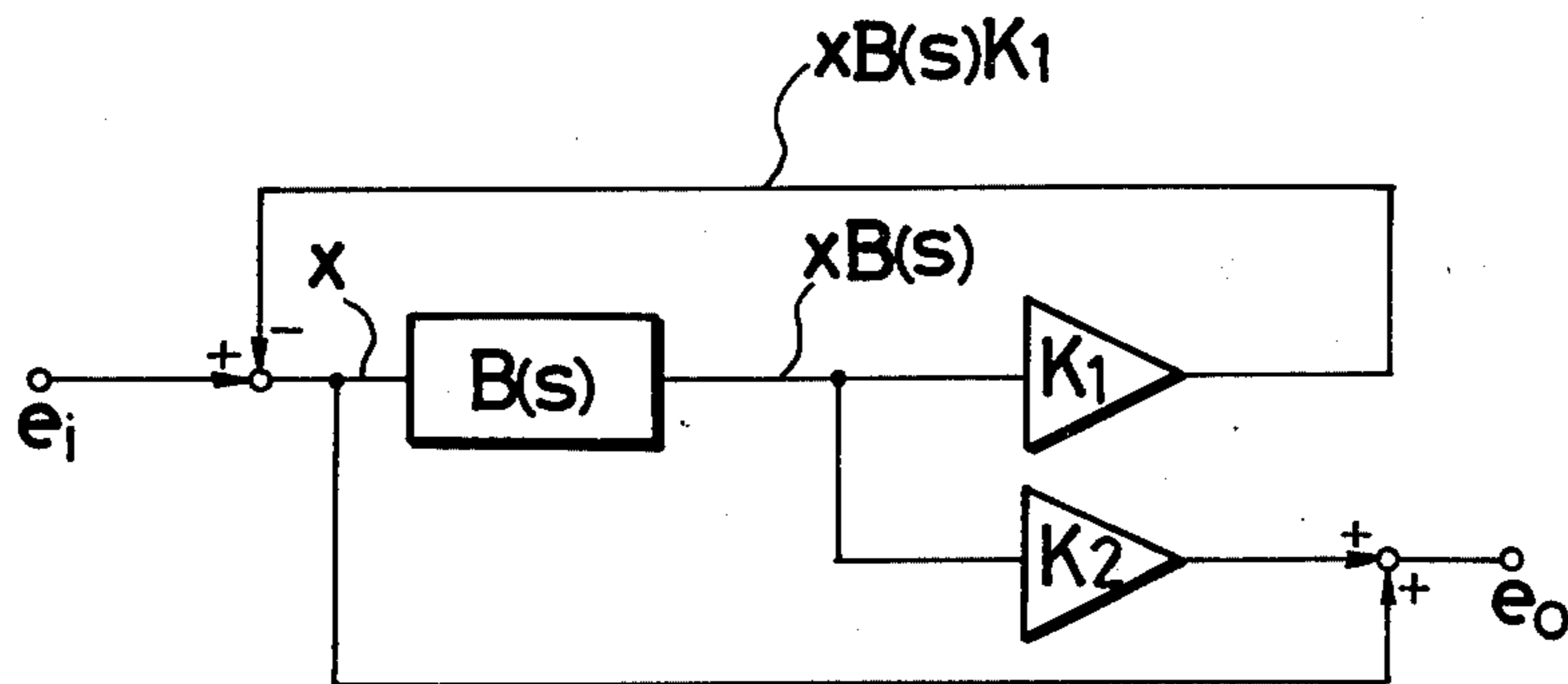
FIG. 2 PRIOR ART
