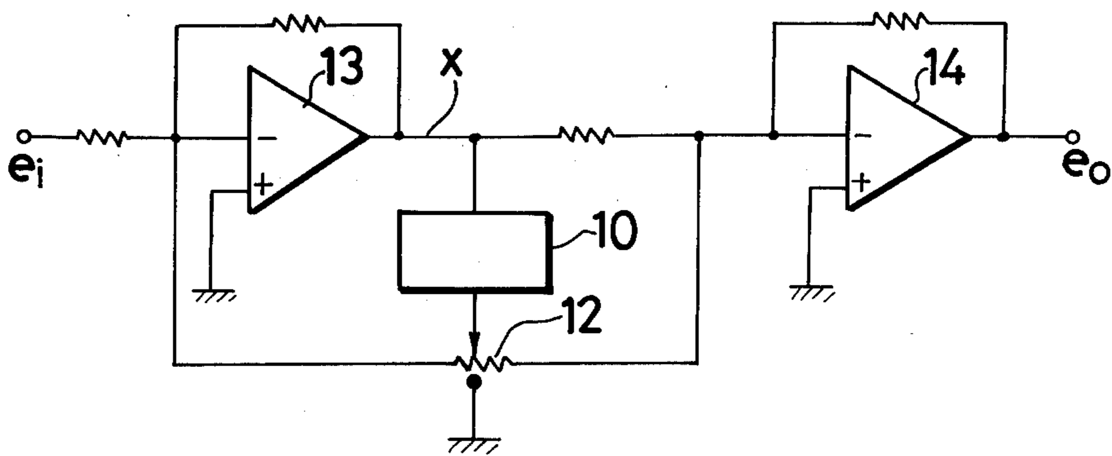
FIG. 2 PRIOR ART
