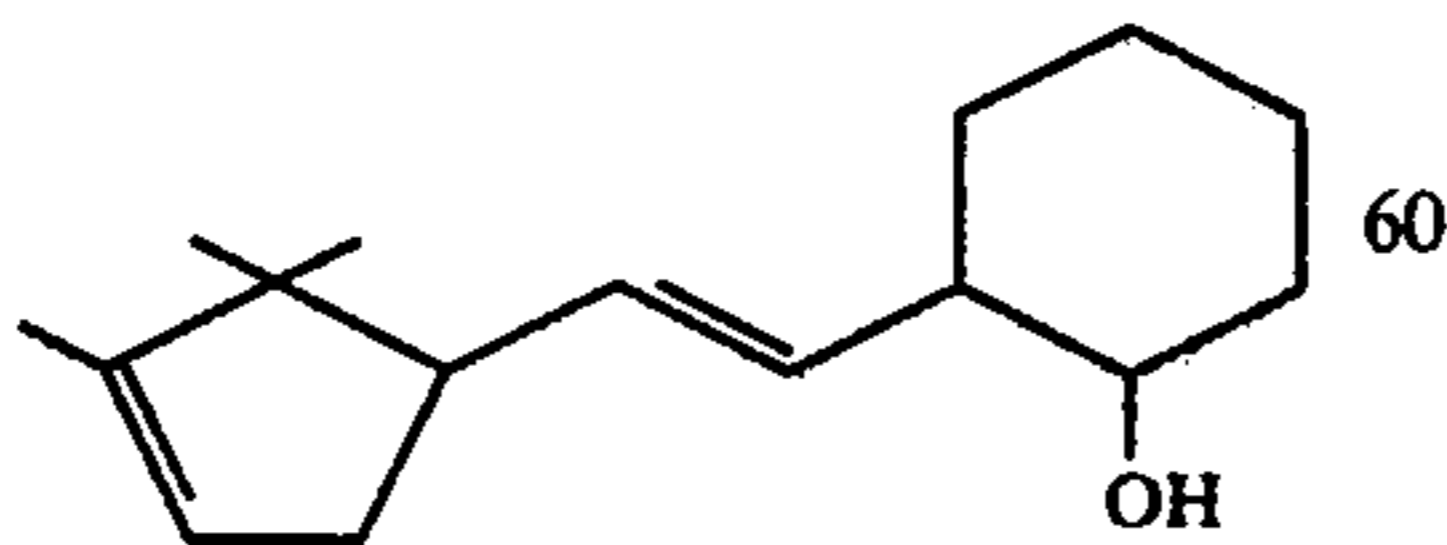
FIG. 5 is the NMR spectrum for fraction 2 resulting from the fractional distillation of the reaction product of Example II containing the compounds having the structures:
