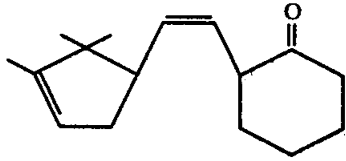
FIG. 3 is the NMR spectrum for fraction 3 resulting from the fractional distillation of the reaction product of Example I having the compounds having the structures:
