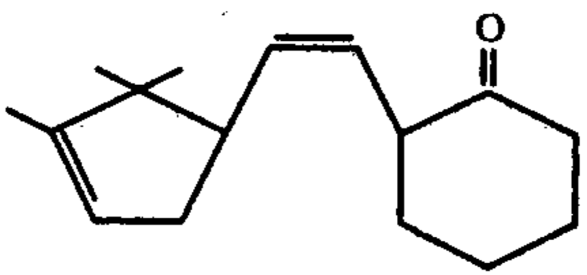
FIG. 4 is the GLC profile for the reaction product of Example II containing the compounds having the structures:
