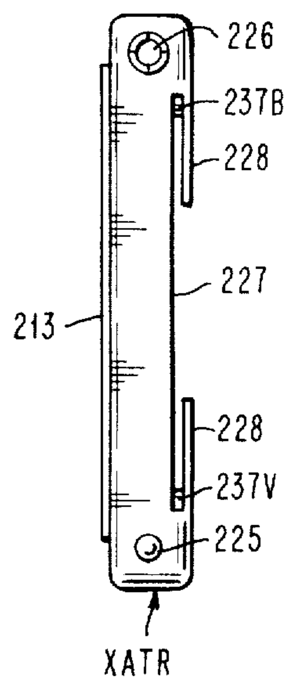
FIG. 2D
