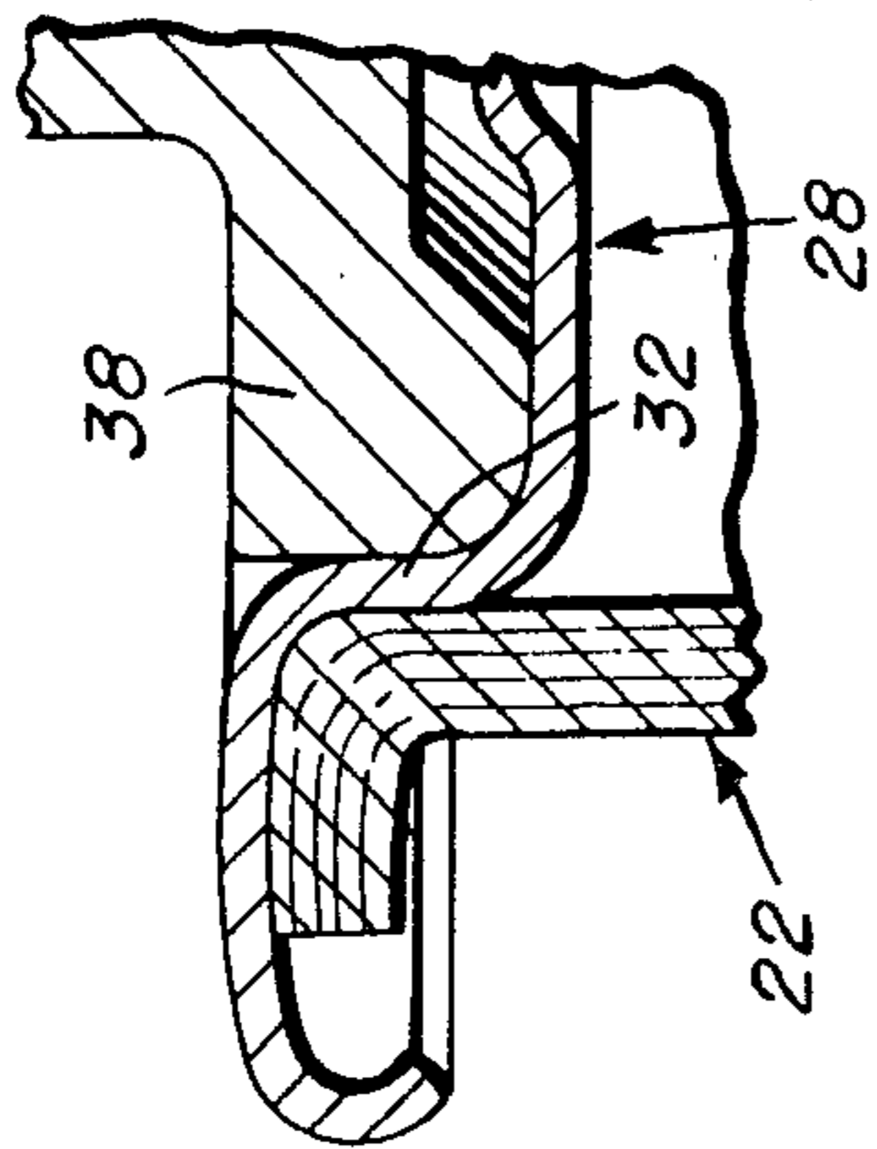
FIG. 11 PRIOR ART
